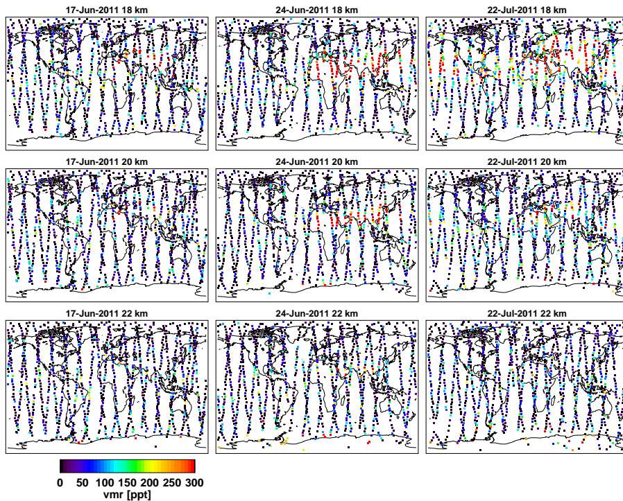
Fig. 9. Example from the MIPAS dataset of SO 2 for three days and at three altitude levels after the eruption of Nabro on 12 June 2011. Note that the color-scale does not cover the entire range of the data such that vmr values > 300 pptv are set to the color at 300 pptv (red) and negative values to zero (black).
