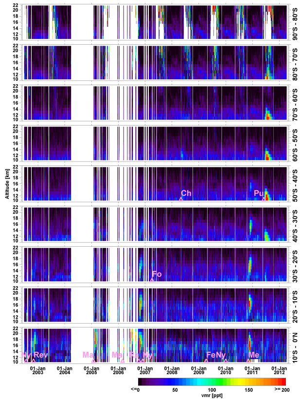
Fig. 11. Time series of color-coded SO 2 volume mixing ratio profiles for 10° latitude bins in the Southern Hemisphere with a time resolution of two days. The color scale is restricted to 0–200 pptv: negative and values larger than 200 pptv are given the color belonging to 0 and 200 pptv, respectively. Volcanic eruptions are indicated at the latitude bin of their location (for details see Table 3).
