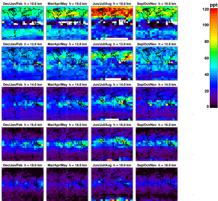
Fig. 16. Seasonal global \text{SO}_2 background distributions at different altitude levels based on all MIPAS observations. The following time periods have been left out to avoid volcanic contributions: October–December 2002, July–August 2003, January–August 2005, May–November 2006, October–November 2007, July 2008–January 2009, April–December 2009, November–December 2010, June–October 2011.
