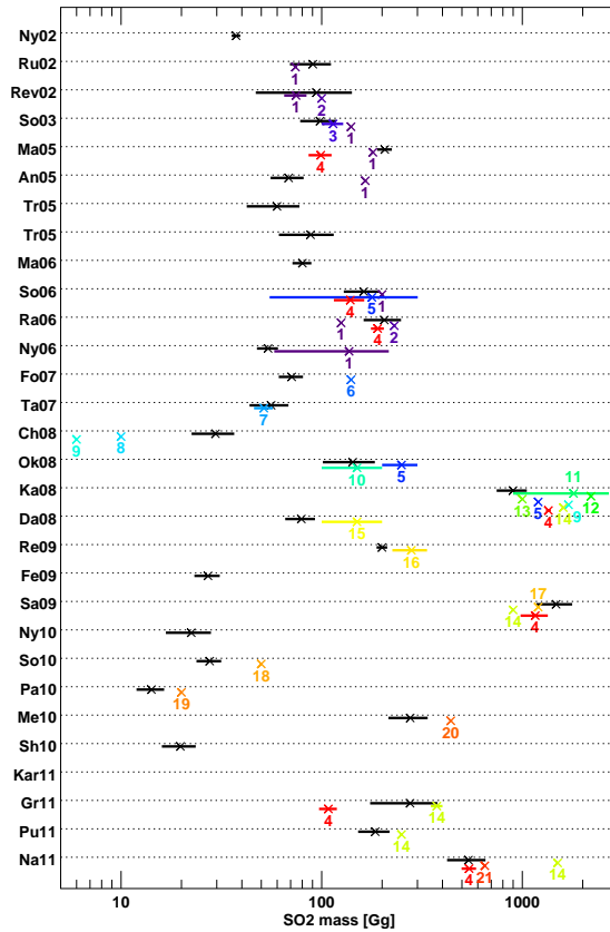
Fig. 15. Graphical representation of total SO 2 eruption masses as listed in Table 3. Black: MIPAS, red: MLS, other colors: nadir instruments. The colored numbers refer to the references given in Table 3.
