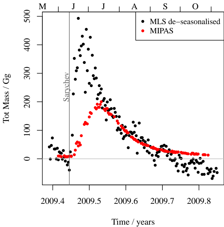
Fig. 13. Comparison between daily values of total mass of \text{SO}_2 above 146.8 hPa from MIPAS (red) and from MLS de-seasonalised observations (black) (Pumphrey et al., 2015).
