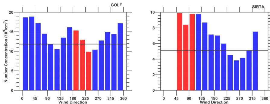
Figure 9. Number concentrations measured at the two satellite sites during summer with respect to wind direction/air mass transport direction measured at the respective site. The angles which indicate that the air mass traveled through the city center prior to reaching the site are depicted in red. The horizontal dashed black line corresponds to the campaign average for each site. Periods with wind speed below 1 \text{ ms}^{-1} were omitted from the analysis.
