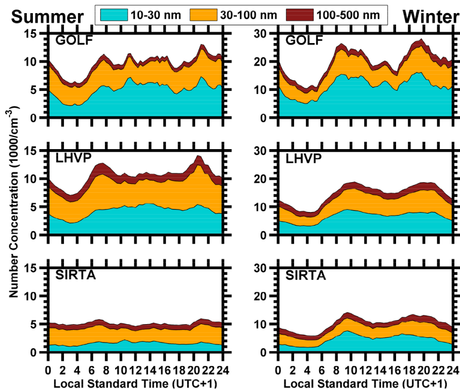
Figure 7. Number concentration diurnal profiles of summer (left) and winter (right) campaigns for size ranges from 10 to 30, 30 to 100, and 100 to 500 nm, respectively. Different scales are used for each season.
