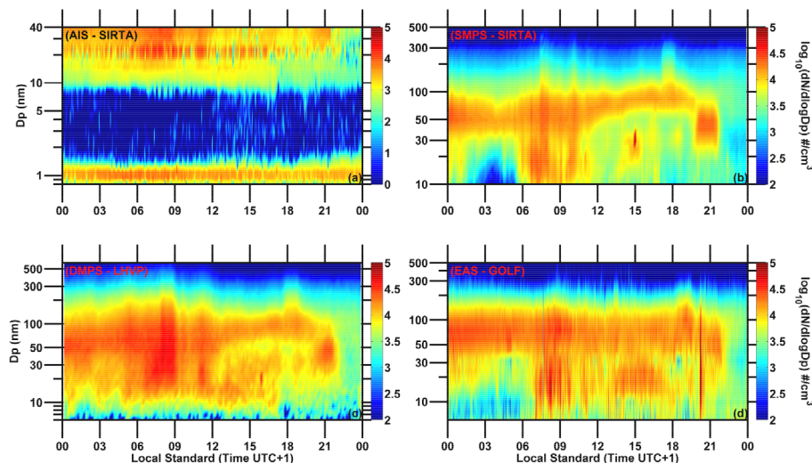
Figure 5. Size distribution measurements during a non-event day (29 July 2009): (a) AIS measurements at SIRTA, (b) SMPS measurements at SIRTA, (c) DMPS measurements at LHVP, (d) EAS measurements at GOLF. Time of day corresponds to local standard time (UTC + 1). D_p is the particle diameter.
