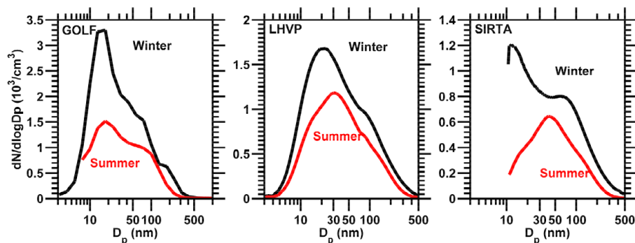
Figure 8. Campaign average particle number size distributions for summer (red) and winter (black) of all ground sites based on measurements of EAS at GOLF, DMPS at LHVP and SMPS at SIRTÀ. Note the different scaling of the y axes.
