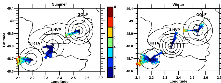
Figure 6. Wind direction rose plots during the summer and winter campaigns at each of the ground sites. Each rose segment corresponds to an angle bin of \pi/18 (i.e. 20^\circ ) and concentric circles at each site correspond to 5% relative frequency. Wind speed, in \text{m s}^{-1} , corresponding to each size bin is color coded inside each rose. Wind speeds below 1 \text{ m s}^{-1} have been omitted from the graph.
