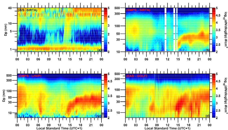
Figure 3. Size distribution measurements during a nucleation event day (12 July 2009) at all ground sites. (a) AIS measurements at SIRTA, (b) SMPS measurements at SIRTA, (c) DMPS measurements at LHVP, (d) EAS measurements at GOLF. Time of day corresponds to local standard time (UTC + 1). D_p is the particle diameter.
