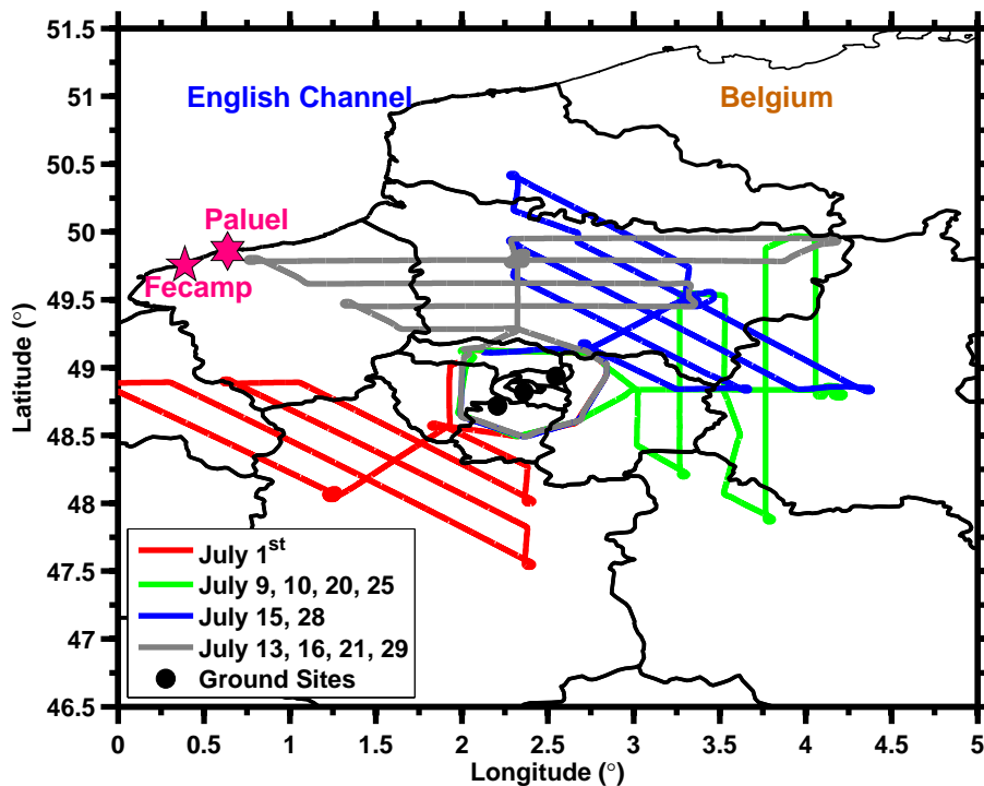
Figure 2. Flight paths of the ATR-42 aircraft during the summer campaign. Different colors correspond to different flight routes. The cities of Fecamp and Paluel are also depicted in the map.
