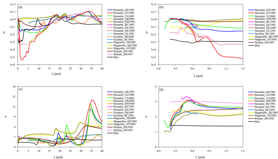
Figure 1. Spectral distribution of the imaginary and real parts of the complex refractive index for different iron oxides from Table 1 at wavelengths of 0 to 40 \mu\text{m} ( a , c ) and expanded for wavelengths of 0 to 1.5 \mu\text{m} ( b , d ).
