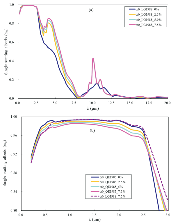
Figure 4. Spectral single scattering albedo (SSA) for mixtures of illite and hematite with varying percentages and refractive indices at wavelengths of 0–20 \mu\text{m} (a) and 0–3 \mu\text{m} (b).
