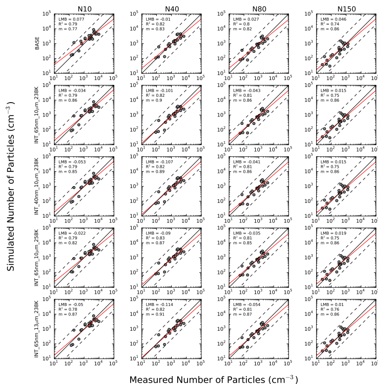
Figure 3. Annual-mean N10, N40, N80 and N150 GEOS-Chem-TOMAS simulation-to-measurement comparisons for the 5 simulations at the 21 SMPS measurement sites.
