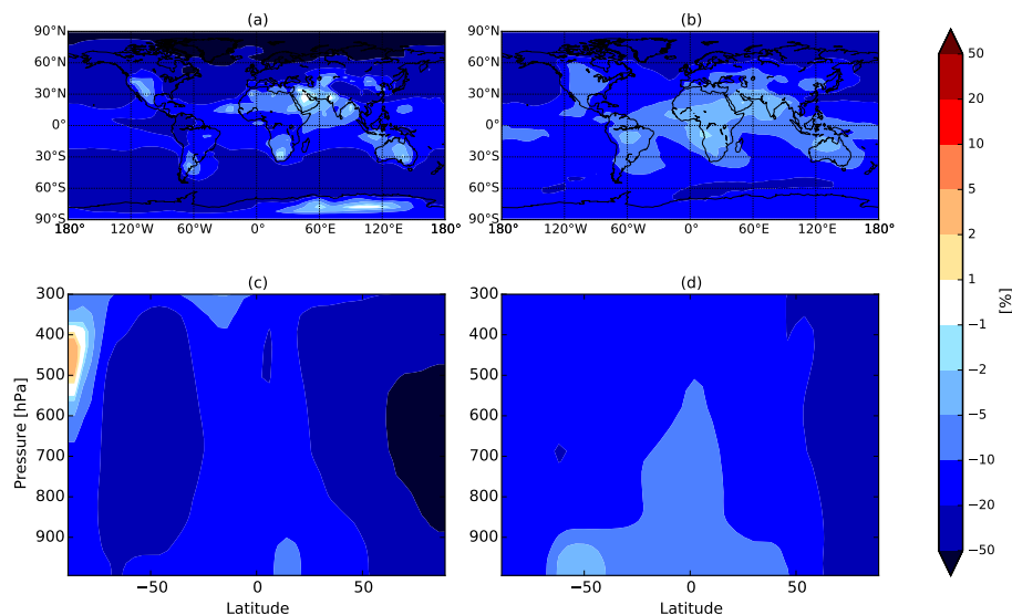
Figure 1. Annual-mean percent changes in N10 ( a and c ) and N80 ( b and d ) changes between INT_65nm_10 \mu m_238K and BASE. ( a ) and ( b ) show the changes for the 2 km model layer, and ( c ) and ( d ) show the zonal-mean changes throughout the troposphere.
