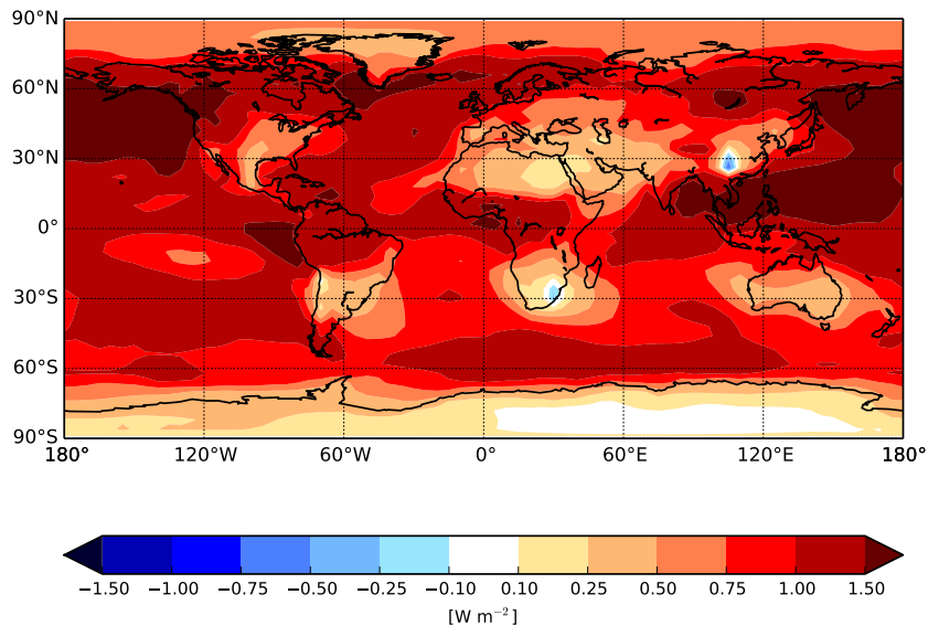
Figure 2. Annual-mean AIE between the INT_65nm_10µm_238K and the BASE simulation.
