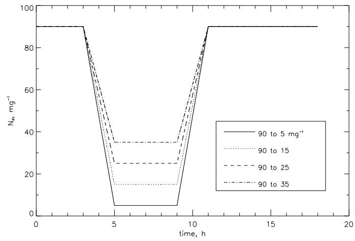
Figure 1. Time series of imposed time series of drop concentration N . The minimum N is varied between 5 \text{mg}^{-1} and 35 \text{mg}^{-1} .
