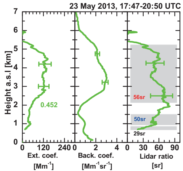
Fig. 10. Mean vertical profiles of the 532 nm particle extinction coefficient, backscatter coefficient, and lidar ratio for the observational period from 17:47–20:50 UTC on 23 May 2013. The Raman lidar method is applied. Vertical signal smoothing lengths of 600 m (below 1.1 km height), 1500 m (1.1–2.8 km height), and 2100 m (above 2.8 km height) are applied before computing the extinction coefficients and lidar ratios. The signal smoothing length is 750 m for the shown backscatter coefficient profile. Total AOT (given as number in the left panel) and layer mean values of the lidar ratio for the 0.7–0.85 km height layer (influenced by marine and local haze particles), the 0.86–1.5 km layer (influenced by European haze) and for the pure dust layer (2.1–5.2 km height range) are given as numbers. Error bars provide the uncertainty (standard deviation) by signal noise.
