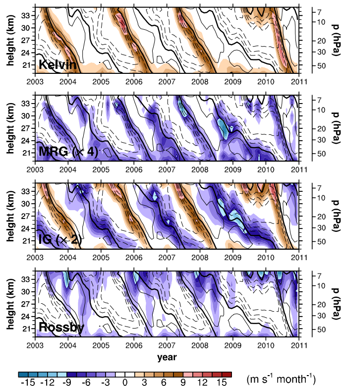
Figure 1. Time–height cross-sections of the zonal momentum forcing by the Kelvin, MRG, IG, and Rossby waves (from top to bottom) averaged over 5^{\circ}\text{N} – 5^{\circ}\text{S} , obtained using the model-level data of ERA-I over the period 2003–2010 (shading). The MRG and IG wave forcing is multiplied by 4 and 2, respectively. The zonal mean wind over 5^{\circ}\text{N} – 5^{\circ}\text{S} is superimposed at intervals of 10\text{ m s}^{-1} (contour). The thin solid, dashed, and thick solid lines indicate westerly, easterly, and zero wind, respectively.
