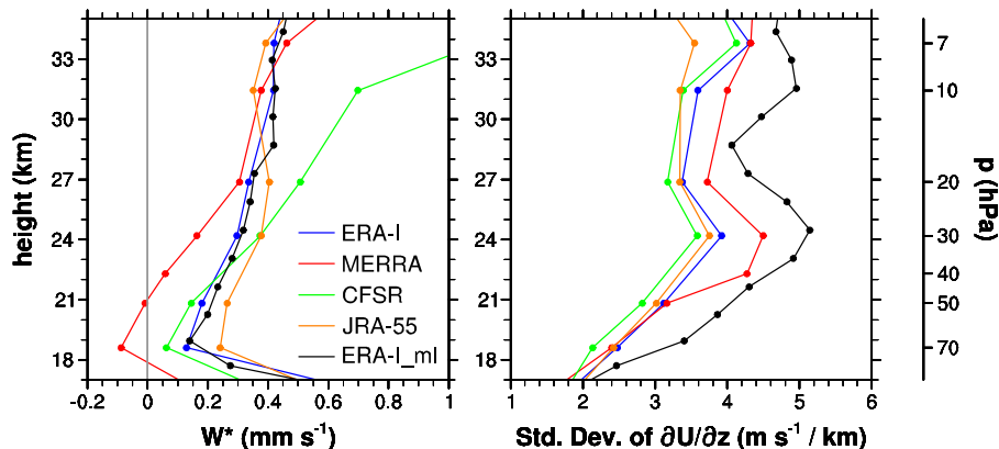
Figure 5. (a) Mean residual vertical velocity and (b) SD of the monthly and zonal mean wind shear for the period 1979–2010 averaged over 5^\circ\text{N} – 5^\circ\text{S} , obtained using the p level data of ERA-I (blue), MERRA (red), CFSR (green), and JRA-55 (orange) as well as the model-level data of ERA-I (black).
