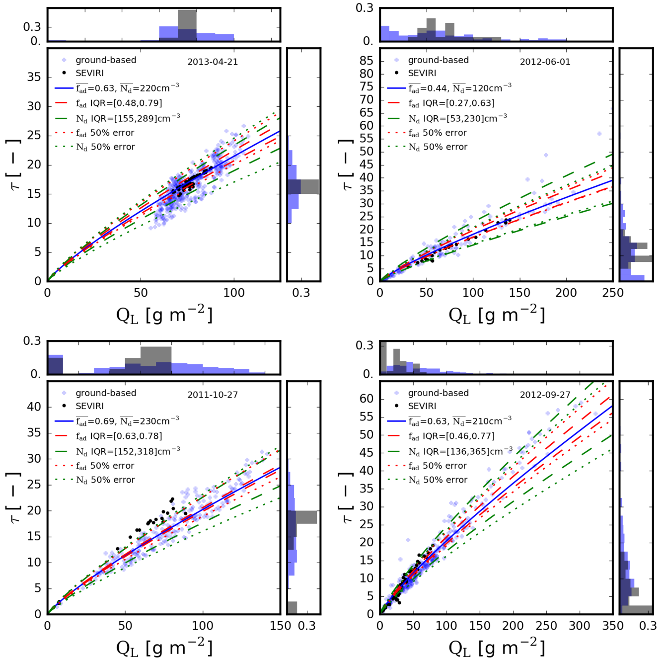
Figure 5. Relationship between Q_L and \tau for the four case days (Table 2). Blue crosses represent the LACROS observations for the case day, black dots the SEVIRI observations. The solid blue line represents the relationship between \tau and Q_L for the median f_{ad} and N_d of the LACROS observations. Uncertainty estimates of \tau as a function of Q_L is given in terms of temporal variability using the IQR of the time-series (dashed), and as 50% relative uncertainty in N_d and f_{ad} (dotted). Furthermore the histograms of ground-based and SEVIRI observations are shown on each axis in the same colors as stated before.
