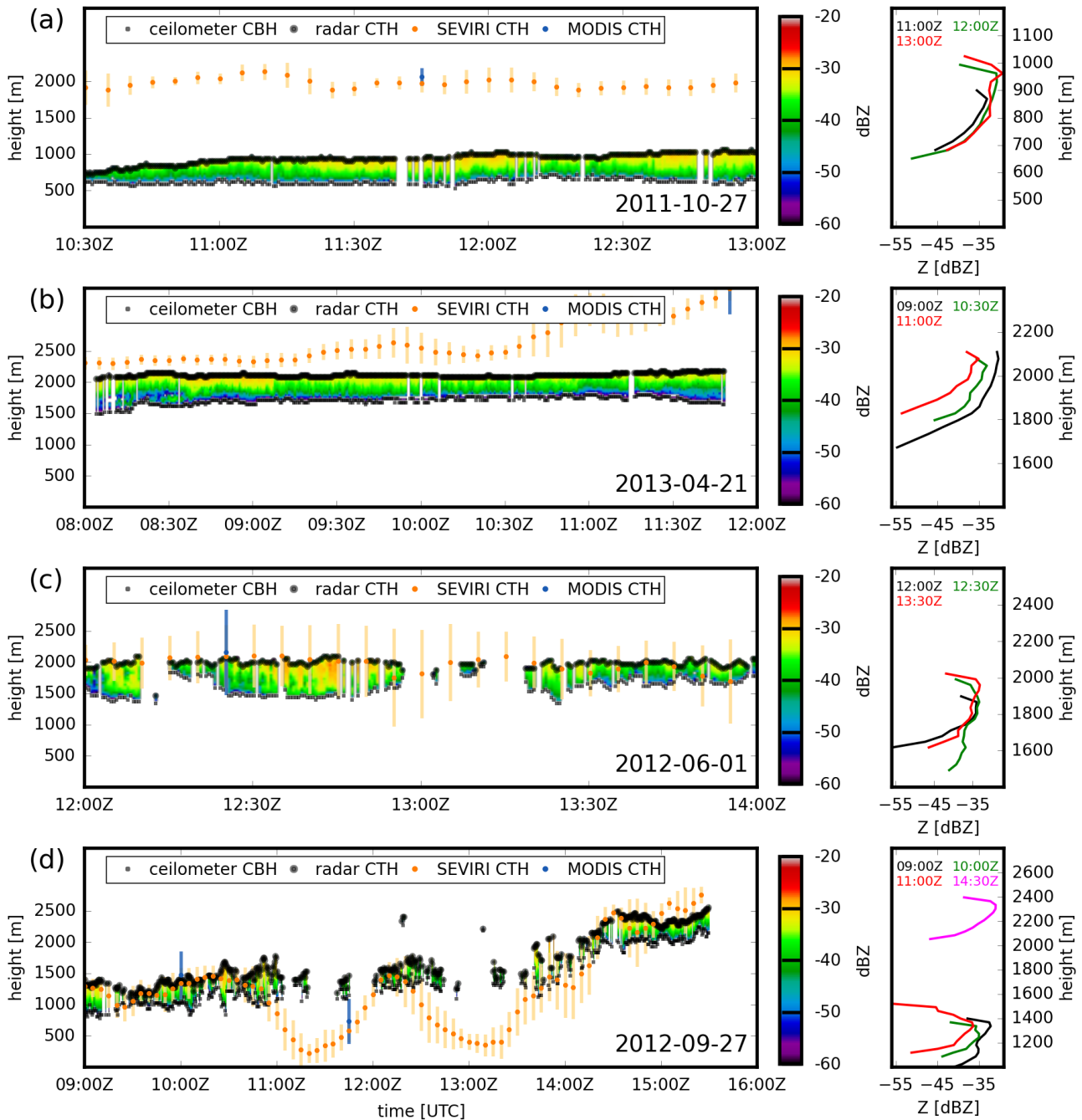
Figure 1. Time series of radar reflectivity Z(z) (in dBZ) and cloud boundaries for the 4 cases listed in Table 2; (a) 27 October 2011, (b) 21 April 2013, (c) 1 June 2012, (d) 27 September 2012. Cloud borders are shown as detected by Cloudnet with black dots and by SEVIRI using NWCSAF in orange dots, and MODIS in blue dots. Sample profiles of Z(z) are shown at different times during each case.
