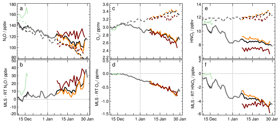
Figure 13. Vortex-averaged (left to right) \text{N}_2\text{O} , \text{O}_3 , and \text{HNO}_3 from MLS (solid lines) and RT passive subtraction (dashed lines) calculations (see text) at 490 K from 8 December 2012 through January 2013. (a) , (c) , and (e) show mixing ratios in each of the vortices present; (b) , (d) , and (f) show the difference between MLS and RT (passively transported) values, indicative of transport uncertainties for \text{N}_2\text{O} , and chemical and/or microphysical changes for \text{O}_3 and \text{HNO}_3 . Line colors are as in Fig. 11.
