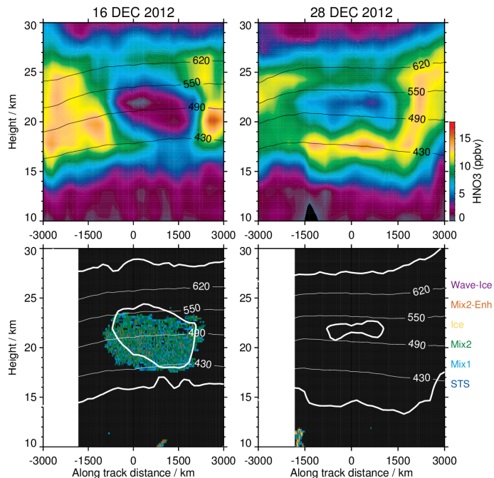
Figure 10. MLS HNO 3 (ppbv) along an orbit track (top panels) and collocated CALIPSO PSC classification (bottom panels, see text), on 16 and 28 December 2012. Overlaid labeled lines are potential temperature contours. Overlaid thick white contour in the bottom panels is the 5 ppbv HNO 3 contour.
