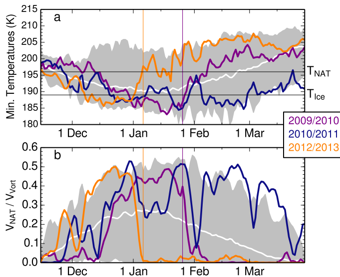
Figure 2. Time series of (a) minimum temperatures poleward of 40^{\circ}\text{N} at 490 K and (b) V_{\text{NAT}}/V_{\text{Vort}} (see text) from MERRA reanalysis. Individual lines show 2009/10 (purple), 2010/11 (blue) and 2012/13 (orange). Envelope shows the remaining years from 1979/80 through 2013/14. Thin vertical lines indicate the dates when the major SSW criteria were met in 2010 (purple) and 2013 (orange). Thin black horizontal lines in (a) indicate the NAT and ice PSC thresholds.
