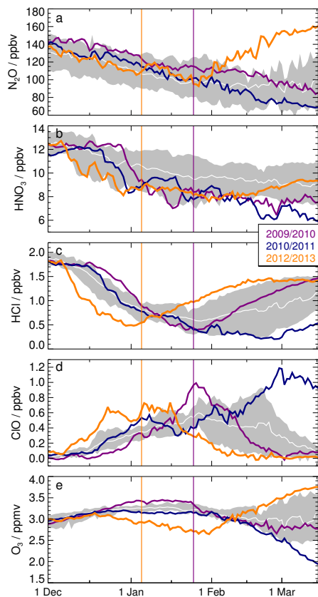
Figure 12. Vortex averaged MLS trace gases at 490 K, in 2012/13 (orange), 2010/11 (blue), and 2009/10 (purple) compared with the range (grey shading) and average (white line) for the other years in 2004/05 through 2013/14. (a) \text{N}_2\text{O} , (b) \text{HNO}_3 , (c) \text{HCl} , (d) \text{ClO} , and (e) \text{O}_3 . Vertical purple and orange lines show the onset dates of the SSWs in 2010 and 2013, respectively.
