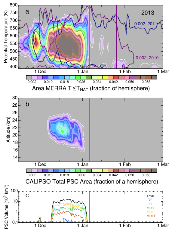
Figure 3. (a) Time series of the area poleward of 30° N with T \leq T_{NAT} as a function of potential temperature in 2012/13 from MERRA (color fill; the white contour shows a value of 0.001, indicating a very small non-zero value); area is expressed as fraction of a hemisphere. The overlaid purple and blue contours show the 0.002 contour (which is at the boundary between grey and lavender in 2012/13) in 2009/10 and 2010/11, respectively; purple and orange vertical lines show the beginning dates of the SSWs in 2010 and 2013, respectively. (b) Time series of CALIPSO total PSC area; format is as in (a), but with only 2012/13 values. (c) Time series of the total volume of different types of PSCs observed by CALIPSO in 2012/13 (see text).
