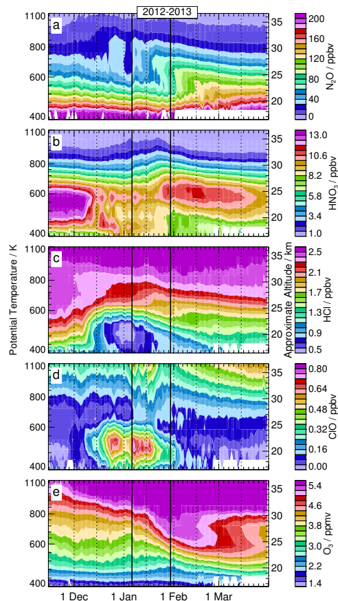
Figure 9. Potential temperature/time series of vortex averaged (within the 1.4 \times 10^{-4} \text{ s}^{-1} sPV contour) (a) \text{N}_2\text{O} , (b) \text{HNO}_3 , (c) \text{HCl} , (d) \text{ClO} , and (e) \text{O}_3 derived from MLS data. The thin solid black vertical lines indicate the onset day of the SSW (6 January, \sim 2 days before the vortex split) and the day when the offspring vortices reunited (30 January).
