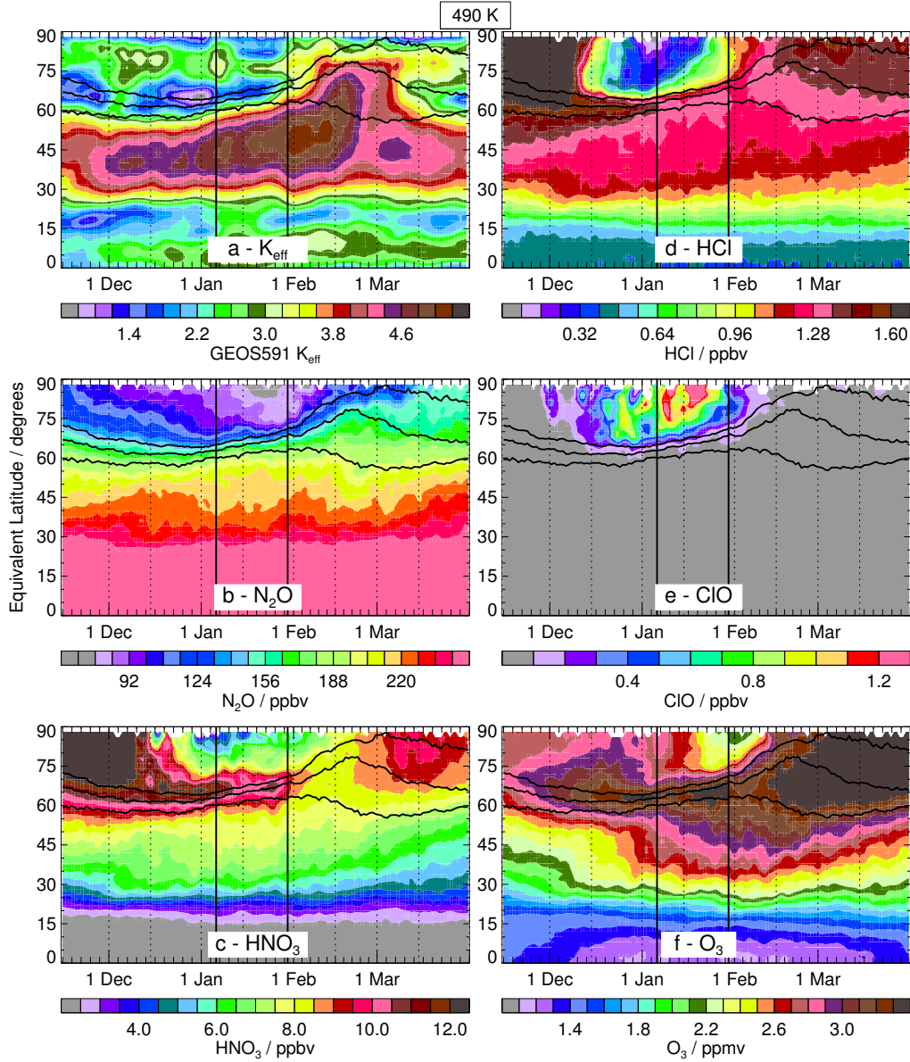
Figure 8. Equivalent latitude/time series at 490 K of (a) effective diffusivity from GEOS591 (color bar range -0.6 to 5.4 , expressed as log-normalized equivalent length; low values indicate transport barriers and high values regions of enhanced mixing) and MLS (b) \text{N}_2\text{O} (color bar range 60 to 252 ppbv), (c) \text{HNO}_3 (color bar range 2.0 to 12.5 ppbv), (d) HCl (color bar range 0 to 1.68 ppbv), (e) ClO (color bar range 0 to 1.3 ppbv), and (f) \text{O}_3 (color bar range 1.0 to 3.4 ppmv). Black contours show sPV values of 1.2 , 1.4 , and 1.6 \times 10^{-4} \text{ s}^{-1} , in the vortex edge region. The thin solid black vertical lines indicate the onset day of the SSW (6 January, \sim 2 days before the vortex split) and the day when the offspring vortices reunited (30 January)
