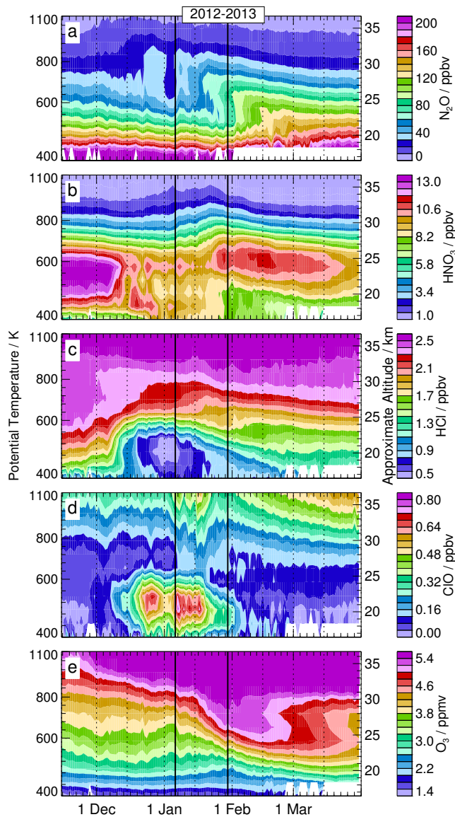
Figure 9. Potential temperature/time series of vortex averaged (within the 1.4 \times 10^{-4} \text{ s}^{-1} sPV contour) (a) N 2 O (color bar range 0 to 210 ppbv), (b) HNO 3 (color bar range 1.0 to 13.6 ppbv), (c) HCl (color bar range 0.5 to 2.6 ppbv), (d) ClO (color bar range 0 to 0.84 ppbv), and (e) O 3 (color bar range 1.4 to 5.6 ppmv) derived from MLS data. The thin solid black vertical lines indicate the onset day of the SSW (6 January, \sim 2 days before the vortex split) and the day when the offspring vortices reunited (30 January).
