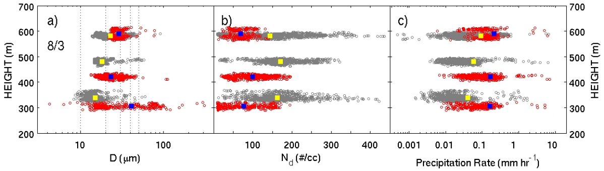
Figure 6. Changes in cloud droplets' (a) size, (b) number concentration, and (c) drizzle rate during cloud-base, mid-cloud and cloud top legs on 3 August 2011. Data obtained from pre-seeding legs (1-second values) are shown as grey (mean value as yellow square); data obtained from post-seeding flights are shown as red (mean value as blue square). (b) and (c) are calculated from drop size distribution (DSD) obtained from CAS and CIP probes, respectively. (a) is calculated from DSDs obtained by combining the CAS and CIP probes.
