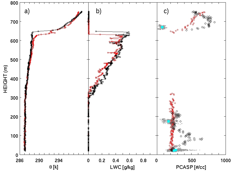
Figure 3. Profiles of (a) potential temperature ( \theta , K), (b) liquid water contents (LWC, \text{g kg}^{-1} ), and (c) accumulation mode aerosol concentrations ( \text{\#}/\text{cc} , PCASP) during the aircraft ascent (black) and descent (red) between 16:52:15-17:10:48 UTC (hh:mm:ss). Aerosol concentrations obtained from sub-cloud layer and above cloud layer are shown as grey colors (mean value is shown as cyan square). The heights and spatial locations of data used are shown in Fig. 4. PCASP resolves particles in diameter ranges from 0.1-3 \mu\text{m} .
