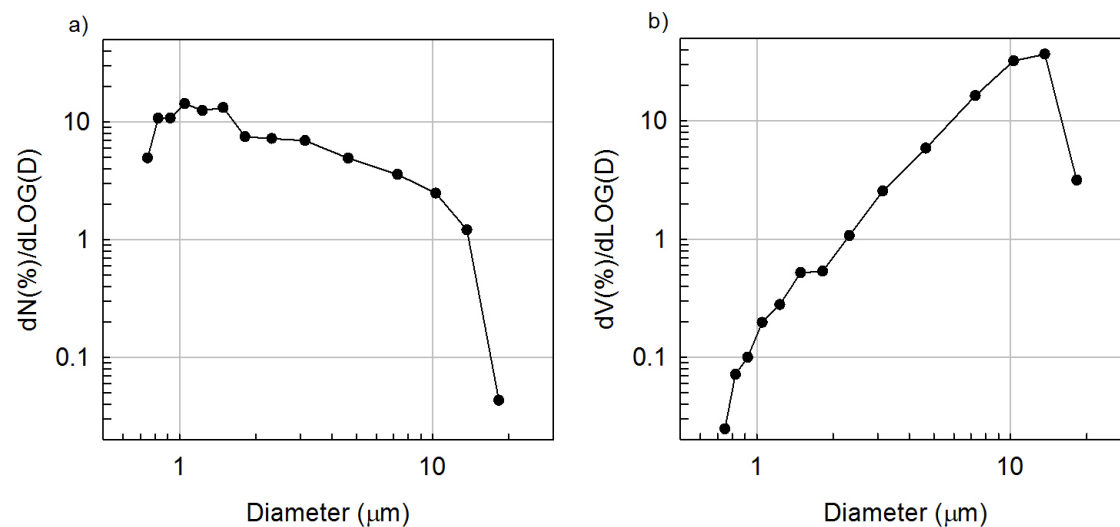
Figure 1. Relative (percent of total) (a) number and (b) volume distributions of powdered salt delivered to CAS sampling volume from atomizer.
