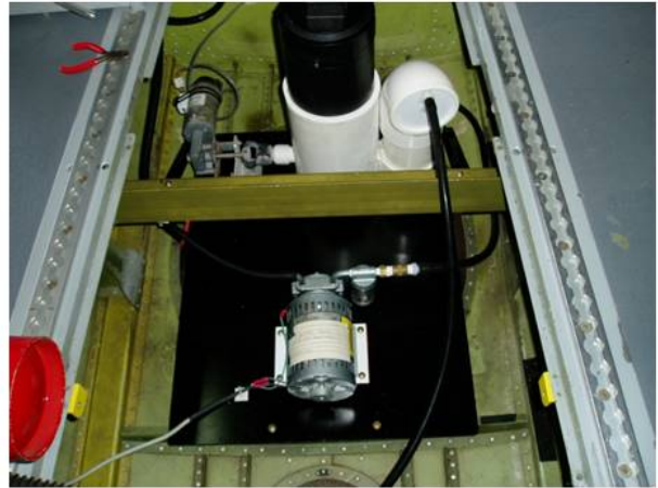
Figure 2. A pictorial schematic and photo of the salt powder delivery system.
