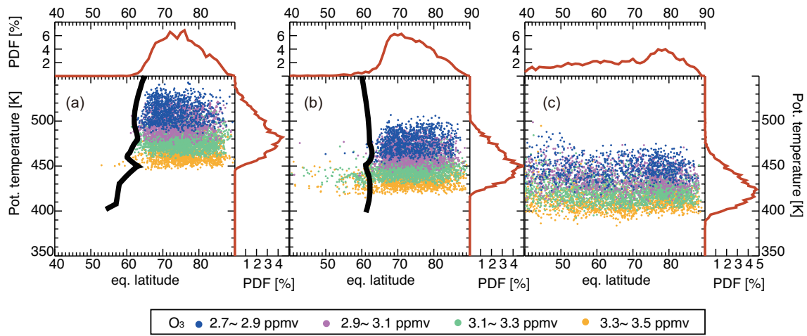
Figure 10. Spatial distribution in the eq. latitude- \theta space of the APs defined by the mixing ratios of \text{N}_2\text{O} and \text{pO}_3 inside the square in Fig. 9(a3), i.e. with \text{N}_2\text{O} and \text{pO}_3 values from 80 to 130 ppbv and from 2.7 to 3.5 ppmv, respectively, calculated from CLaMS run without mixing. (a) Dec. 23, 2008; (b) Jan. 23, 2009; (c) Feb. 23, 2009. Colors indicate different ranges of \text{pO}_3 values and are defined in the box. The PDFs along the eq. latitude and potential temperature axes are shown as red lines. Thick black lines denote the edge of the polar vortex.
