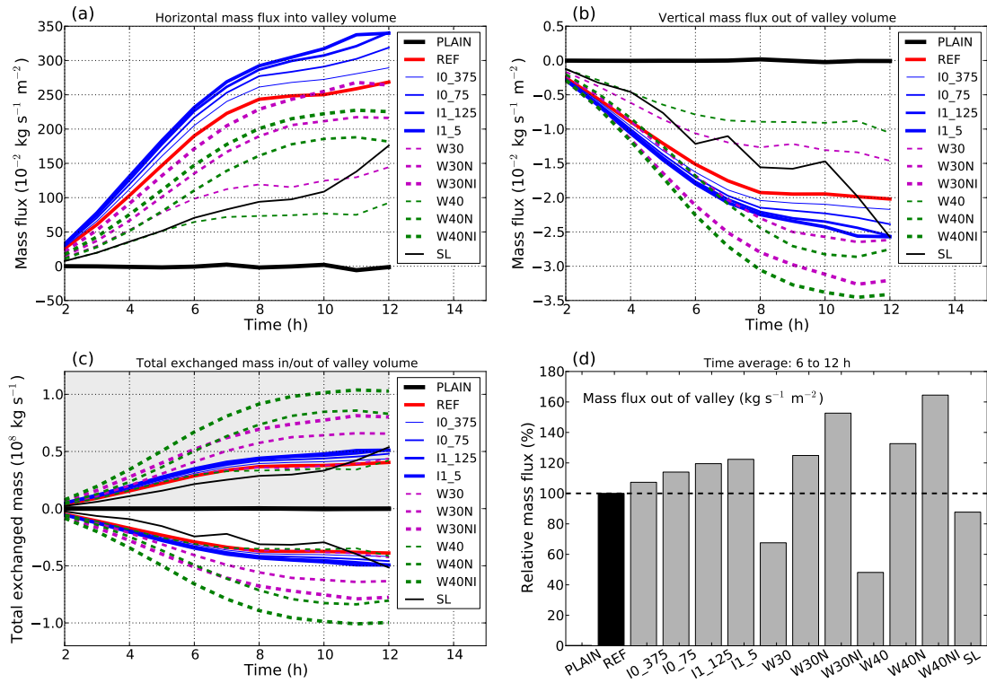
Figure 9. Mean mass flux budget of the whole valley volume, which is limited by the vertical cross section at the valley entrance ( y = 0 km, 0 \leq z \leq 1.5 km) and the horizontal area at crest height ( 0 \leq y \leq 100 km, see Fig. 1). Negative values imply mass fluxes out of the volume. a) Time series of horizontal mass flux ( \text{kg s}^{-1} \text{m}^{-2} ) into and b) vertical mass flux ( \text{kg s}^{-1} \text{m}^{-2} ) out of the valley volume. c) Total exchanged mass (i.e. \text{kg s}^{-1} ) into (grey shaded area) and out (white shaded area) of the valley volume. d) Relative mass fluxes out of the valley averaged between 6 and 12 hours of simulation and scaled with the corresponding value of the REF case (black bar). The horizontal dashed line in d) marks mass flux ratios of 100%.
