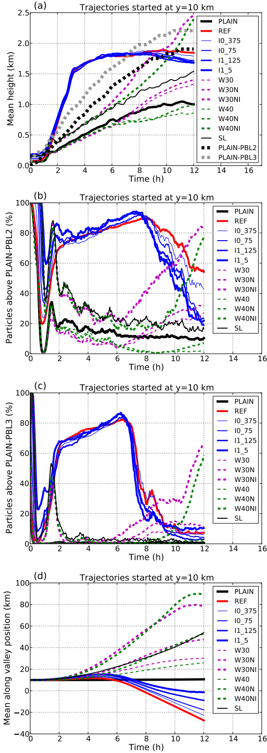
Figure 13. Time series of a) mean trajectory height, b) fraction of parcels, which are located above PLAIN-PBL2 and c) above PLAIN-PBL3 and d) mean along-valley position of parcels started at y = 10 km. The thick black and grey dashed lines in a) mark the PLAIN-PBL2 and PLAIN-PBL3 height, respectively.
