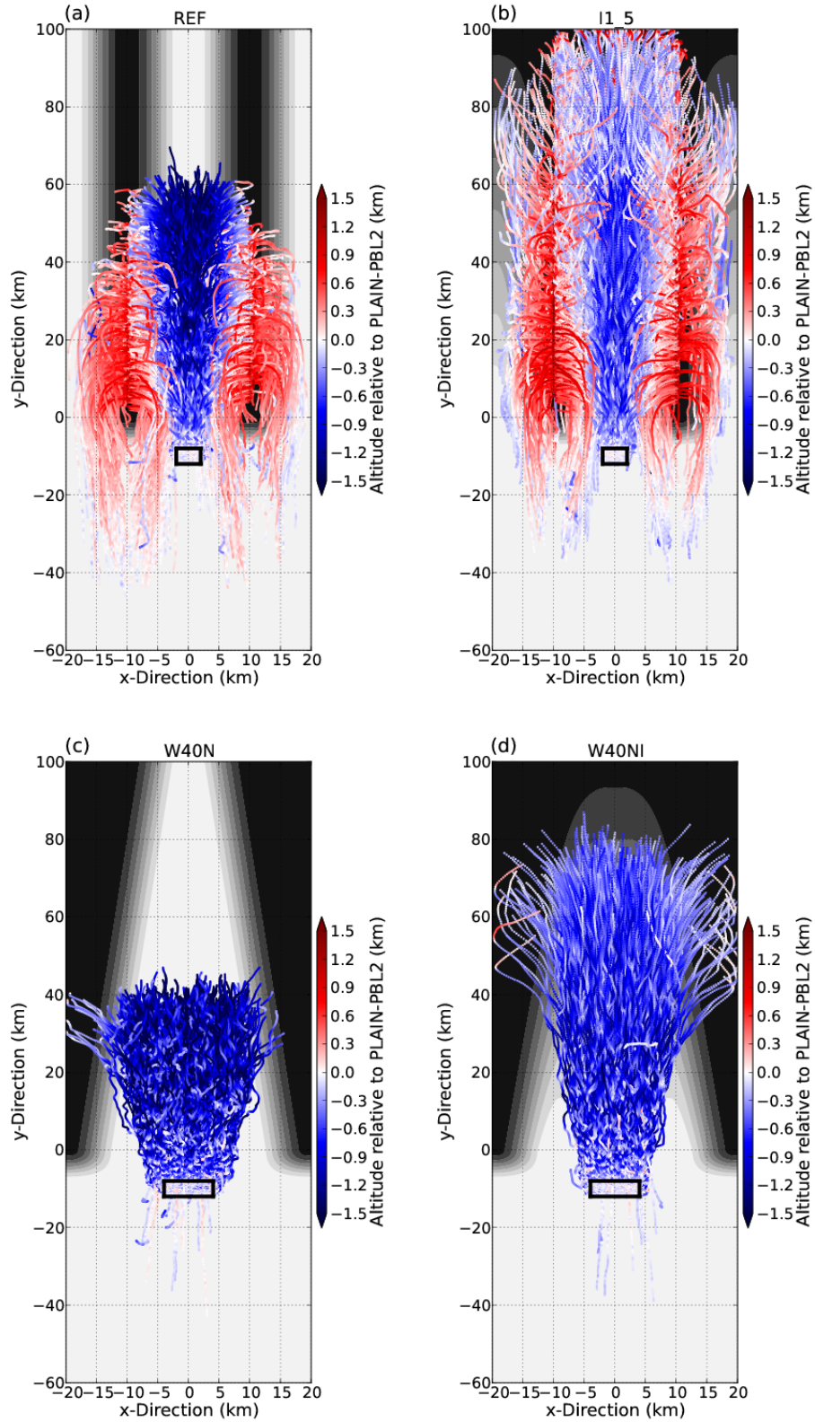
Figure 10. Trajectories started at the initial time of the simulations in a box centred at x = 0 km and y = -10 km and computed for 12 hours for a) REF, b) I1_5, c) W40N and d) W40NI cases. Trajectories are started at vertical levels of 25, 50, 75 and 100 m AGL in the region shown by the black box. The colour shading indicates the time-dependent height of the trajectories. The time-dependent boundary layer height PLAIN-PBL2 (see Fig. 2) is used as reference height: blue colours denote parcels, which are located below this reference height, whereas red colours indicate parcels above PLAIN-PBL2.
