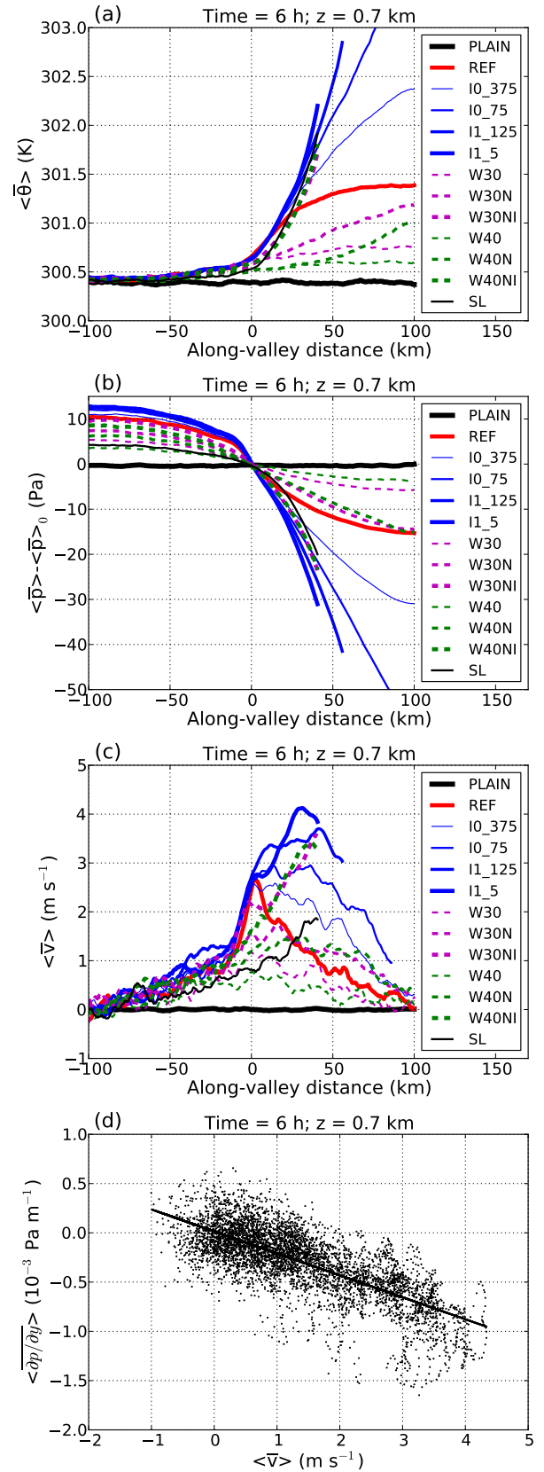
Figure 7. Along-valley structures at 0.7 km altitude in the valley centre ( x=0 km) after 6 hours of simulation of a) potential temperature, b) pressure deviation from pressure at the valley entrance ( y=0 km) and c) along-valley wind speed. Running average smoothing with an interval of 5 km is applied to all curves. The correlation of along-valley wind speed and along-valley pressure gradient is plotted for points in the valley ( x=0 km, y>0 km) for all simulations in d). The black line marks a linear fit of all points.
