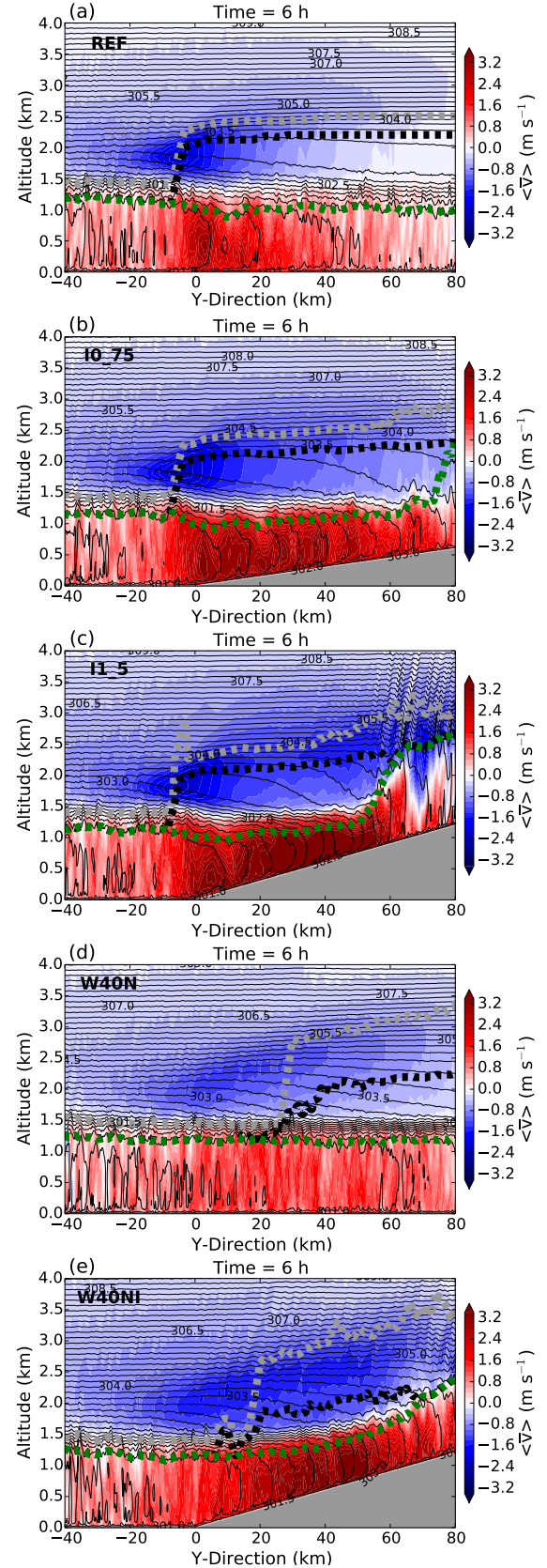
Figure 5. Temporally averaged along-valley flow (colour shading) and potential temperature (contour lines, interval: 0.25 K) after 6 hours of simulation at x = 0 km for different valley depths and widths. Boundary layer heights PBL1, PBL2 and PBL3 are plotted with thick dashed green, black and grey lines, respectively.
