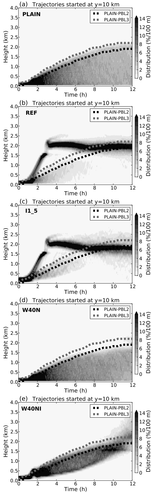
Figure 11. Evolution of parcel height distribution for trajectories started at y = 10 km for a) PLAIN, b) REF, c) I1_5, d) W40N and e) W40NI simulation. The thick black and grey dashed lines mark the PLAIN-PBL2 and PLAIN-PBL3 height, respectively. Distribution values are calculated by splitting the vertical height column into bins of 100 m and determining the percentage of parcels within these height intervals (%/100 m).
