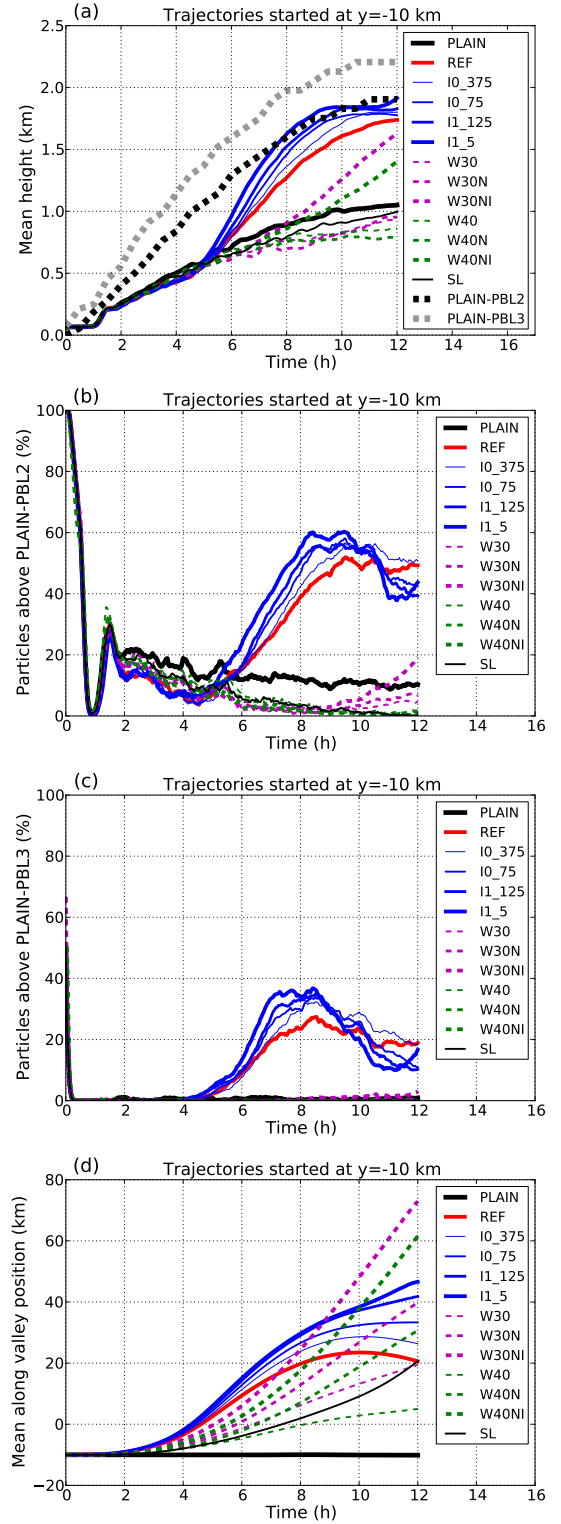
Figure 14. Time series of a) mean trajectory height, b) fraction of parcels, which are located above PLAIN-PBL2 and c) above PLAIN-PBL3 and d) mean along-valley position of parcels started at y = -10 km. The thick black and grey dashed lines in a) mark the PLAIN-PBL2 and PLAIN-PBL3 height, respectively.
