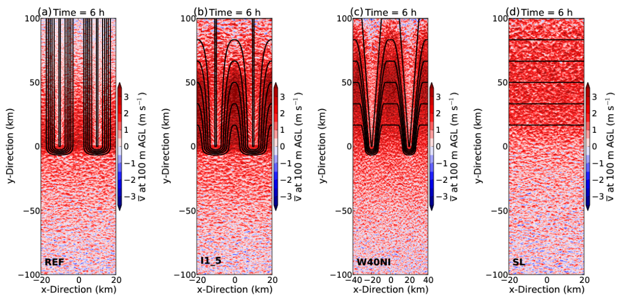
Figure 3. Instantaneous along-valley flow at 100 m AGL after 6 hours of simulation for a) REF, b) I1_5, c) W40NI and d) SL simulation. Black contour lines show the topography with intervals of 0.25 km. The lowermost topography contour line is set to 0.25 km.
