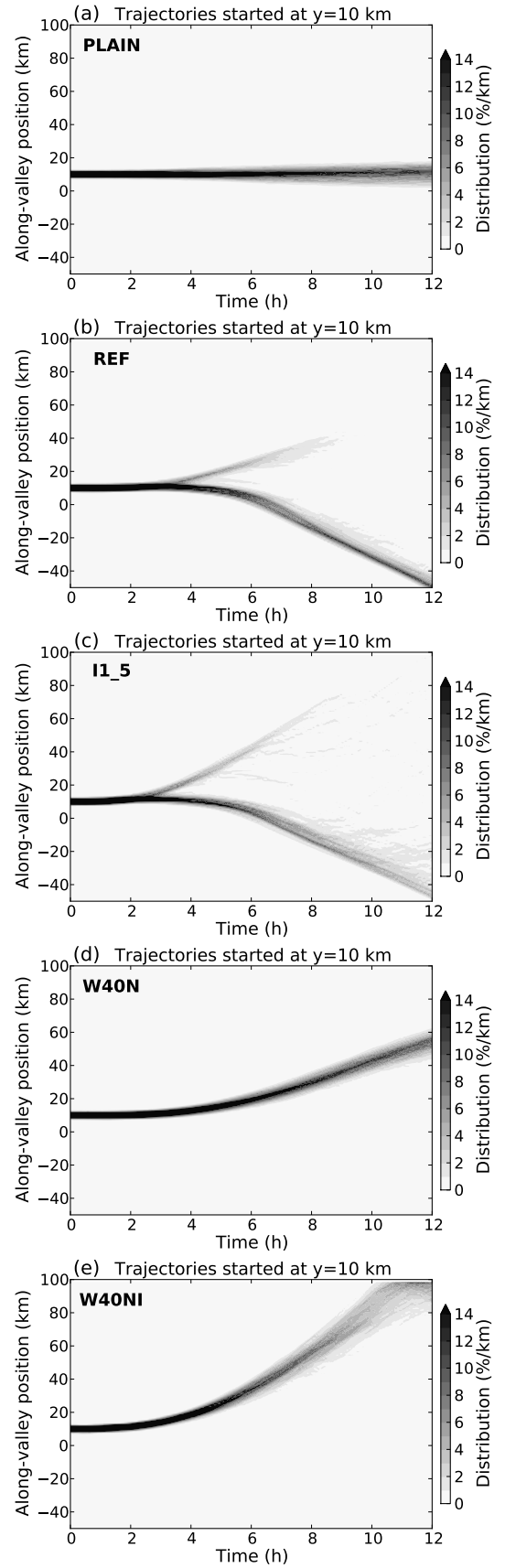
Figure 12. Evolution of parcel along-valley position distribution for trajectories started at y = 10 km for a) PLAIN, b) REF, c) I1_5, d) W40N and e) W40NI simulation. Distribution values are calculated by splitting the along-valley distance into bins of 1 km and determining the percentage of parcels within these along-valley intervals (%/km).
