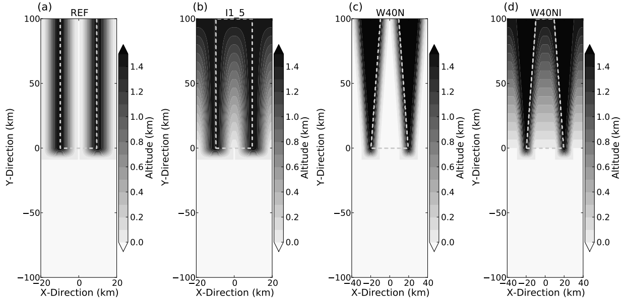
Figure 1. Modelling domain and valley topography for a) REF, b) I1_5, c) W40N and d) W40NI simulations. The dashed grey boxes mark the horizontal areas at crest height, which define the upper surface of a box that is used for computations of valley volume mass flux budgets and valley volume averages of along-valley wind speed.
