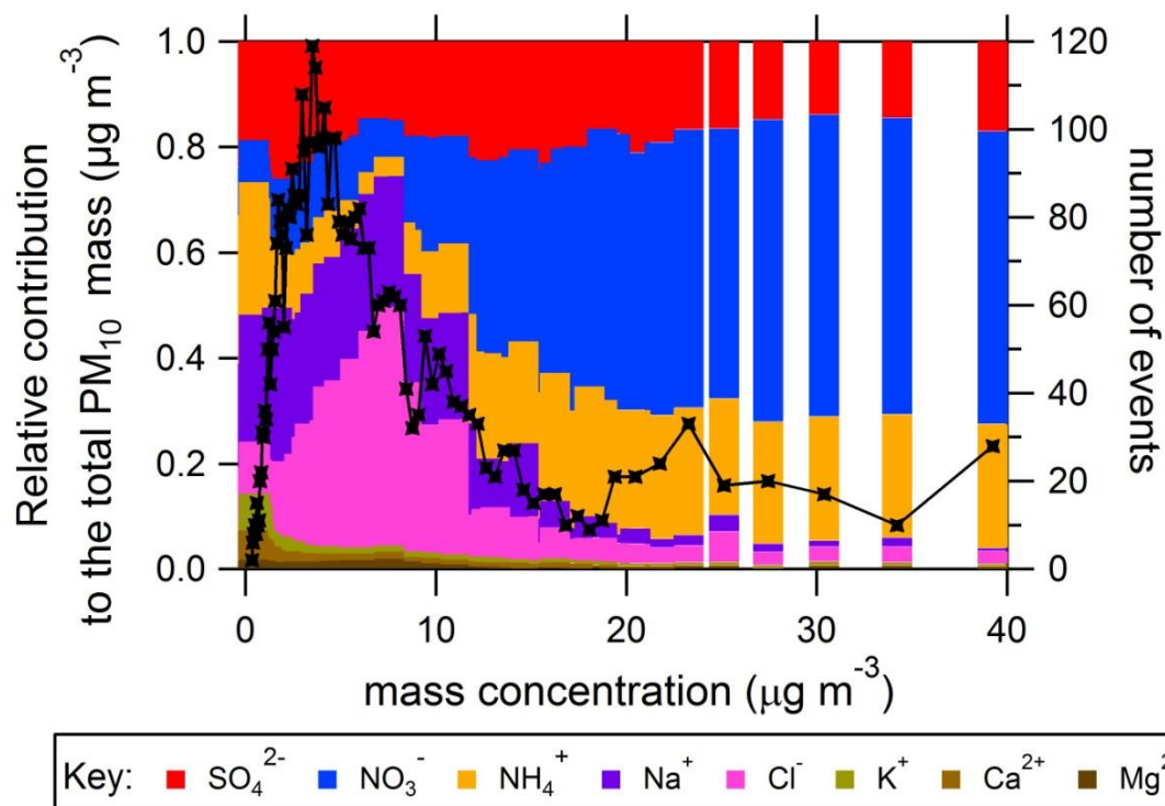
Figure 11. Average relative contribution of inorganic water soluble species to the total PM 10 mass measured by the MARGA during 2012 as a function of total mass concentration. The black line is the number of events at each mass concentration. Graph produced using the plotting routine of Crippa et al. (2014).
