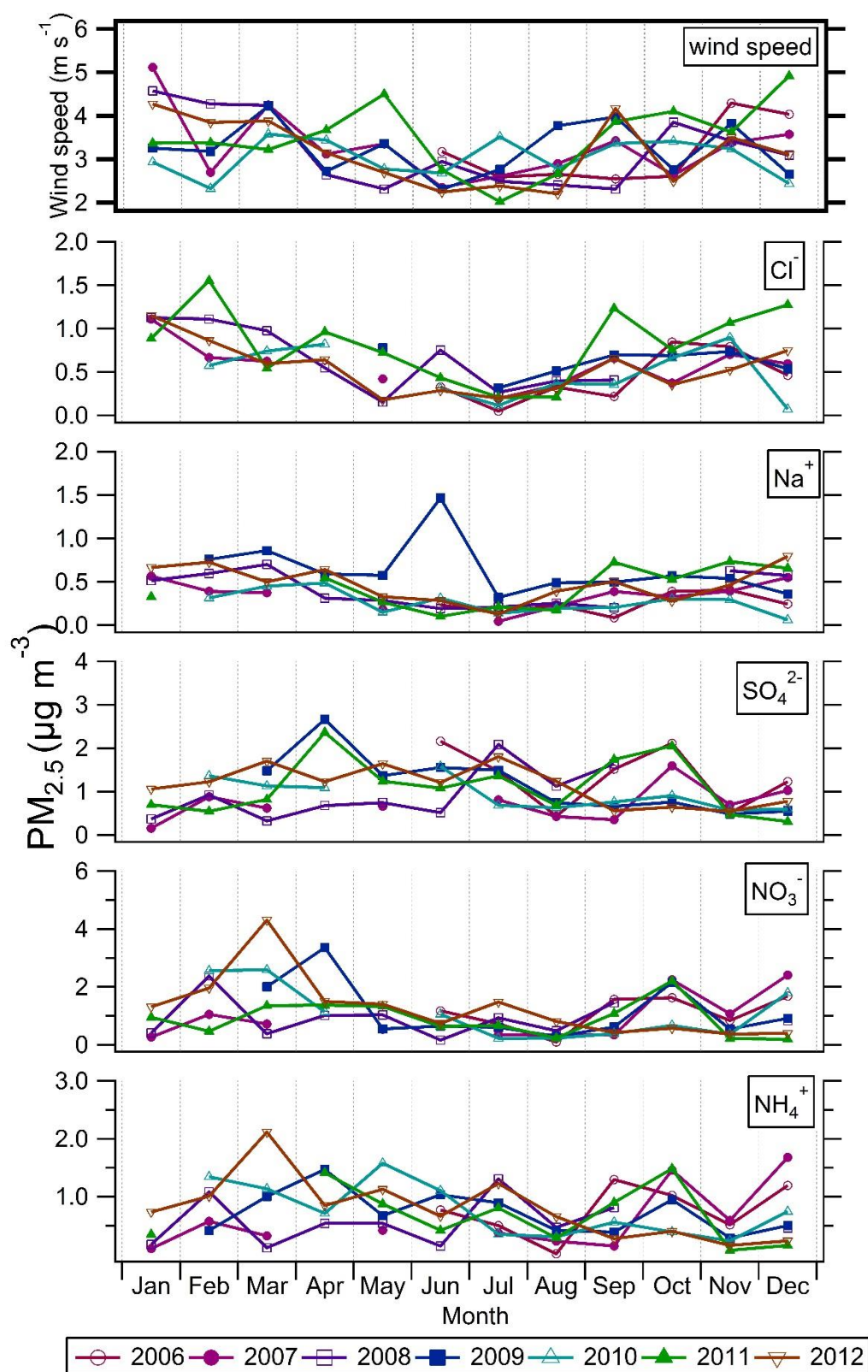
3 Figure 2 a) Median monthly mass concentrations of \text{PM}_{2.5} species measured by the MARGA 4 and median wind speed from June 2006 to December 2012
