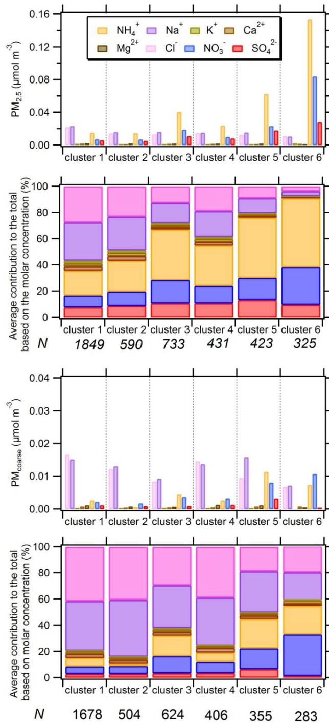
Figure 10. Average molar concentrations and average contribution of the species to the total molar concentration of PM_{2.5} and PM_{coarse} for each back trajectory cluster (refer to Figure 9) from January 2007 to December 2012. Key: N – number of back trajectories used to calculate average concentration and % contribution for each trajectory.
