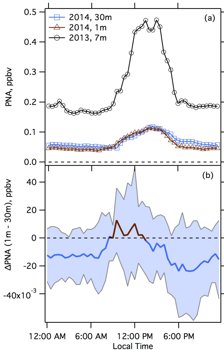
Figure 4. Diurnal profiles of PNA are shown in panel (a) for the full measurement period during the UBWOS 2013 and 2014 studies, with the 2014 study separated based on the sampling height location. Panel (b) presents the difference in the 1m and 30m PNA measurements for duration of the 2014 study, where a positive value (brown) indicates larger concentrations at the ground and a negative value (blue) suggests a relative PNA depletion in the 1m measurements. The shaded region represents 1 standard deviation on the hourly average for the entire measurement period.
