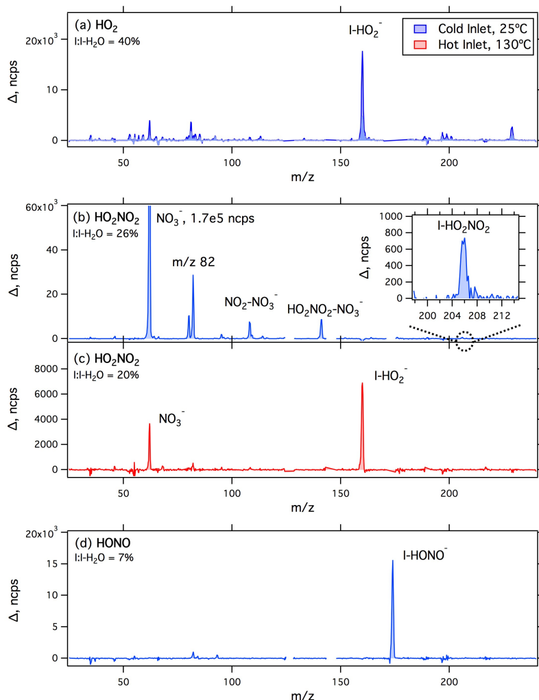
Figure 1. Shown are normalized ( 1\text{e6 cps I}^- ), background corrected mass spectra acquired in the laboratory for calibration sources of \text{HO}_2 (a), \text{HO}_2\text{NO}_2 (b) and (c), and \text{HONO} (d). Spectra colored in blue were collected using a room temperature inlet ( \sim 25^\circ\text{C} ) while spectra in red indicate that an inlet dissociator at a temperature of 130^\circ\text{C} was used. Background mass spectra have been subtracted from the displayed mass spectra to highlight the m/z ions that are produced via the \text{I}^- CIMS ion chemistry. All three species are detectable at a unique m/z , when an inlet dissociator is not used, allowing for simultaneous detection of \text{HO}_2 , \text{HO}_2\text{NO}_2 , and \text{HONO} .
