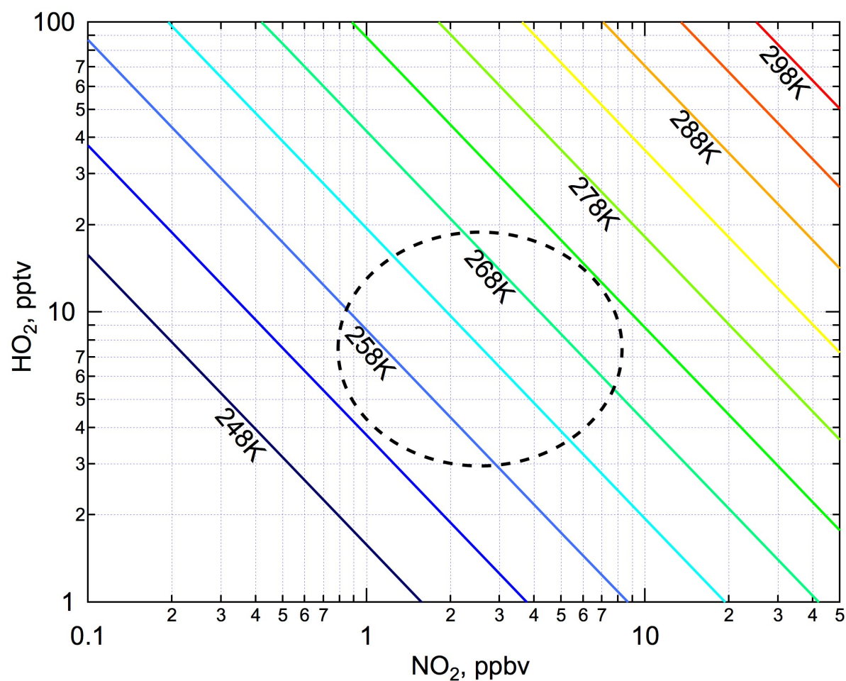
1 2 Figure 5. Temperature and mixing ratios of \text{HO}_2 and \text{NO}_2 required to sustain an equilibrium 3 concentration of 1 ppbv \text{HO}_2\text{NO}_2 . The region within the dashed circle superimposed on the 4 figure highlights the conditions encountered during the 2013 UBWOS study. Data shown were 5 calculated using the IUPAC database (Atkinson et al., 2004).
