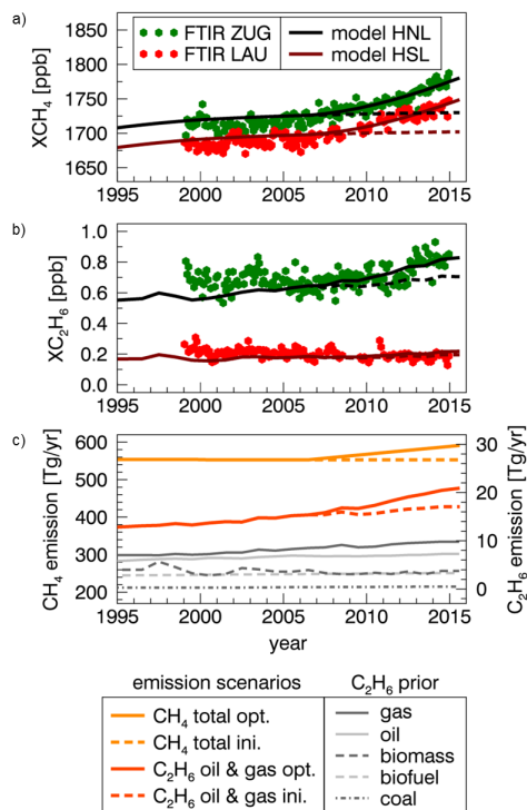
Figure 3. Methane and ethane two-box model: (a) Monthly mean column-averaged methane and (b) ethane from Zugspitze and Lauder FTIR observations. Modeled annual means of XCH_4 and XC_2H_6 are shown for high northern and southern latitudes (HNL, HSL) after emission optimization (solid lines) and with prior emissions (dashed lines). An overall offset is applied to the modeled time series to fit the observed average for 2007–2014. (c) Emission scenario for 2007–2014: optimized global emissions of methane ( CH_4 total opt., left y axis) and ethane from oil and natural gas sources ( C_2H_6 oil & gas opt., right y axis). For comparison, the corresponding initial emission histories are displayed along with prior ethane emissions of all considered source categories.
