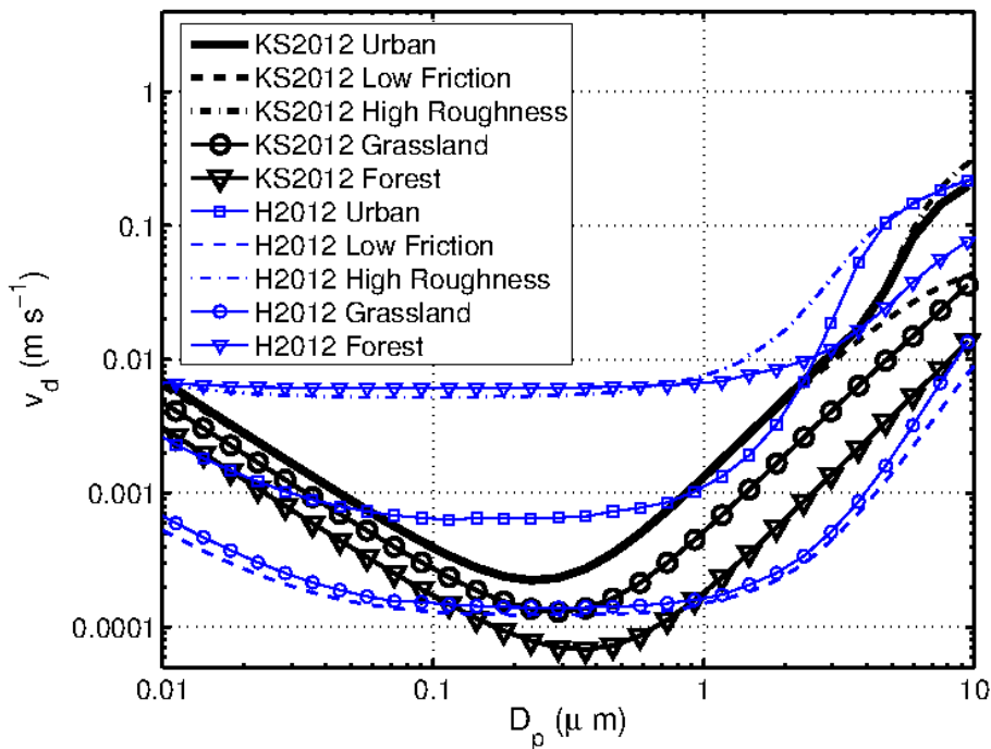
Figure 2. Dry deposition velocity, \nu_d (in \text{m s}^{-1} ) as function of particle diameter D_p (in \mu\text{m} ), using a particle density of 1400 \text{ kg m}^{-3} . The results with the model of Kousnezov and Sofiev (2012) (KS2012) are shown as black lines and the results with the model of Hussein et al. (2012) (H2012) are shown as blue lines. The curve of “KS2012 Urban” (thick black line) represents the dry deposition parameterization that is used in all model runs with MAFOR. The curves for cases “KS2012 Low Friction” (dashed black line) and “KS2012 High Roughness” (dash-dotted black line) partly overlay with the curve for “KS2012 Urban”.
