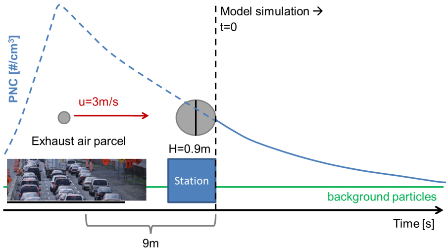
Figure 1. Idealized scenario for model simulations with MAFOR to study aerosol processes between roadside and neighborhood scale. Model simulations start at the point where the exhaust parcel (plume height typically 0.9 m) has approached the roadside traffic station. The simulations are initialized with PN concentration and size distribution measured at roadside. Particle concentrations in the exhaust air are diluted by background air with constant PN concentration.
