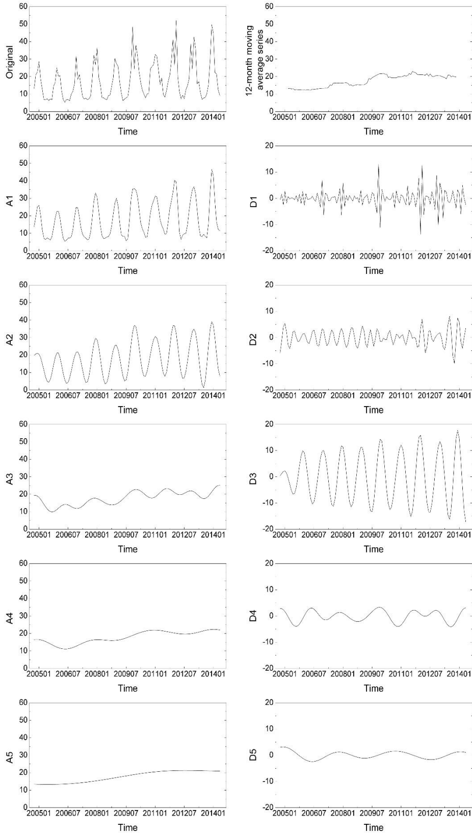
Figure R1. Wavelet analysis results for the OMI NO 2 time series at a grid cell in Xi'an, Shaanxi (34.5°N, 108.9°E). The top left panel shows the original monthly time series, and the top right panel displays the 12-month moving average time series.
