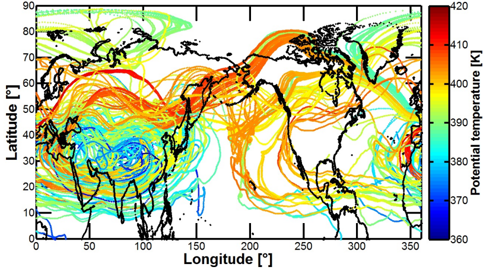
Figure 6. Fifty-day backward trajectories for all data points with flight sections, where \Theta > 370 K, PV > 7.5 pvu. To select trajectories, and minimum \Theta along which experienced a diabatic ascent to the backwards flight level we only show trajectories with a minimum potential temperature which is at least 5 K smaller as below \Theta at the measurement location (cf. Fig. 5). Color: Potential temperature along the backward trajectories based on ERA-Interim reanalysis data.
