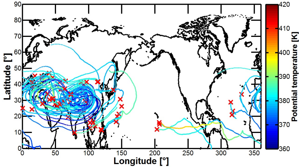
Figure 7. Pathway of the trajectory ensemble as shown in Fig. 6 with PV_{Tra} < 5 pvu. Red crosses mark the location of the trajectories where PV values exceed 5 pvu.
