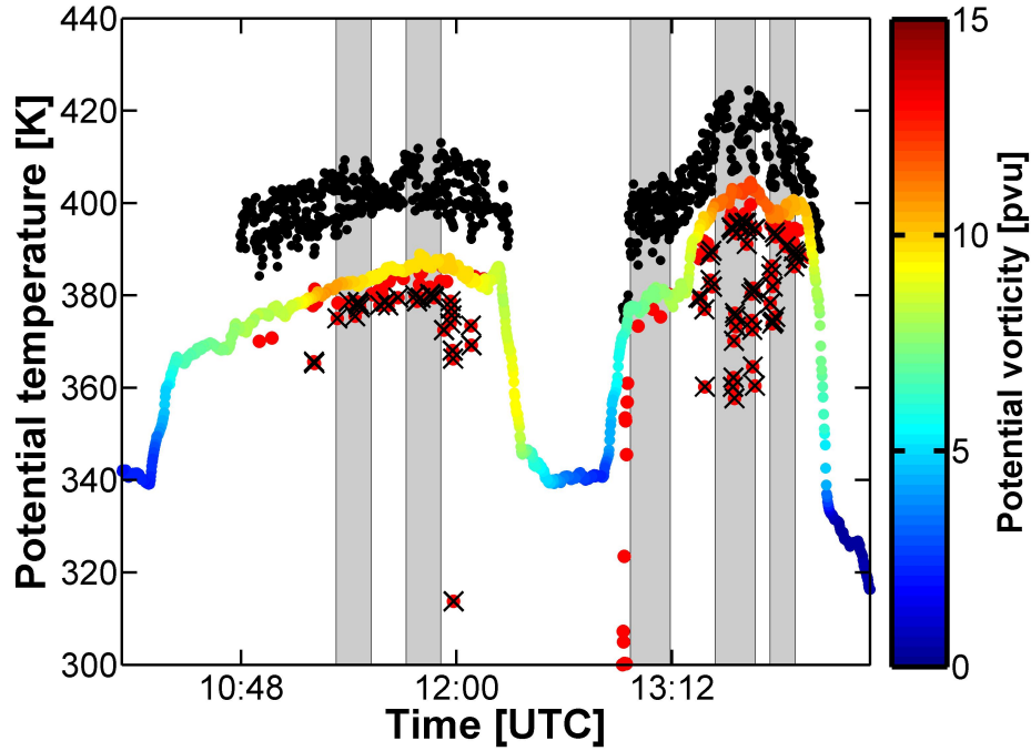
Figure 5. Solid line: Time series of the measured potential temperature \Theta for measured during the second half of TACTS Flight 2 with PV as color (from ECMWF data). Black dots: Maximum potential temperature along 50-day back trajectories for all data points with \Theta > 370 and PV > 4 pvu at the measurement location. Red dots: Minimum further indicate the minimum potential temperature along 50-day back the trajectories for all data points with \Theta > 370 K at flight sections, PV > 4 pvu, and where this minimum \Theta along the backwards trajectories is smaller as \Theta at below the measurement measured values along the flight track. Red dots with PV > 7.5 pvu and minimum \Theta at least 5 K smaller as \Theta at the measurement are marked with a black cross (cf. Fig. 6).
