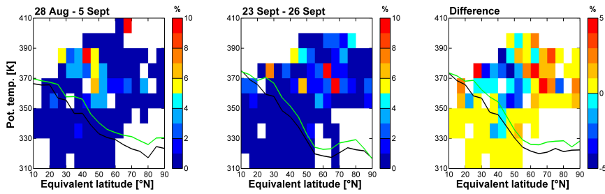
Figure 12. Same presentation as in Fig. 11 but with different color coding. Proportion Fraction of data points for which 50-day-fifty-day backward trajectories calculated with CLaMS-TRAJ indicate an origin in the Asian summer monsoon anticyclone (Criterion: 25^\circ\text{N} < \text{TRA-latitude} < 40^\circ\text{N} , 40^\circ\text{E} < \text{TRA-longitude} < 110^\circ\text{E} and \text{Tra-}\Theta > 360\text{ K} for t = -30 days).
