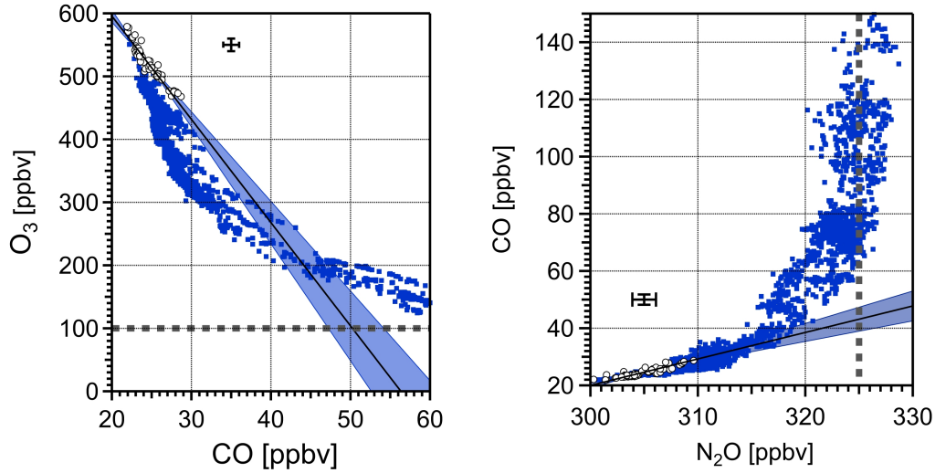
Figure 4. Linear fitting-fits for ML 4 based on the FITEXY-routine described in Press et al. (1992). Blue dots: Scatter plot of CO and O 3 (left), and N 2 O and CO (right), respectively. White dotsCircles: Data-Individual data points of ML 4 on-forming the respective scatter-plot-mixing line ML 4. Solid black line: Linear fit with confidence region (shaded area). Dotted lines :-Assumption of a-indicate typical tropopause mixing ratios for O 3 and N 2 O, respectively to determine the tropospheric endmember of mixing line 'end member' ( R(O_3)_{Trop} = 100 ppbv (top) and R(N_2O)_{Trop} = 325 ppbv (bottom)). Uncertainties are separately shown as black crosses.
