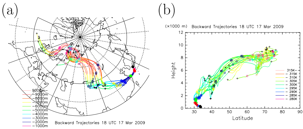
Figure 6. Backward trajectories starting at 18:00 UTC 17 March 2009 (case 1). (a) Horizontal component of the routes and (b) routes in the latitude-vertical section of the top-1% trajectories (18 lines) and the top-25% averaged trajectory (thick line) are shown. The colors are the same as those in Fig. 3. The \circ symbol indicates positions at each 24 h interval, whereas the + symbol shows the fifth day and the last. The difference in days is represented by different colors.
