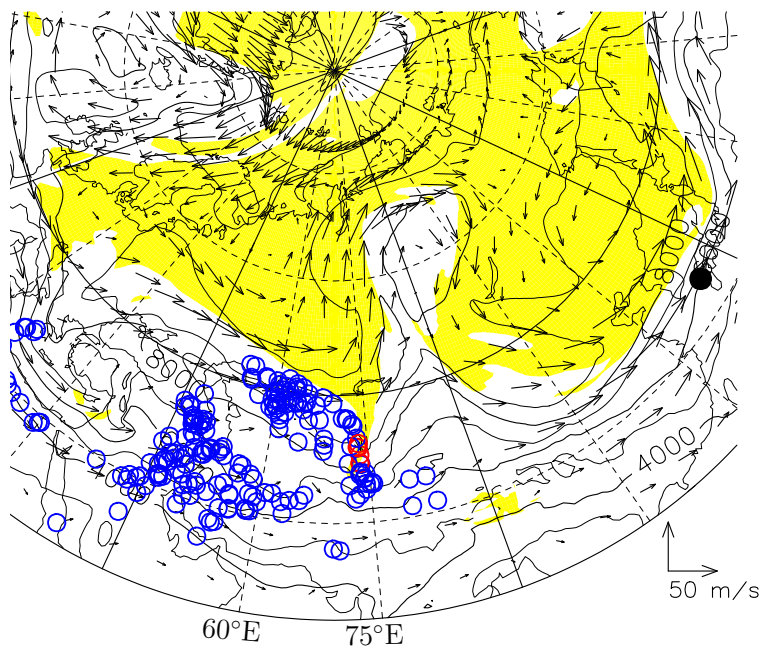
Backward Trajectories 18 UTC 25 Dec 2009 310K 18 UTC 16 Dec 2009
