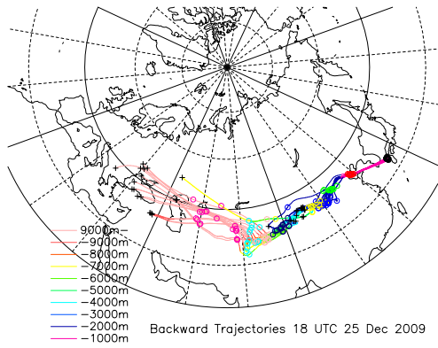
Figure 13. Same as Fig. 6 except for case 7 (starting time of 18:00 UTC 25 December 2009).
