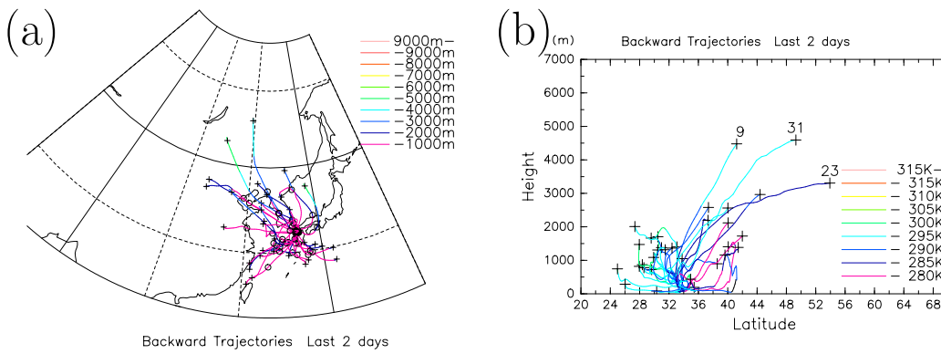
Figure 5. Top-1% averaged trajectories for the last two days of travel. (a) Horizontal component of the trajectories and (b) trajectories in the latitude-vertical section for all 33 cases are shown. The colors are the same as those in Fig. 3. The + symbol indicates the position before two days of object times for analysis. The three numerals (9, 23, and 31) in panel (b) indicate the case numbers.
