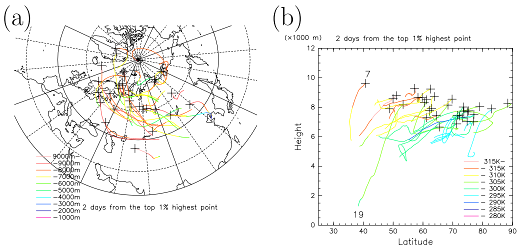
Figure 3. Top-1% averaged trajectories for two days from their highest altitude. (a) Horizontal component of the trajectories and (b) trajectories in the latitude-vertical section for all 33 cases are shown. Colors indicate altitudes in panel (a) and potential temperature in panel (b) . The symbol + shows the position of the highest altitude of each top-1% averaged trajectory. The two numerals, 7 and 19, are the case numbers.
