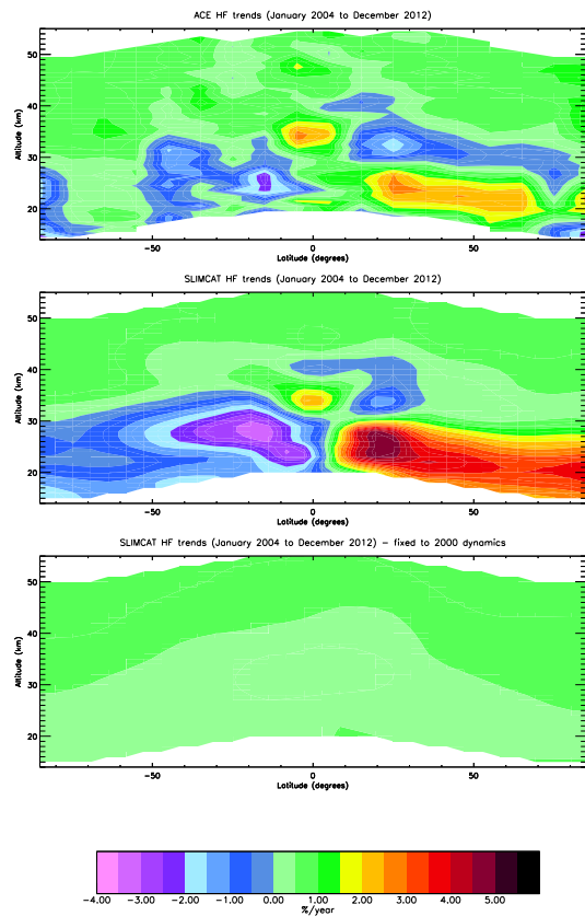
Figure 8. Trends in the growth of HF ( \% \text{ year}^{-1} ; January 2004 to December 2012) for ACE-FTS and SLIMCAT as a function of latitude and altitude. A full discussion of these trends is provided in the text.
