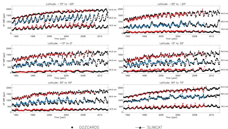
Figure 7. The GOZCARDs and SLIMCAT HF time series for selected altitude–latitude bin combinations. Observations are plotted between October 1991 and September 2010.
