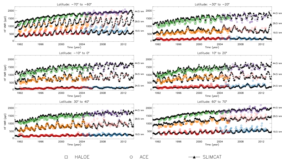
Figure 6. The HALOE, ACE-FTS and SLIMCAT HF time series for selected altitude–latitude bin combinations. Observations are plotted between October 1991 and December 2012.
