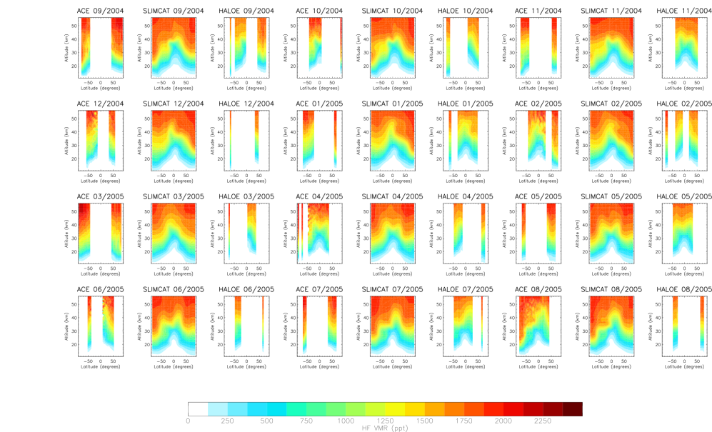
Figure 2. A comparison between ACE-FTS, HALOE and SLIMCAT HF zonal means (September 2004 to August 2005). The ACE-FTS and HALOE time series of measurements overlap during the period January 2004 to November 2005.
