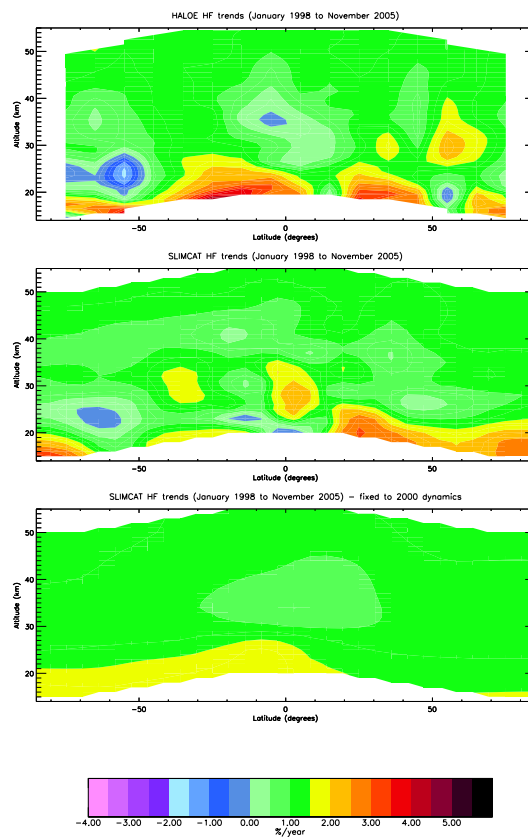
Figure 10. Trends in the growth of HF ( \% \text{ year}^{-1} ; January 1998 to November 2005) for HALOE and SLIMCAT as a function of latitude and altitude. A full discussion of these trends is provided in the text.
