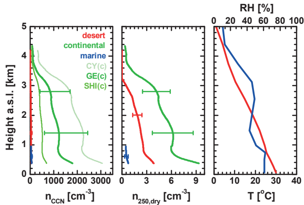
Fig. 11. (Left) Particle number concentration n_{CCN} for a supersaturation of ss = 0.15\% . The thick green (GE(c) conversion parameters), red, and blue profiles are obtained with Eqs. (10)–(12) for continental, desert, and marine aerosol, respectively. The thin light green profile (CY(c)) is obtained with Cyprus conversion parameters, and SHI(c) (thin green) with the parameterization of Shinozuka et al. (2015) (see text for more explanations). (Center) Large-particle number concentration n_{250,dry} , computed with Eqs. (4)–(6). (Right) GDAS temperature and relative-humidity profiles for Limassol on 16 August 2012.
