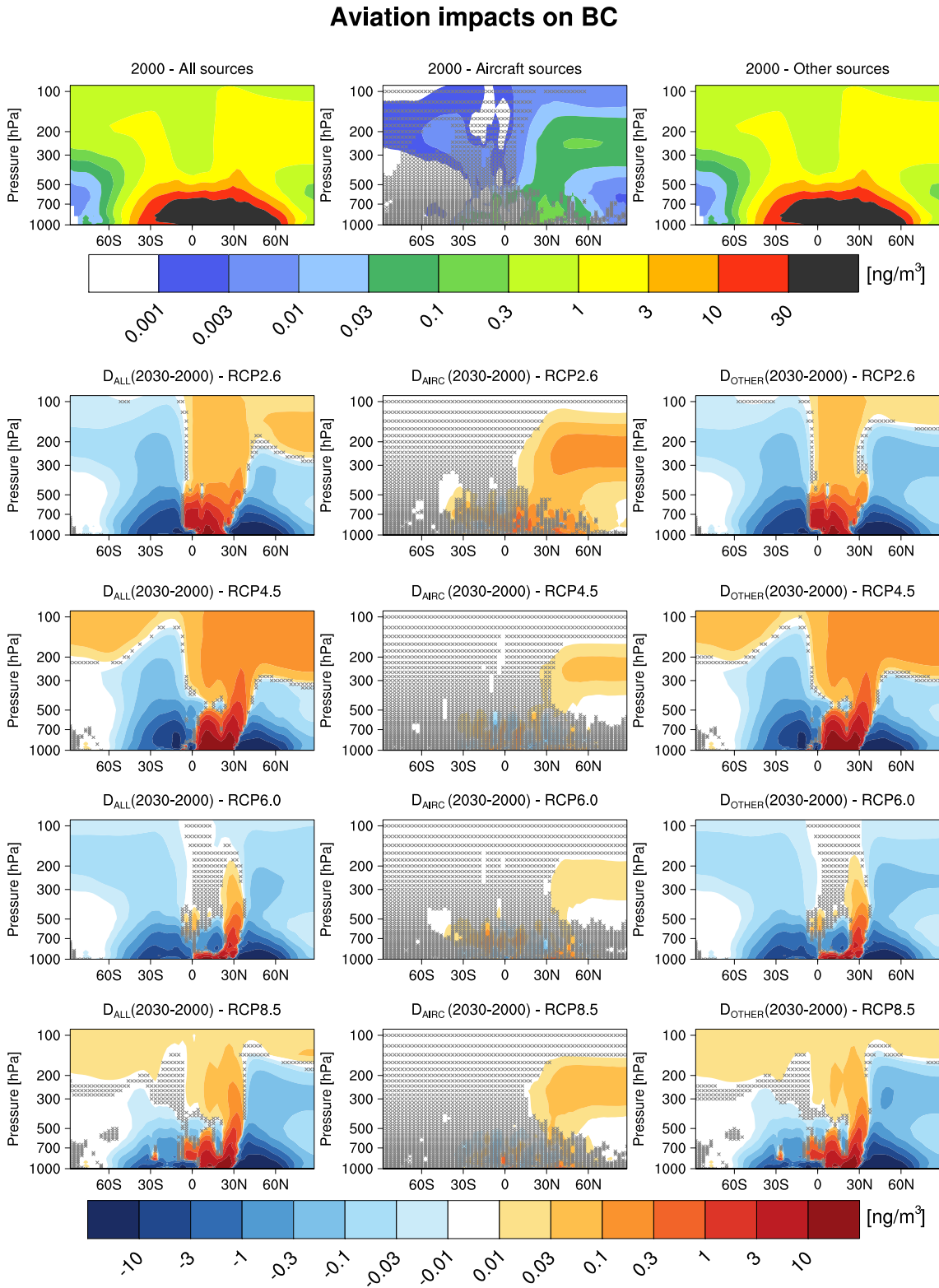
Fig. 3. Annual average zonal mean concentrations of BC. The first row shows the results for year 2000 emissions: Total concentration ( REF_{2000} , left), the concentration induced by aviation ( \Delta_{2000}^{AIRC} , middle) and the concentration induced by other sources ( NOAIRC_{2000} , right). The lower four rows show the changes in these quantities between 2000 and 2030 for the four RCPs, as given in Eqs. (2)–(4). Grid points where the difference is not statistically significant according to a univariate t test (5 % error probability) are hatched.
