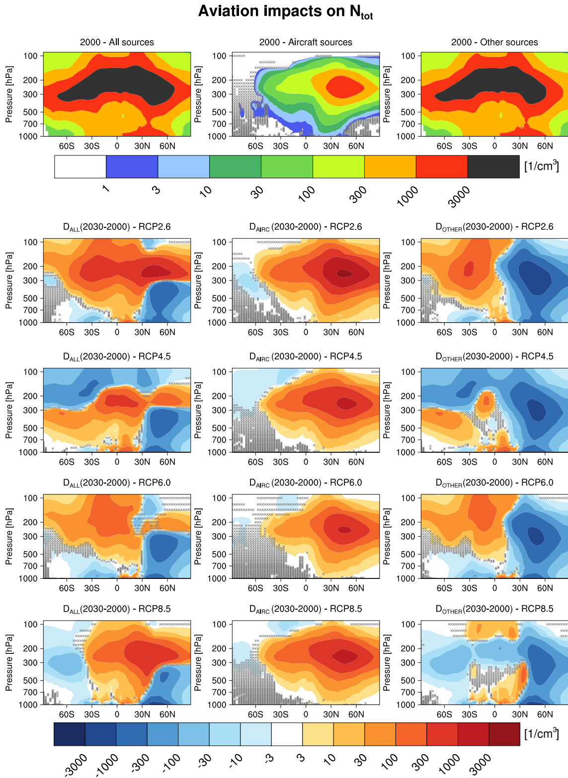
Fig. 6. As in Fig. 3, but for fine particle ( <1 \mu\text{m} , sum of the Aitken and accumulation mode particles) number concentrations.
