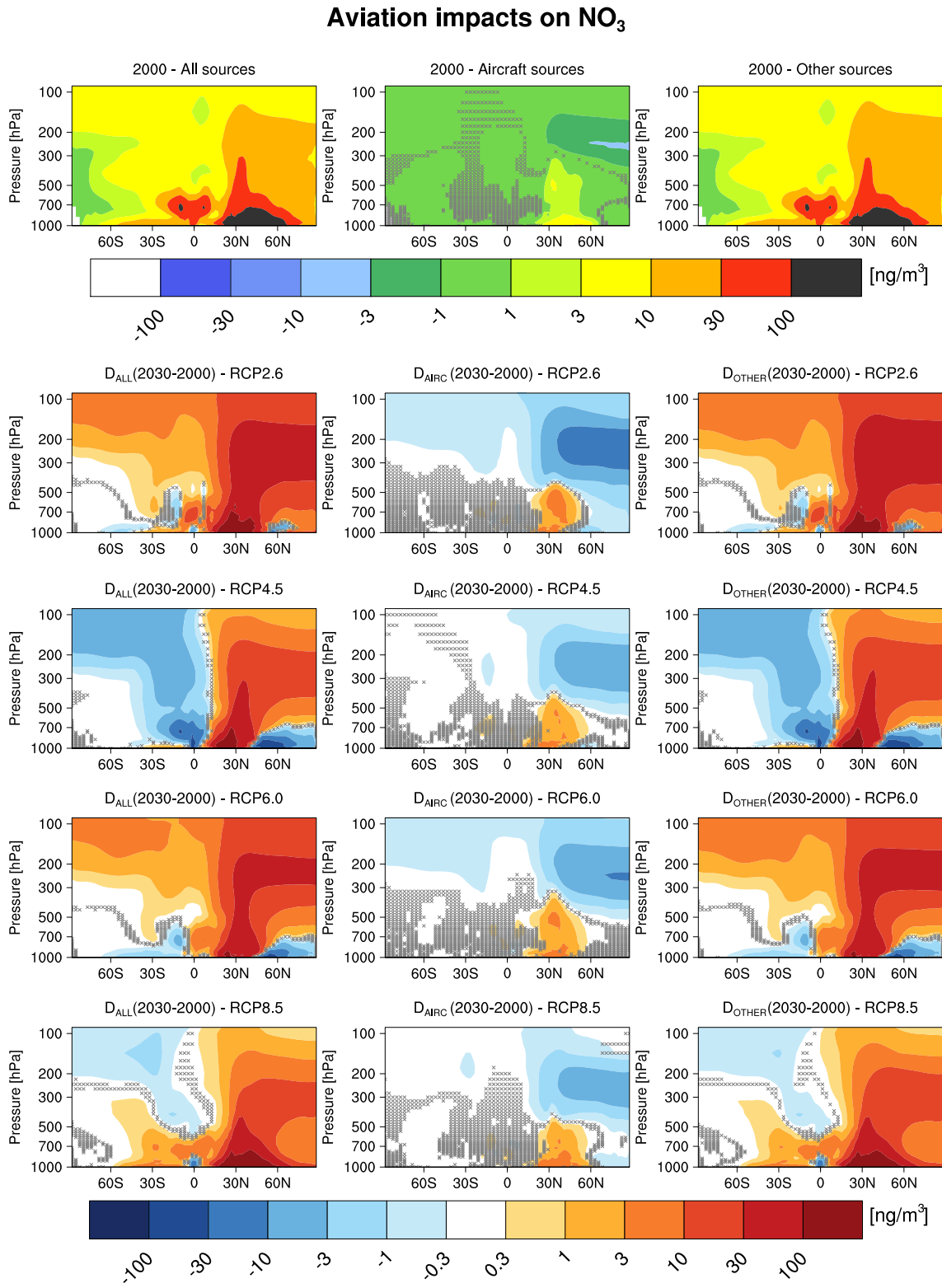
Fig. 5. As in Fig. 3, but for aerosol nitrate concentration.
