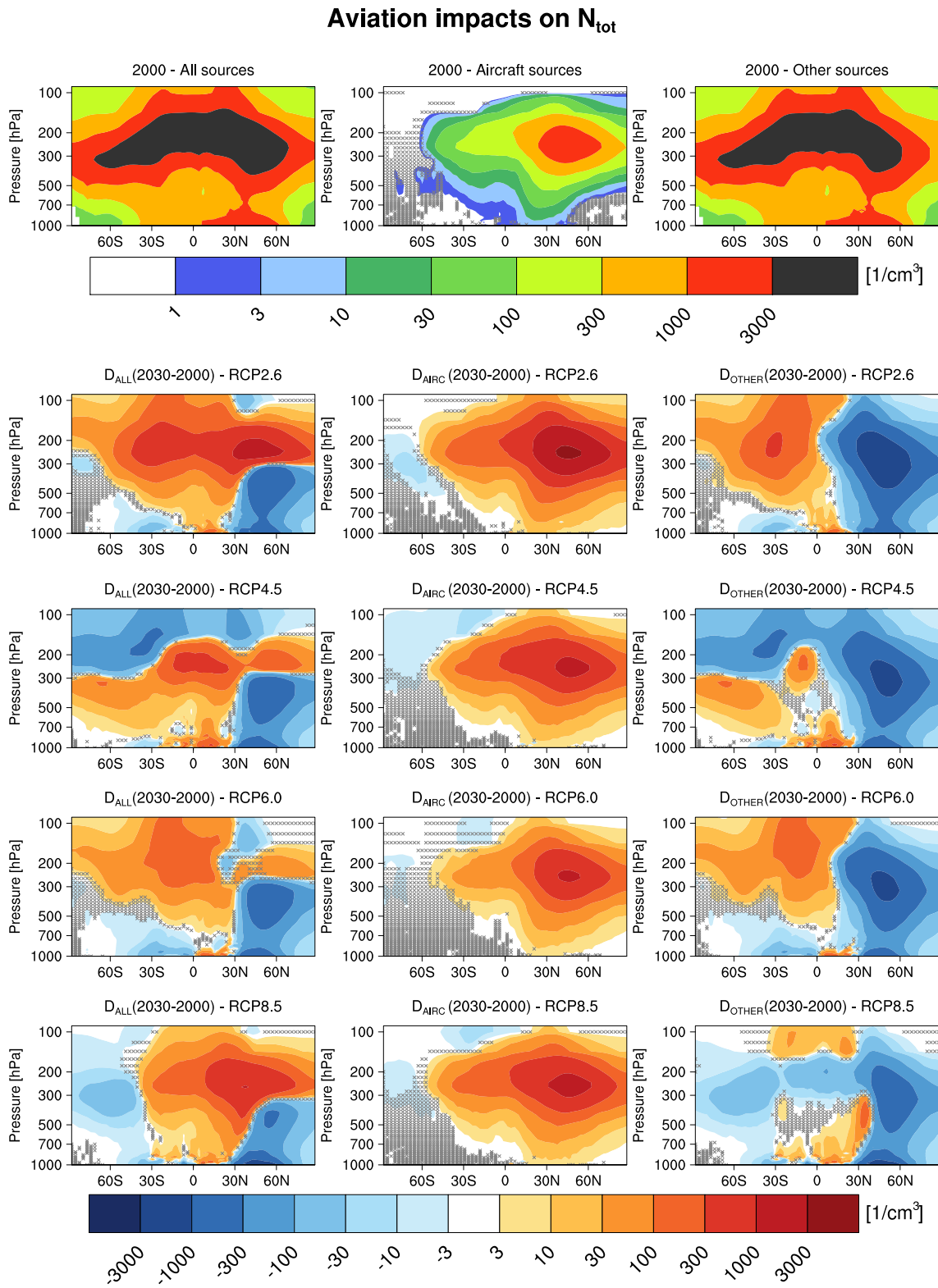
Fig. 6. As in Fig. 3, but for fine particle ( \lesssim 1 \mu\text{m} , sum of the Aitken and accumulation mode particles) number concentrations.
