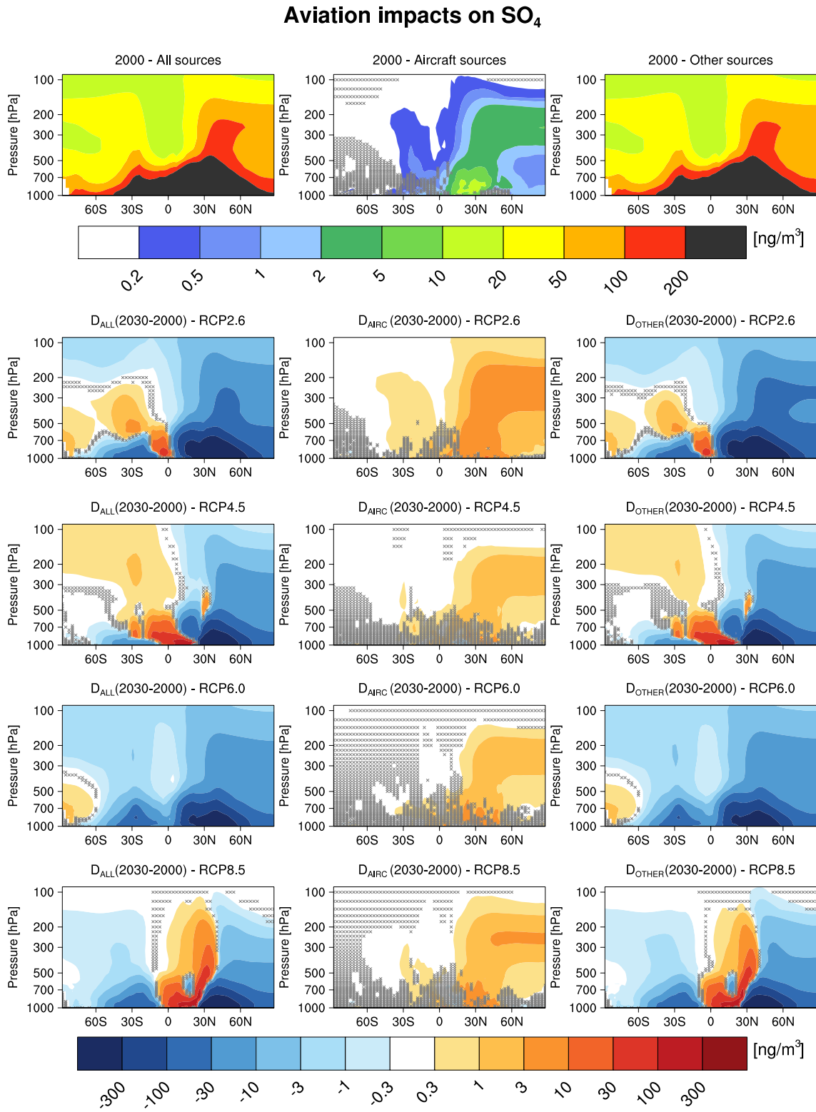
Fig. 4. As in Fig. 3, but for aerosol sulfate concentration.
