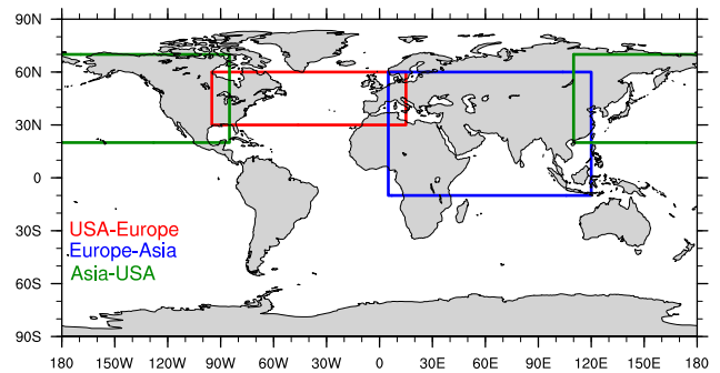
Fig. 1. The regions selected for the analysis of the aviation impacts.
