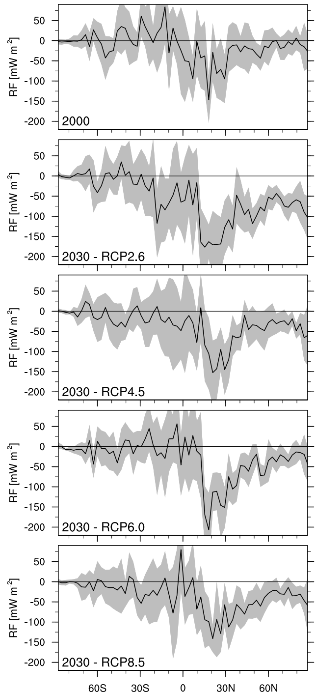
Fig. 9. Zonal mean all-sky RF resulting from aviation emissions in the year 2000 and 2030 for the four RCP scenarios (from top to bottom, respectively). The gray shadings represent the 95 % confidence interval with respect to the interannual variability.
