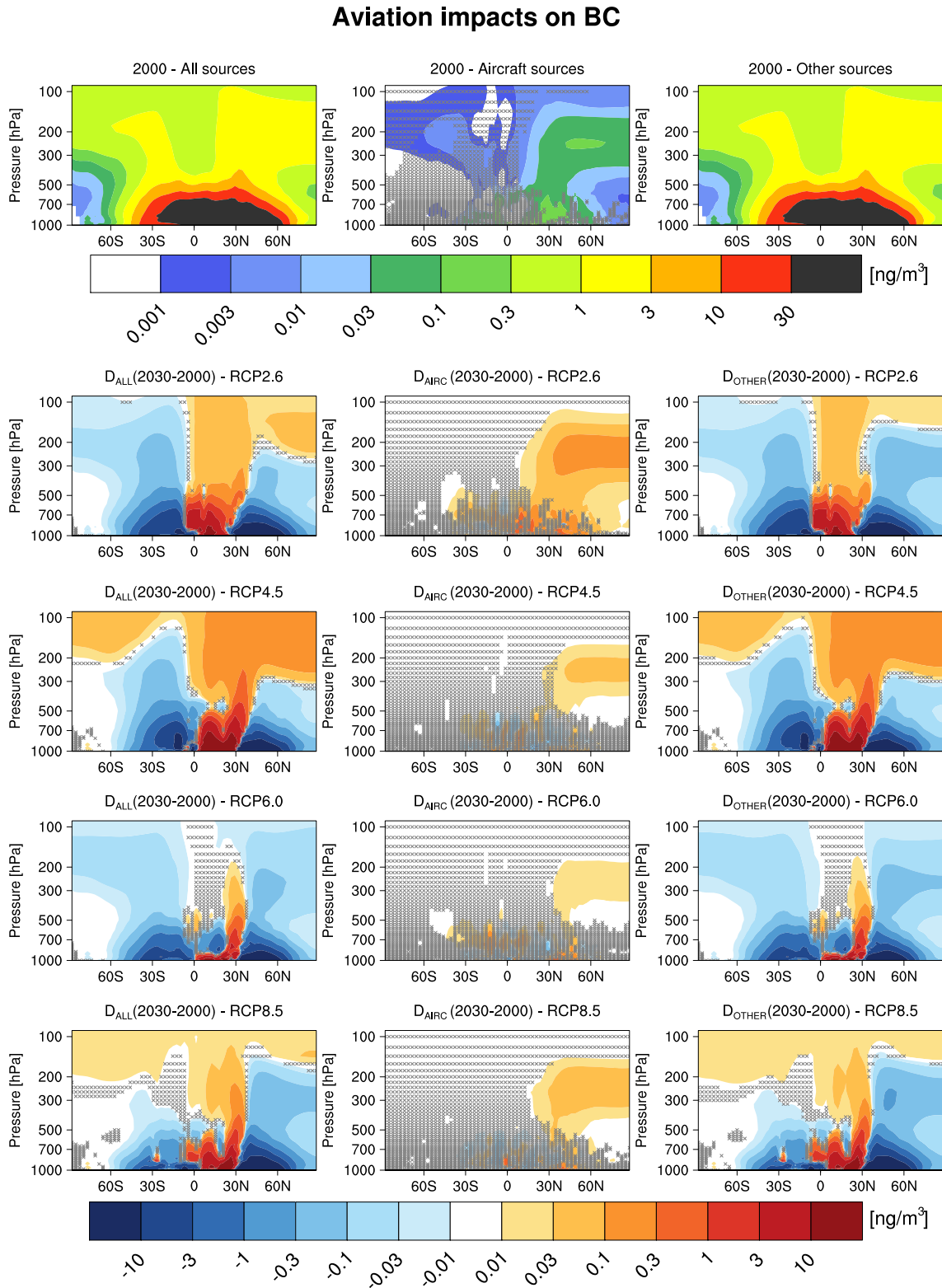
Fig. 3. Annual average zonal mean concentrations of BC. The first row shows the results for year 2000 emissions: Total concentration ( \text{REF}_{2000} , left), the concentration induced by aviation ( \Delta_{2000}^{\text{AIRC}} , middle) and the concentration induced by other sources ( \text{NOAIRC}_{2000} , right). The lower four rows show the changes in these quantities between 2000 and 2030 for the four RCPs, as given in Eqs. (2)–(4). Grid points where the difference is not statistically significant according to a univariate t test (5 % error probability) are hatched.
