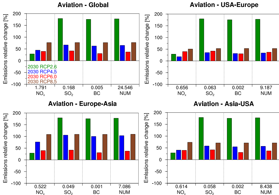
Fig. 2. Relative changes in the emissions from aviation in the year 2030 with respect to 2000, for the four RCP scenarios. The changes are displayed globally (top left) and for the regions defined in Figure 1. Total emissions for the year 2000 are indicated at the bottom of each panel, in units of Tg(species)a -1 for SO 2 and BC, Tg(NO)a -1 for NO x , and 10 25 particles a -1 for particlenumbers(NUM).
