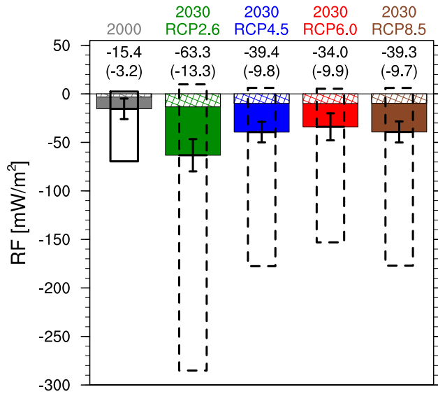
Fig. 8. Global mean all-sky RF resulting from aviation emissions in the year 2000 (gray bar) and for the four RCP scenarios in 2030 (colored bars). The hatched part of each bar is the corresponding clear-sky forcing, calculated neglecting the radiative effects of clouds. The numerical values of the all-sky (clear-sky) forcing are shown on top of each bar in units of \text{mW m}^{-2} . The whiskers represent the 95 % confidence interval with respect to the interannual variability. The boxes correspond to the uncertainty range derived from the assumption on the size distribution of emitted particles and fuel sulfur content, as calculated by R13 for the year 2000 (solid) and rescaled here to the 2030 values (dashed).
