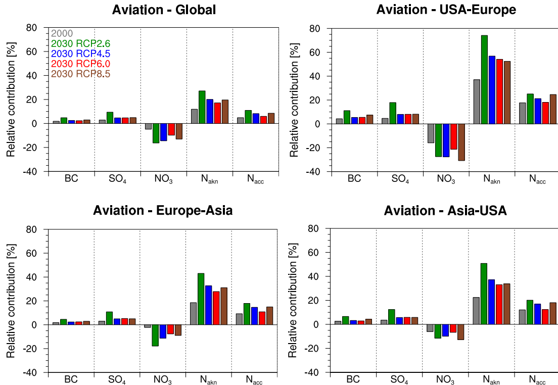
Fig. 7. Relative contributions of aviation to the average mass and number burdens of selected aerosol species and different particle size modes (Aitken and accumulation mode), respectively. Results are shown for the year 2000 and for the four RCP scenarios in 2030. The values are integrated in model layers 7 to 9 (~8–13 km) globally and in three different regions (defined in Fig. 1).
