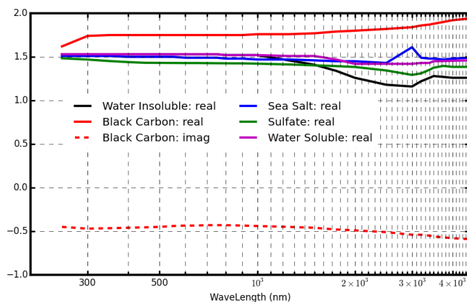
Figure 3. The real or imaginary parts of the refractive indices of aerosol chemical positions used in OPAC.
