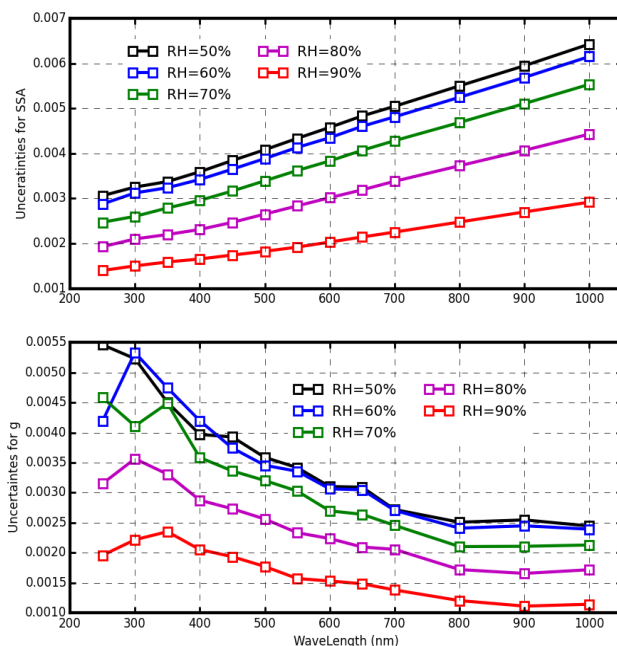
Figure 4. Uncertainties for SSA and g at different RH levels and wavelengths.
