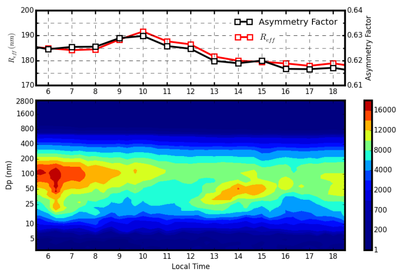
Figure 5. The diurnal variations of PNSD, the effective radius and g of aerosol particles at dry state.
