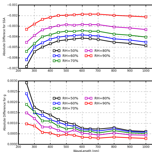
Figure 2. The absolute difference for SSA and g , when i_{non} is changed from 10^{-7} to 0.001.
