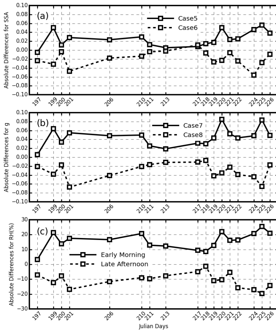
634 635 Figure 6. The absolute differences between early morning (or late afternoon) average and the daytime average of SSA, g, 636 and RH. (a) For SSA: corresponding to Case 5 and 6; (b) For g: corresponding to Case 7 and 8; (c) For RH.
