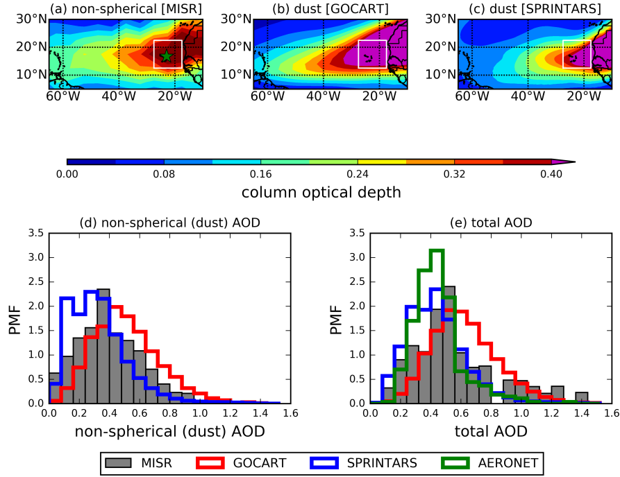
Figure 4. (a) Climatological mean optical depth of the non-spherical aerosols in MISR, dust AOD in (b) GOCART and (c) SPRINTARS over the Eastern Atlantic for July. Data from the eight Julys between 2000 and 2007 are averaged for MISR and GOCART. Spatio-temporal distributions of (d) the non-spherical (or dust) AOD and (e) total AOD from MISR (grey bars), from GOCART (red lines), and from SPRINTARS (blue lines), covering the boxed region ( 112.5^{\circ}E - 122.5^{\circ}E, 32.5^{\circ} - 37.5^{\circ}N ) off the coast are displayed. The green star in (a) displays a location of the AERONET station in Capo Verde. The green line in (e) represents the total AOD distribution in Capo Verde for July 2005.
