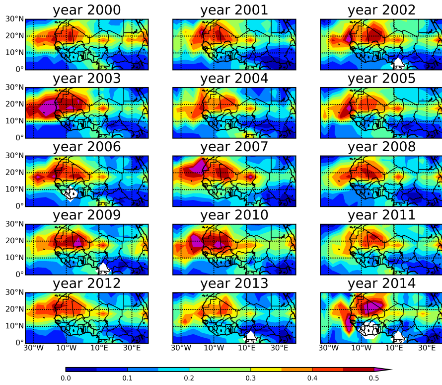
Figure 5. Monthly mean optical depth of the non-spherical aerosols from MISR in July for 15 years between 2000 and 2014. The white blank spots indicate that there were no retrieved non-spherical AOD for the month.
