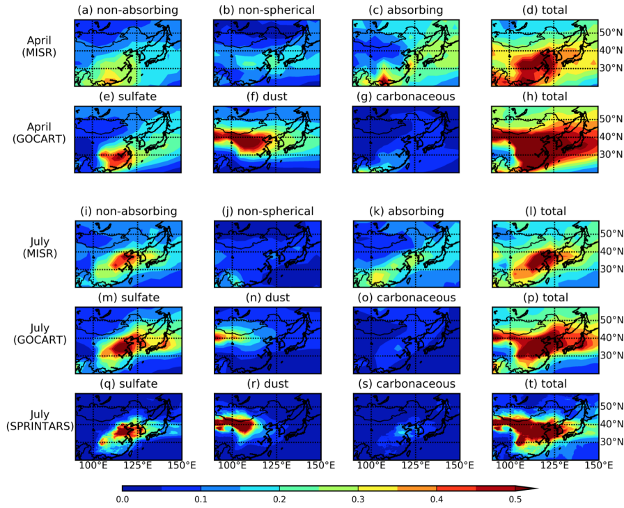
Figure 3. Maps of average MISR optical depth of spherical non-absorbing aerosols, non-spherical, spherical absorbing aerosols and total aerosols in April ((a)-(d)) and July ((i)-(l)). Maps of average GOCART optical depth of sulfate, dust, carbonaceous and total aerosols in April ((e)-(h)) and July ((m)-(p)). Maps of average SPRINTARS optical depth of sulfate, dust, carbonaceous and total aerosols in July ((q)-(t)).
