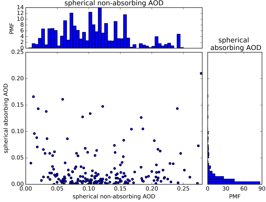
Figure 1. A scatter plot of spherical absorbing-component AOD and spherical non-absorbing-component AOD at 558 nm wavelength and their histograms over East Asia ( 117.5^{\circ} - 127.5^{\circ}E, 32.5^{\circ} - 42.5^{\circ}N ) in April between 2000 and 2014. The AOD data are from MISR Version 1 of the Level 3 Joint Aerosol product (JOINT_AS) based on the Version 22 operational Level 2 aerosol retrievals. The two histograms for spherical non-absorbing and absorbing-component AOD are scaled to show a probability mass function (PMF) so that the total area of the bars in each histogram becomes one.
