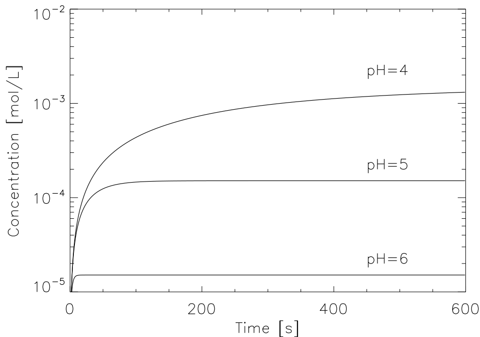
Figure 8. The aqueous phase concentration of \text{NH}_4^+ in a 7\text{ }\mu\text{m} diameter water droplet, exposed to a 22 pptv \text{NH}_3 gas phase, similar to the conditions of experiment CLD8_20_11_1b.
