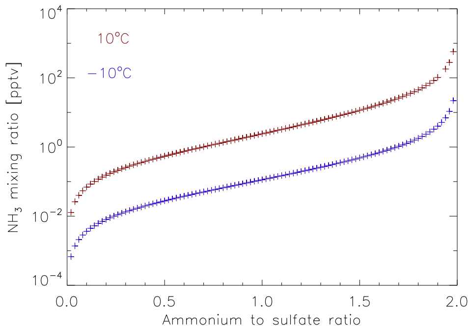
Figure 7. The equilibrium gas phase ammonia mixing ratio, calculated with E-AIM, as a function of the ammonium to sulphate ratio of the aerosol. Data shown are for -10 and 10^{\circ}\text{C} , at \text{RH} = 95\% .
