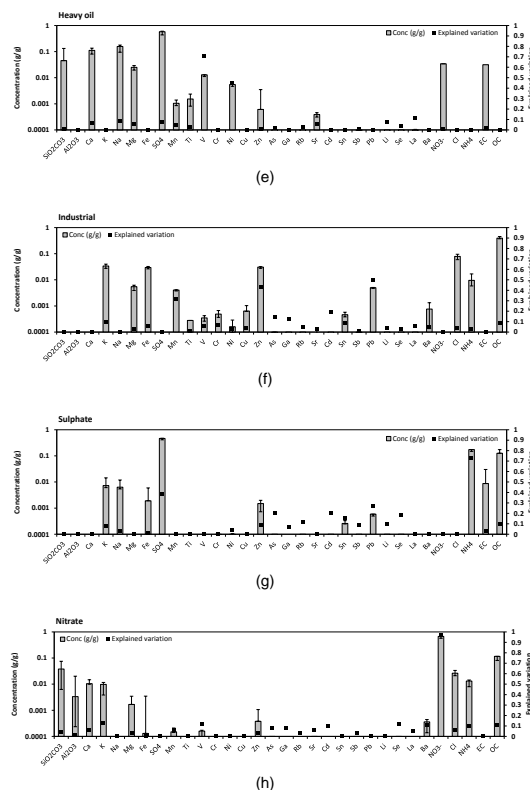
Figure 4. PMF sources profiles for PM 10 during the SAPUSS campaign: (a) vehicle exhaust and wear, (b) road dust, (c) mineral, (d) aged marine, (e) heavy oil, (f) industrial, (g) sulphate, (h) nitrate. Uncertainties were obtained by bootstrapping.
