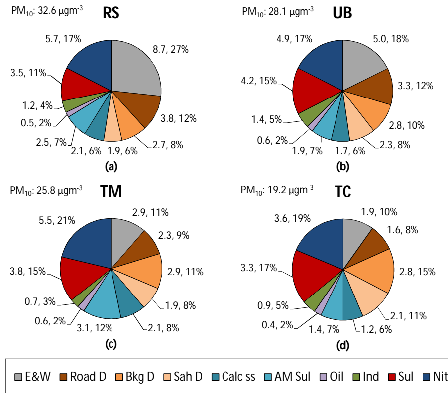
Figure 9. Sources contributing to the PM 10 load extracted with the PMF tool and subcomponents at each monitoring: (a) RS, (b) UB, (c) TM and (d) TC. Exhaust&Wear (E&W), Road dust (Road D), Heavy oil (Oil), Industrial (Ind), Sulphate (Sul) and Nitrate (Nit) are direct PMF factors. The mineral factor was broken into Background dust (Bkg D) and Saharan dust (Sah D) and the aged marine factor into Calculated sea salt (Calc ss) and Anthropogenic marine sulfate of regional origin (AM Sul). Data are given in µgm -3 and %. The average PMF PM 10 concentration are represented at the top left of each graph for each site.
