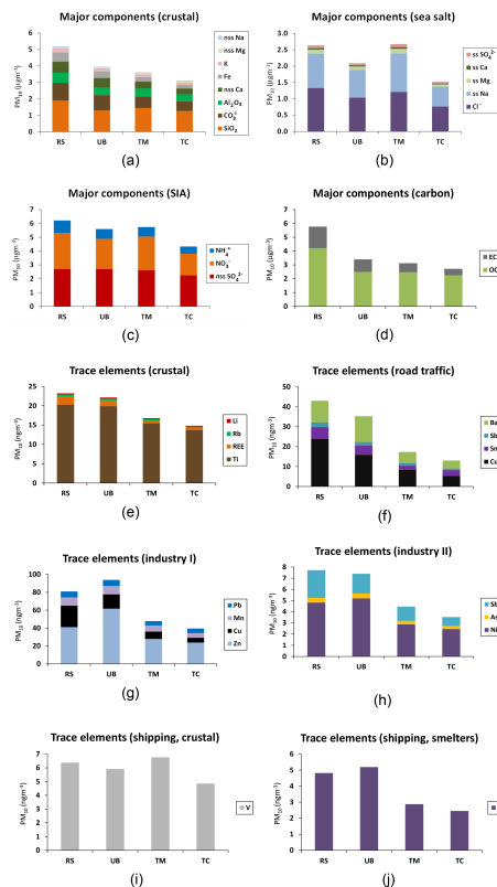
Figure 3. Average PM 10 concentration of main and trace elements for different emission sources at each site (RS: Road Site, UB: Urban Background, TM: Torre Mapfre, TC: Torre Collserola). REE denote Rare Earths elements.
