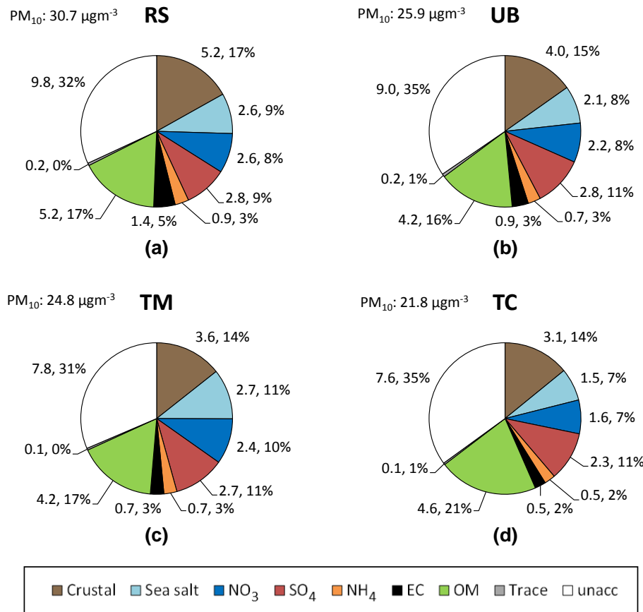
Figure 2. Mean composition of PM 10 concentration in µgm -3 measured during the SAPUSS campaign at: (a) Road Site (RS), (b) Urban Background (UB), (c) Torre Mapfre (TM) and (d) Torre Collserola (TC). Data are given in µgm -3 and %. On the top right of each graph average gravimetric PM 10 concentration are represented.
