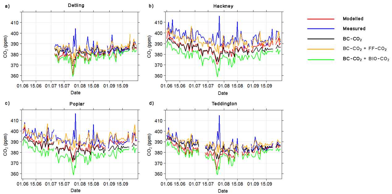
1 2 Figure 4: Time series of averages for the afternoon period (12:00 to 17:00) each day of 3 modelled CO 2 mole fractions (red), measured CO 2 mole fractions (blue), modelled signature 4 of the CO 2 boundary condition mole fractions from MACC-II CO 2 (BC-CO 2 , mole fractions 5 from MACC-II (black), the and modelled CO 2 mole fractions (red) modelled signature of the 6 CO 2 fossil fuel emissions added to that of the boundary conditions BC-CO 2 and fossil fuel 7 CO 2 (BC-CO 2 + FF-CO 2 , orange) and the modelled signature of the CO 2 NEE added to that of 8 the boundary conditions BC-CO 2 and biological CO 2 (BC-CO 2 + BIO-CO 2 , green) at a) 9 Detling, b) Hackney, c) Poplar and d) Teddington.
