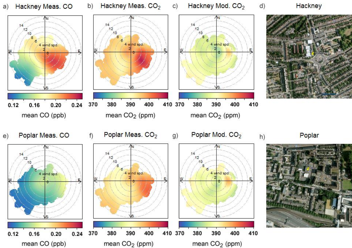
2 Figure 2: Wind roses for each urban measurement site incorporating hourly data for wind 3 speed, wind direction (Heathrow measured data) and CO 2 mole fraction between the hours 4 12:00 and 17:00 for a) observed CO mole fractions at Hackney, b) observed CO 2 mole 5 fractions at Hackney, c) modelled CO 2 mole fractions at Hackney, d) a map (© 2012 Google- 6 Imagery and Bluesky, the GeoInformation group) of the immediate vicinity of the Hackney 7 site, e) observed CO mole fractions at Poplar, f) observed CO 2 mole fractions at Poplar, g) 8 modelled CO 2 mole fractions at Poplar and h) a map (© 2012 Google-Imagery and Bluesky, 9 the GeoInformation group) of the immediate vicinity of the Poplar site. The colours on the 10 wind roses show the gas mole fraction (parts per million, ppm) with the radius corresponding 11 to the magnitude of the windspeed (m s -1 ) and the azimuthal angle to the wind direction (°N). 12 Red corresponds to relatively high concentrations and blue to relatively low concentrations 13 within the given scale of each gas (min = 0.11 parts per billion (ppb) and max = 0.25 ppb for 14 CO, and min = 370 ppm, max = 410 ppm for CO 2 ).
