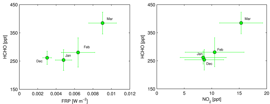
Figure 13. Multi-year averaged (2004–2009) monthly means of X_{\text{HCHO}} as a function of spatially averaged FRP over selected regions (see Table 3) (left) and multi-year averaged (2004–2009) monthly means of X_{\text{HCHO}} as a function of X_{\text{NO}_2} (right) at Pico Espejo. The standard deviation of monthly means is given (see Table 3).
