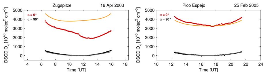
Figure 5. Diurnal evolution of \text{O}_4 DSCDs for \alpha = 0^\circ and \alpha = 90^\circ for single days with clear sky conditions at Zugspitze (left) and Pico Espejo (right). Here, \text{O}_4 DSCDs are retrieved from measured (red and black lines for \alpha = 0^\circ and \alpha = 90^\circ , respectively) and synthetic (orange and gray lines for \alpha = 0^\circ and \alpha = 90^\circ , respectively) spectra in the 346–372 nm fitting window and only shown for SZAs < 70^\circ (see Sect. 3).
