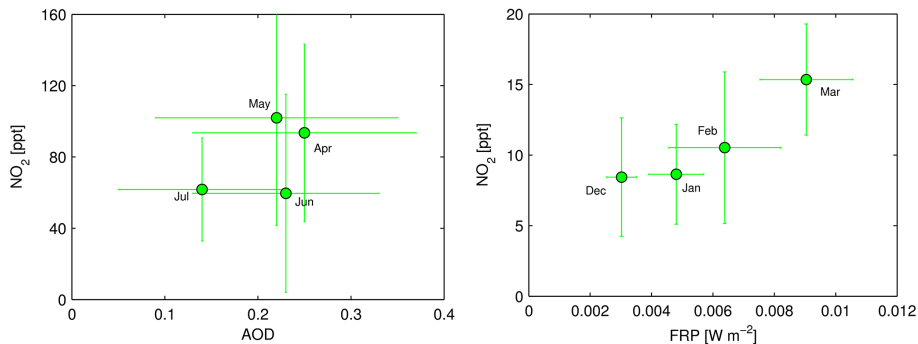
Figure 9. Monthly averaged X_{\text{NO}_2} at Zugspitze as a function of AOD and multi-year averaged (2004–2009) monthly means of X_{\text{NO}_2} at Pico Espejo as a function of spatially averaged fire radiative power (FRP) over selected regions (see Table 3). The standard deviation of daily and monthly means is given for Zugspitze and Pico Espejo, respectively (see Table 3).
