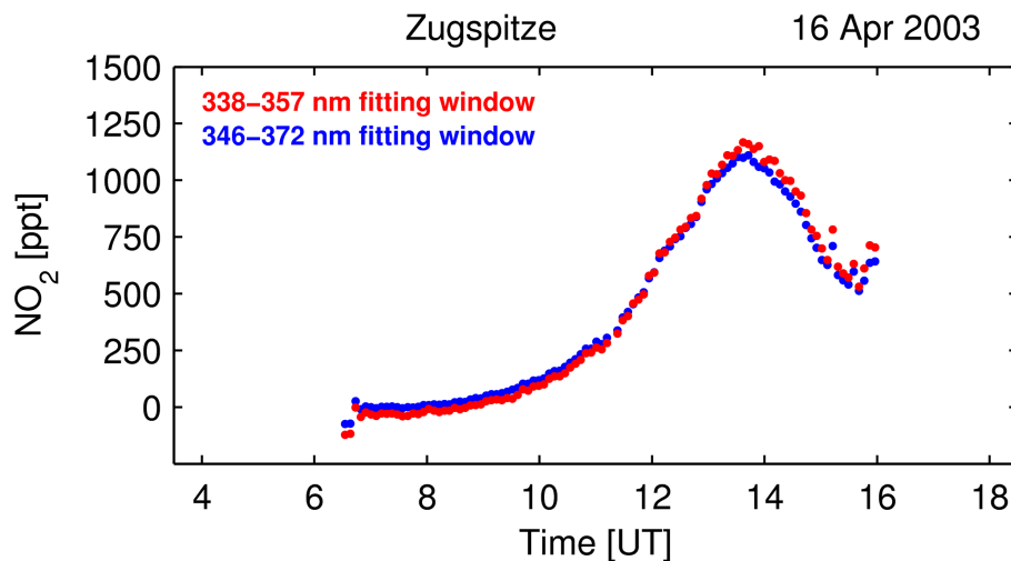
Figure 10. Diurnal evolution of X_{\text{NO}_2} (for \text{SZA} < 70^\circ , but without applying the other filter criteria as described in Sect. 6.2) on 16 April 2003 at Zugspitze as derived using the 338–357 nm (red) and 346–372 nm (blue) fitting windows.
