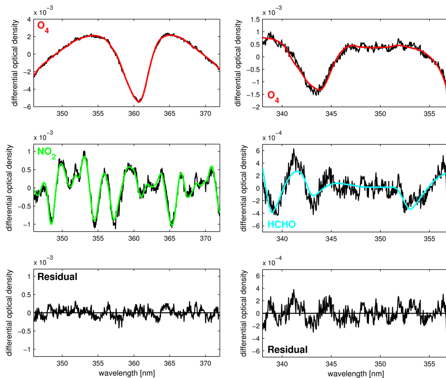
Figure 2. Exemplary fit results of the DOAS analysis in the 346–372 nm (left) and 338–357 nm (right) fitting window for a horizontal noontime MAX-DOAS spectrum ( \alpha = 0^\circ , SZA = 37.86^\circ ) as measured on 16 April 2003 at Zugspitze under elevated NO 2 (DSCD = 1.228 \times 10^{16} molec cm -2 ) and HCHO (DSCD = 1.737 \times 10^{16} molec cm -2 ) pollution. The red (upper panel), green and cyan (middle panel) lines show the O 4 , NO 2 and HCHO cross sections, respectively, as scaled to the O 4 , NO 2 and HCHO absorptions detected in the measured spectrum (black lines). The residuals with calculated root mean square (RMS) errors of 1.2 \times 10^{-4} (346–372 nm) and 1.3 \times 10^{-4} (338–357 nm) are also shown (lower panel).
