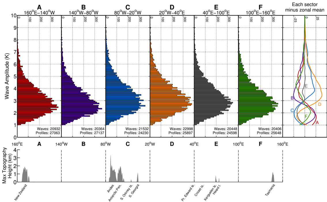
Figure 9. Histograms of individual wave amplitudes detected during June–August 2006–2012 in longitudinal sectors A–F in the latitude band 40\text{--}65^\circ\text{S} using the Wave-ID method (see text). The right-most panel shows the difference between the wave amplitude distribution in each sector and the zonal-mean distribution. The bottom panel shows maximum topography height in the latitude band 40\text{--}65^\circ\text{S}
