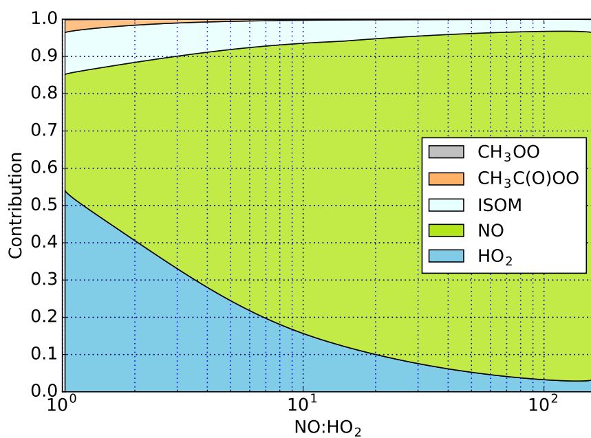
Figure 7. Relative contributions of different reaction pathways to the fate of ISOPOO radicals under different NO:HO 2 . ISOM indicates isomerization. Data are from the MXLCH complex scheme with F_{NO_x} = \pm 30 \text{ pptv ms}^{-1} and Yield_{ISOPN} = 6\% .
