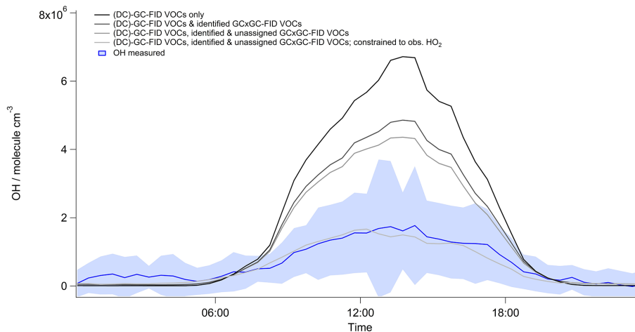
Figure 9. Average diurnal profile of modelled and measured [OH]. The shading represents the 1\sigma variability of the measurements; with each data point representing 30 min averaged data. See text for details of the different model scenarios.
