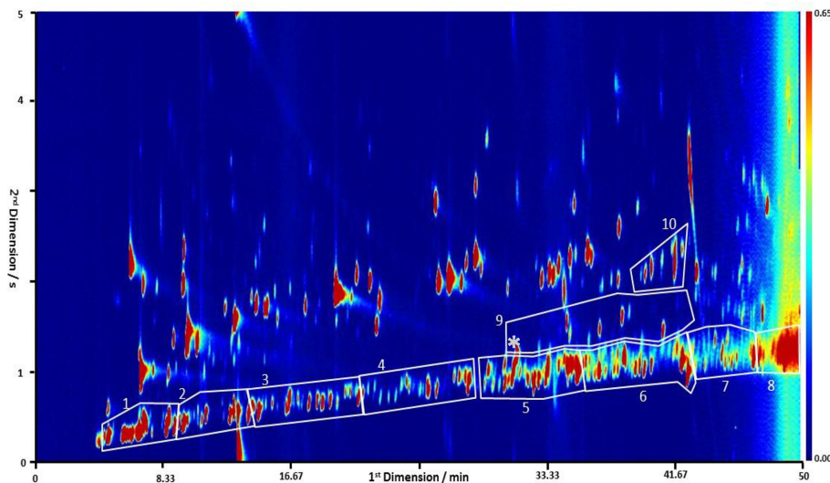
Figure 4. A typical GCxGC chromatogram from the summer ClearfLo campaign. The retention times from column 1 (separation based on volatility) and column 2 (separation based on polarity) are the x and y axis respectively, and compound intensity is the coloured contour. Labelled groups are identified as follows; (1–8) aliphatic groups from C_6 to C_{13} , (9) C_{10} monoterpenes with * corresponding to \alpha pinene which is the start of that group and (10) C_4 substituted monoaromatics.
