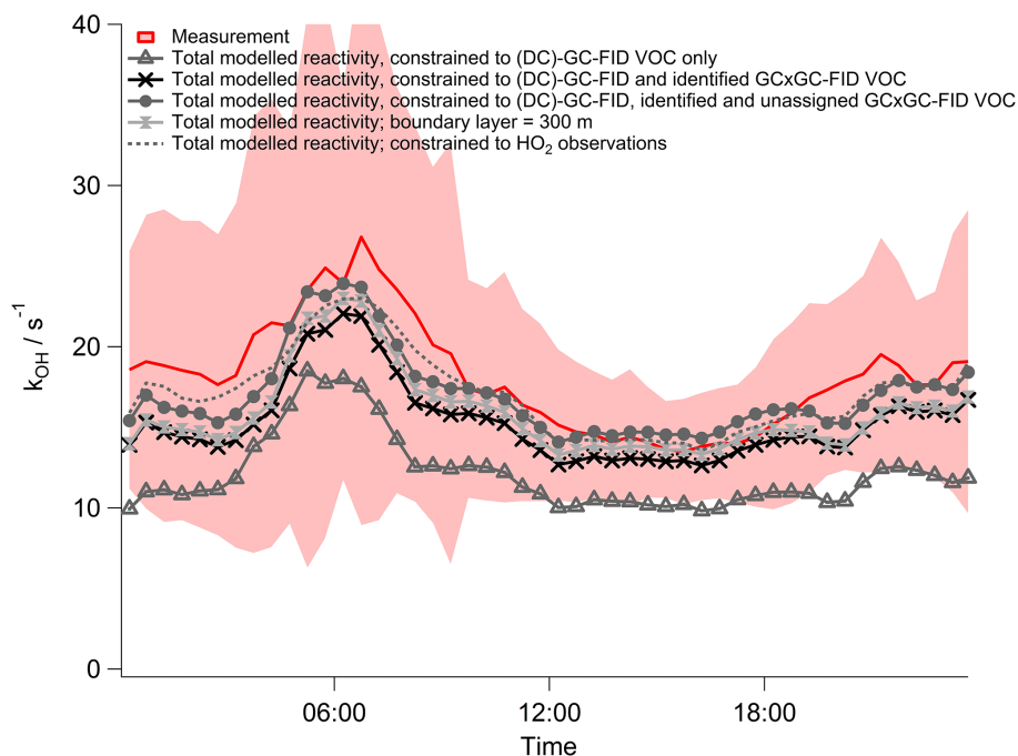
Figure 8. Average diurnal profile of the total modelled and measured OH reactivity for different model scenarios (see text for further details). The shading represents the 1\sigma variability of the measurements, with each data point representing 30 min averaged data.
