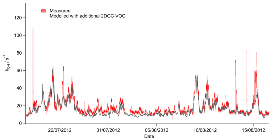
Figure 1. Measured and modelled OH reactivity time-series during ClearfLo with the periods of more polluted Easterly flows highlighted. The averaging period is 15 min. The 1\sigma uncertainty of the OH reactivity measurements (red shading) was, on average, \pm 3.2\text{ s}^{-1} . The model represents the OH reactivity calculated from the VOCs measured by the (DC)-GC-FID and GCxGC-FID instruments (see Table 1 for details), and the additional VOCs derived from unassigned peaks from the GCxGC-FID chromatographs as explained in the text, plus all model intermediates deriving from these species.
