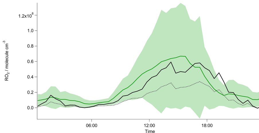
Figure 10. Average diurnal profile of measured RO_2 (green) and steady state calculated RO_2 using Eq. (3) (black, solid line = [RO_2]_{ss} derived from the observed total OH reactivity and grey, dashed line = [RO_2]_{ss} derived from calculated OH reactivity using (DC)-GC-FID VOC only). The shading represents the 1\sigma variability of the measurements; with each data point representing 30 min averaged data.
