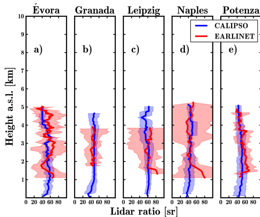
Page 31239 – Figure 5: Lidar ratio at 532 nm for CL3* (blue line) and EARLINET (red line). From left to right: (a) Evora, (b) Granada, (c) Leipzig, (d) Naples, and (e) Potenza.
