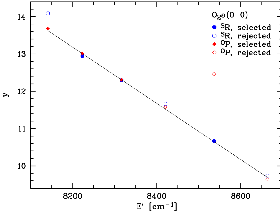
Figure 6. Derivation of O_2a(0-0) T_{\text{rot}} . The plot is similar to Fig. 4. Resulting from ^sR (circles) and ^oP (diamonds) line intensities, the mean populations of the odd rotational levels with N' from 13 to 23 for the full X-shooter sample are shown. Filled symbols mark reliable data points that were used for the derivation of T_{\text{rot}} (see Fig. 5), which is illustrated by the solid regression line.
