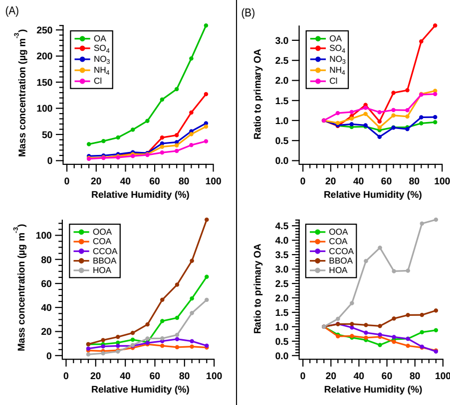
Figure 8. (a) Average mass concentration of the organic and inorganic species (top) and of the different OA sources (bottom) as a function of RH. (b) Average mass concentration of the OA and inorganic species (top) and of the OA sources (bottom) normalized to the sum of all primary sources (HOA, BBOA, CCOA and COA) and represented as a function of RH. For better representation of the trends, all components were further normalized to their corresponding value in the first RH bin. Note: RH bins of 10 % in all cases.
