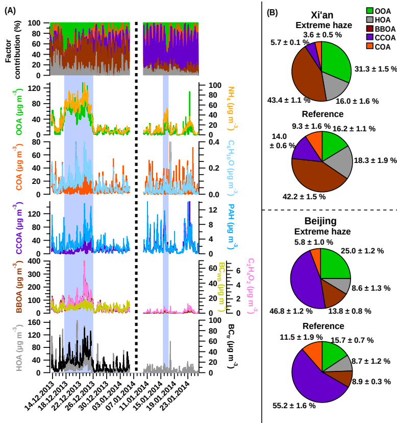
Figure 6. (a) Time series of the OA sources and the external tracers and relative contribution of the different sources over time; (b) Mean relative contributions of the OA sources for the four periods of interest. Errors represent the standard deviation among all good a value combinations.
