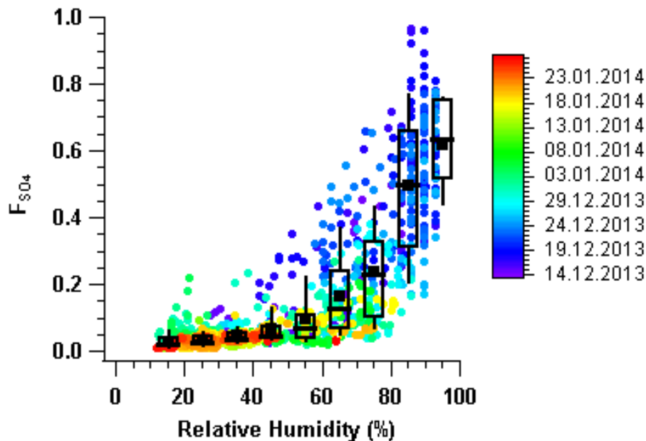
Figure 9. Sulfur oxidation ratio ( F_{\text{SO}_4} ) as a function of RH, color coded by date. Mean (square), median (middle horizontal line), 25th and 75th percentiles (P25-P75, box) and 10th and 90th percentiles (P10-P90, whiskers) are reported for each RH bin (10 % step).
