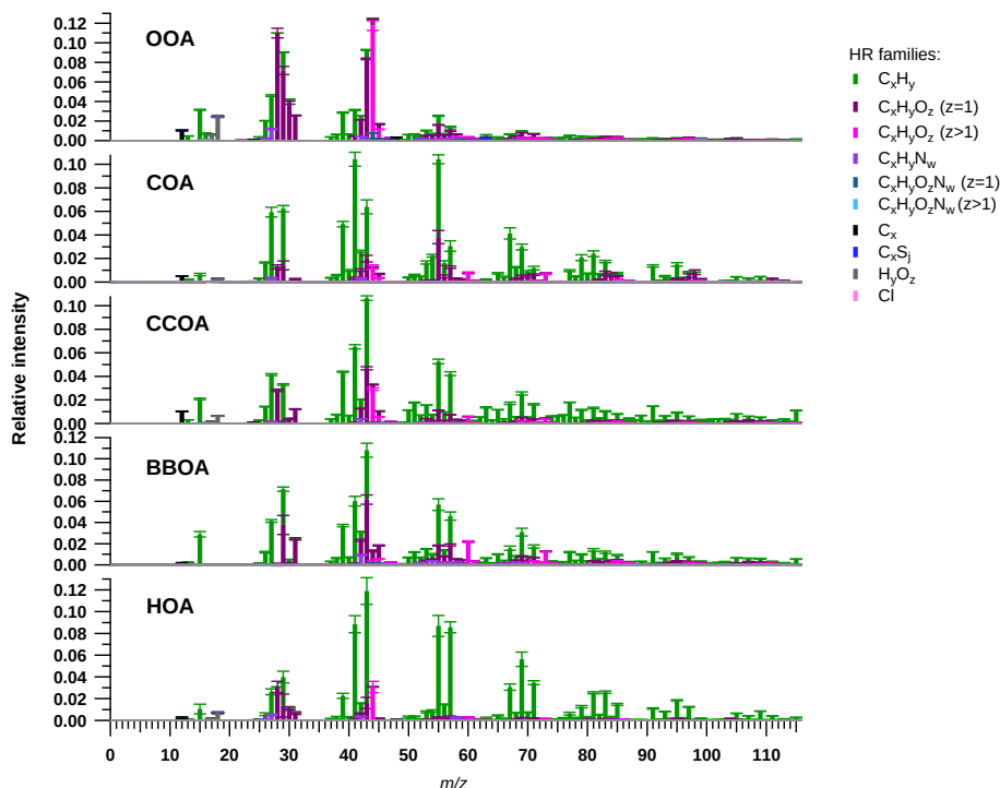
Figure 3. Mass spectra of the five identified OA factors color coded with the chemical families; Spectra are averaged over all good a value combinations and error bars represent the standard deviation of each m/z over all the accepted solutions.
