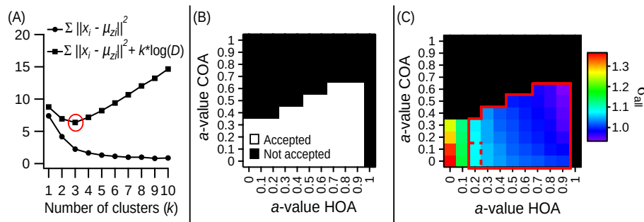
Figure 2. (a) The first term T1 (circles) and the total cost function CF ( T1+T2 ) (squares) defined in Eq. (4) for increasing number of clusters ( k ); (b) Final accepted a value range after applying the criteria 1 and 2; (c) Color coded quadratic sum of standard deviations between external tracers and correlated primary OA sources. The region surrounded with red line includes all final accepted a value combinations obtained from the study of the variability of the solution among 50 solutions with pseudo-randomly modified input matrix within twice its errors ( OA \pm 2OA_{error} ). Dashed line in left lower corner shows the two a value combinations that would not have been considered as good solutions if smaller changes are allowed to the input matrix ( OA(i, j) \pm 1OA_{error}(i, j) ) and only 10 solutions are considered for the variability study.
