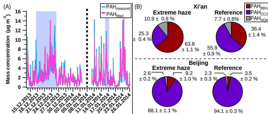
Figure 10. (a) Time series of the measured (blue) and fitted PAH (pink); (b) Relative contributions of the different sources to PAH for the four periods of interest. Errors represent the standard deviation among all good a value combinations.
