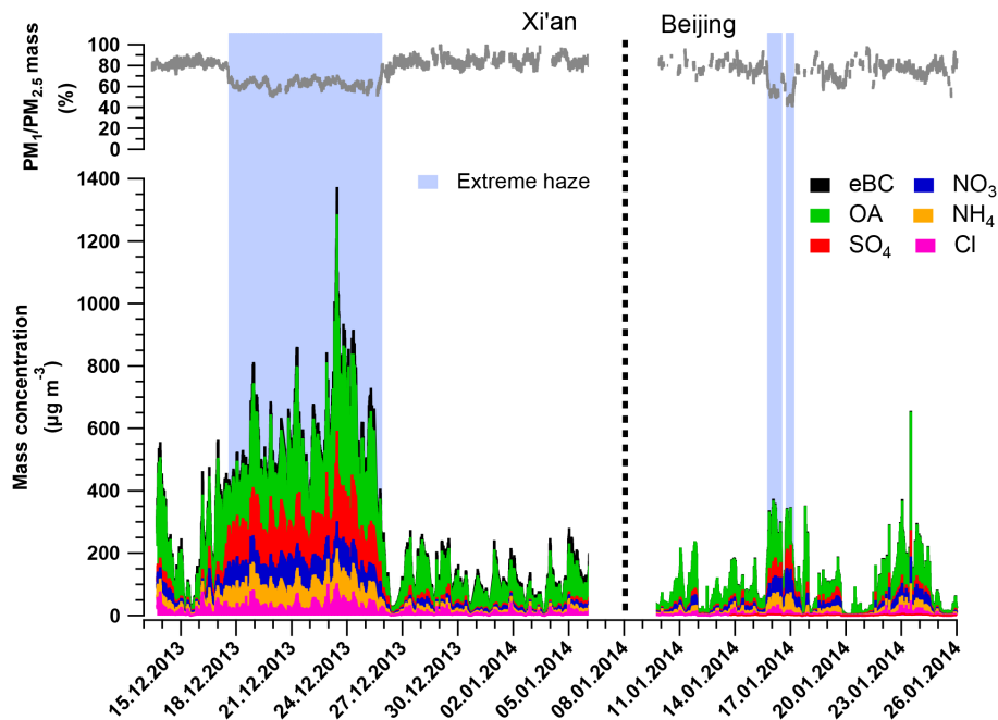
Figure 4. Bottom: time series of the AMS species and eBC mass concentrations for the full measurement period; Top: ratio between the NR mass that would have been measured using a PM 1 lens and the total mass measured with the PM 2.5 lens.
