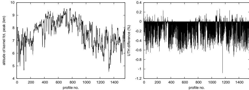
Figure 3: Left panel: peak emission altitude (km) at Lindenberg for 1560 radiosonde profiles from February 2000 to April 2001. Right panel: UTH differences for changes in the peak emission altitude and water vapour scale height. Peak emission altitude is assumed to rise by 50 m, scale height by 10 m.
