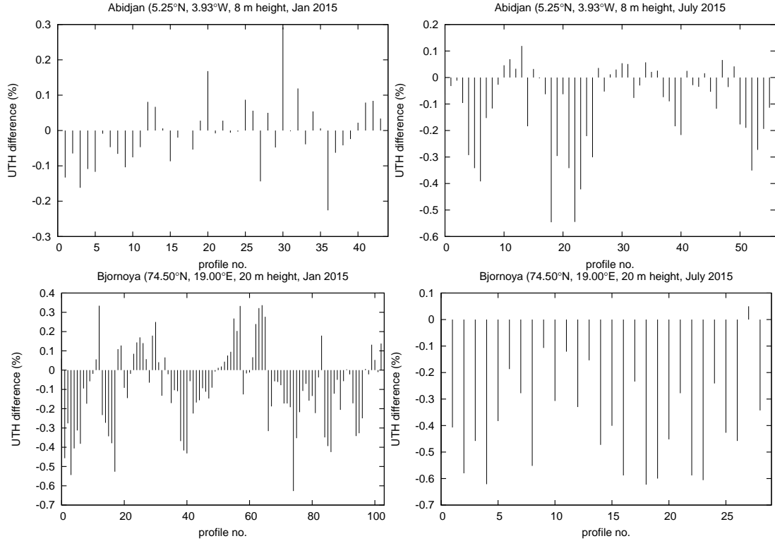
Figure 1: UTH differences for changes in the peak emission altitude and water vapour scale height for tropical station Abidjan and polar station Bjørnøya. Peak emission altitude is assumed to rise by 50 m, scale height by 10 m.
