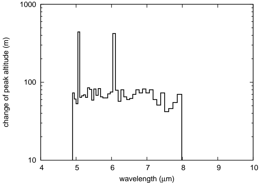
Figure 2: Change in peak emission altitude (m) as a function of wavelength resulting from a run of the SBDART radiative transfer code run in the wavelength range 4.5 to 9.9 \mu\text{m} with a resolution of 20 \text{ cm}^{-1} .
