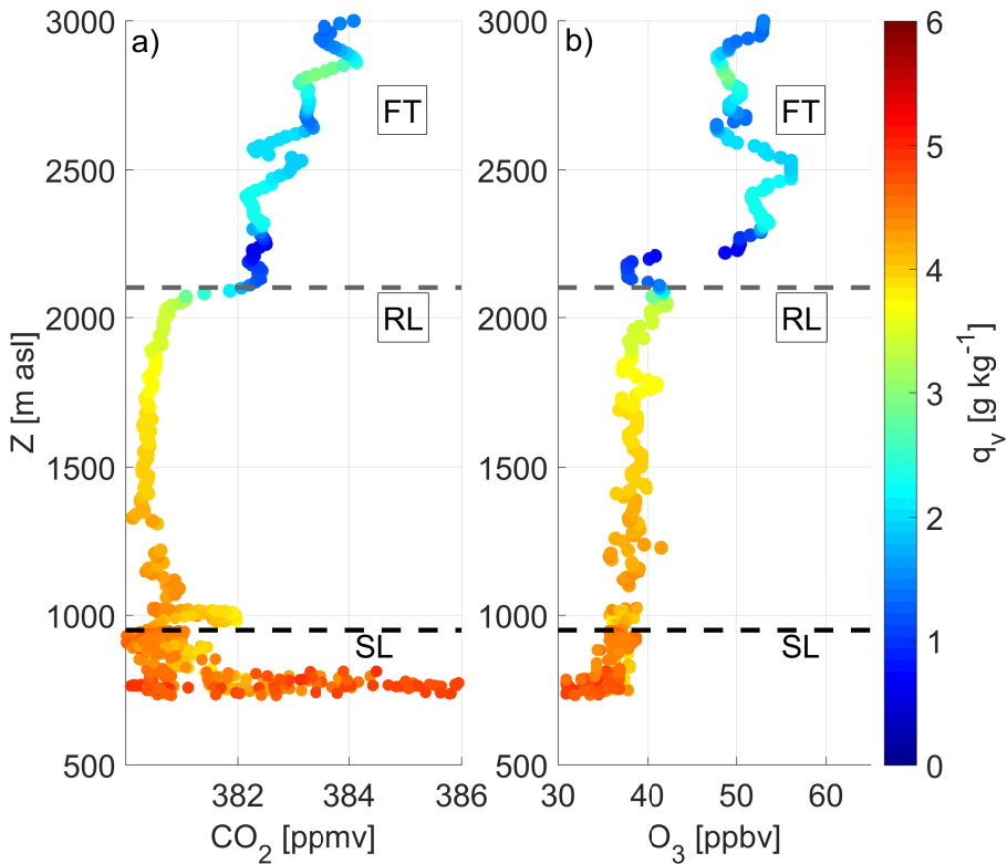
Figure 7. Vertical profiles of a) CO 2 and of b) O 3 in the morning (07:27 UTC) on 6 September 2011. The color shows the specific humidity, and the horizontal lines show the boundary layer height (black dashed line) and the residual layer height (dashed gray line).
