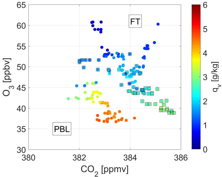
Figure 10. Same as Fig. 9 at noon. The measurement points between 1640 and 2200 m a.s.l. (black boxes) are related due to the mixed air masses from the stable Layer and the FT.
