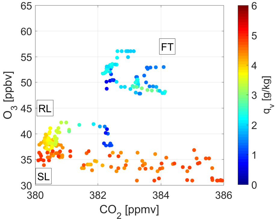
Figure 9. Correlations between CO 2 and O 3 during the observations at 07:27 UTC color-coded according to specific humidity measurements. The aircraft descended from the FT into the PBL, indicated by a clear separation from the chemical signature.
