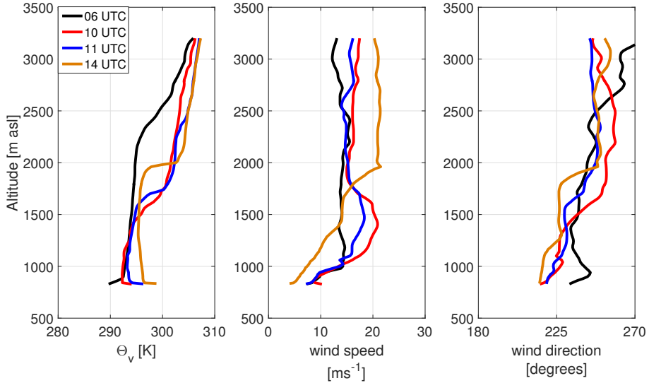
Figure 6. Profiles of a) virtual potential temperature, b) wind speed, and c) wind direction derived from radiosondes during the day (black : 6 UTC, red: 10 UTC, blue: 11 UTC, orange: 14 UTC) on 6 September 2011.
