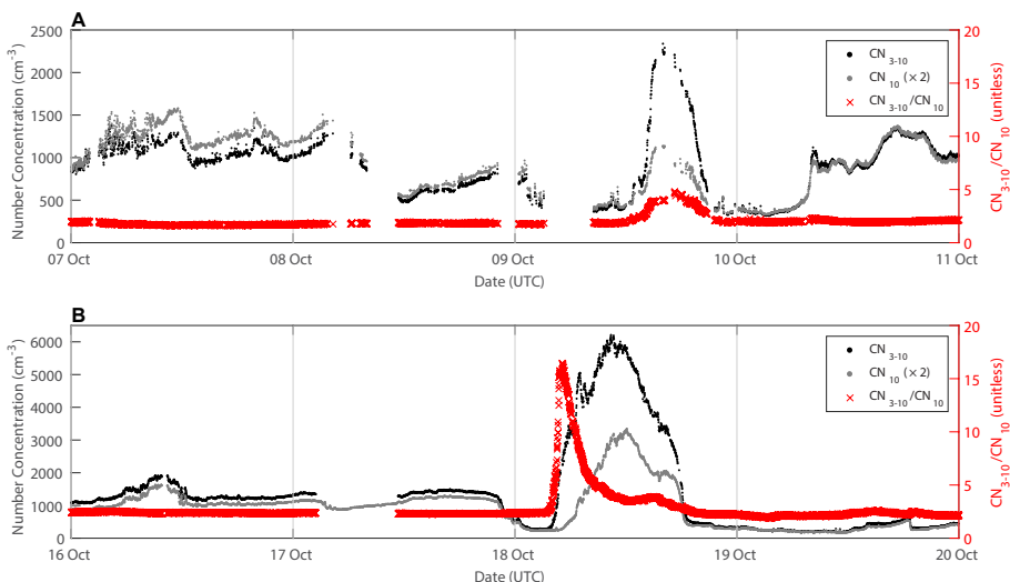
Figure 2. Four days of aerosol number concentrations in the two available size bins, 3–10 nm ( \text{CN}_{3-10} ), and those larger than 10 nm ( \text{CN}_{10} ), along with their ratio that helps to identify new particle formation and growth. (a): four days representative of the dataset show simultaneous variation in both size bins, and little variation in ratio data. (b): similar to (a) , except it includes the only growth event that was observed during the voyage, included to demonstrate what growth would look like with the available data, showing a delay in variations between the two size bins. Note the change in scale of the left y axis between the two plots.
