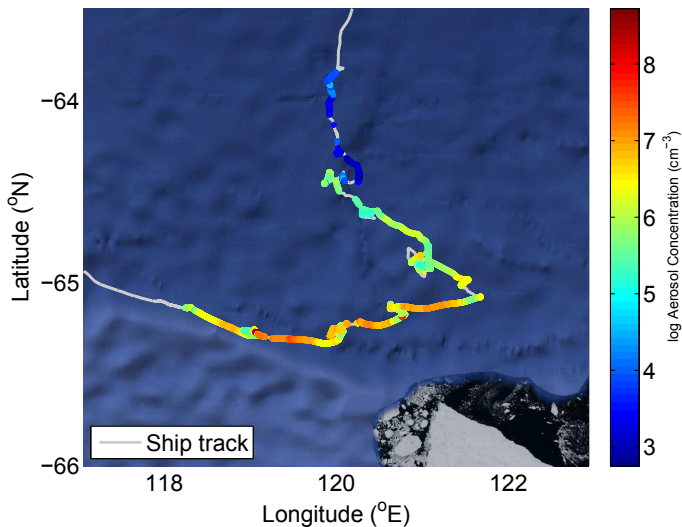
Figure A3. CN_{3-10} number concentrations in log scale, overlaid on the ship's track (grey line) and Google Earth satellite imagery. The step change is observed clearly around 64.4°S, while a gradual increase can be discerned with increasing latitude within the Polar Cell.
