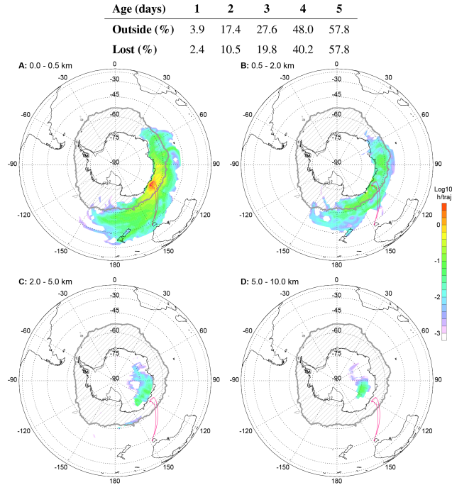
Figure 7. Five day forward trajectories released from SIPEXII locations and times and passing through the following atmospheric layers: (a) the first 500 m, (b) 500 m to 2 km, (c) 2 to 5 km and (d) 5 to 10 km. The ice edge and ship track are shown for reference, while colours reflect the percentage, in log scale, of trajectories released which pass through a given grid box. The table above classifies, as a function of days after release, the percentage of the total number of trajectories either outside – those outside the sea-ice edge on the given day; or lost – those which do not re-enter the sea-ice zone after the given number of days.
