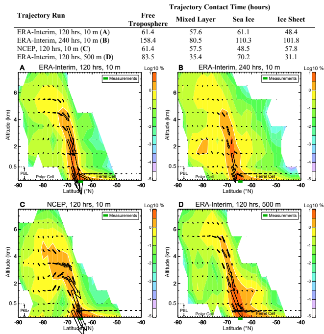
Figure A4. Assessment of reliability of trajectory analyses in the Antarctic region. (a): longitudinally averaged cross section showing grid frequency of five day back-trajectories using ERA-Interim reanalysis, released at 10 m a.s.l. for every hour of the voyage, with two-dimensional vectors weighted by the number of points at each location. (b): as in (a) , but for ten day trajectories. (c): as in (a) , but using NCEP reanalysis. Analyses with GDAS reanalysis produced patterns similar to ERA-Interim. (d): as in (a) , but using a starting point of 500 m. Varying any of these parameters creates minimal changes in final trajectories, giving confidence in the conclusions of circulation. The table above outlines average contact time with various aspects of the atmosphere and surface. Note the sum of the free-troposphere and mixed layer contact times does not equal the total time due to necessary data removal and rounding.
