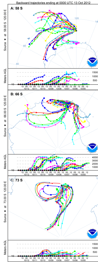
Figure 4. Three day (72 h) back trajectories calculated from 10 m above mean sea level using the HYSPLIT model with GDAS input meteorology for a seven day period ending at midnight on 13 October 2012. All trajectories have endpoints at 120^{\circ} E, and differing latitudes: (a) ( 58.0^{\circ} S), (b) ( 66^{\circ} S) and (c) ( 73.0^{\circ} S). Changes in colour help identify different trajectory ending times.
