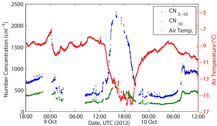
Figure A8. Air temperature and aerosol number concentrations in the two size ranges during the enhanced aerosol event of the 9 October.
