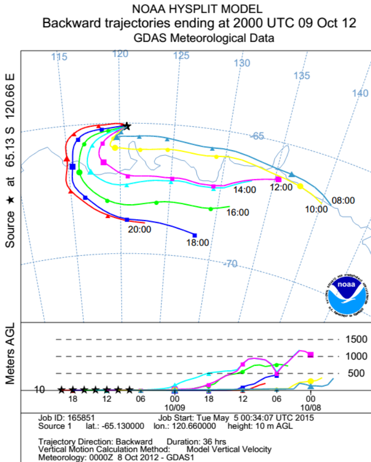
Figure A7. 36 h backward trajectories released every two hours from the measurement location (10 m a.s.l.) and spanning the 9 October enhanced aerosol event.
