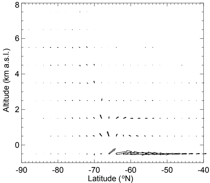
Figure A5. Two-dimensional vectors weighted by number of points at each pixel. Trajectories were calculated from the ten day forward trajectories beginning at the ship location throughout the voyage. The rising air of the polar front is clearly visible, however the overwhelming flow is found to ascend slightly within the boundary layer, above the layer closest to the surface, then travel north.
