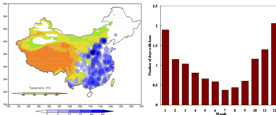
Figure 2. Distribution of annual haze event frequency (days per year) averaged over 1961–2012 in China, and Chinese topography of the TP and the Loess Plateau with altitudes is shown with yellow shades (left panel). Monthly variation of haze frequency averaged from 1961–2012 over the CEC region (right panel).
