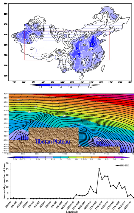
Figure 3. Surface wind speed distribution ( \text{ms}^{-1} ) averaged over 1961–2012 in China with the red rectangle marking the region for cross sections in the middle and lower panels (upper panel). Cross sections of horizontal wind speed ( \text{ms}^{-1} ; filled color contours) and vertical circulations illustrated by stream lines (middle panel) and zonal variations of annual haze event frequency (lower panel) at 27\text{--}41^\circ\text{N} averaged over 1961–2012. Note that near-surface vertical and horizontal winds are not illustrated well here due to north–south variations in the terrain and approximation of the location of the TP in this figure. All fields are for the annual-averages.
