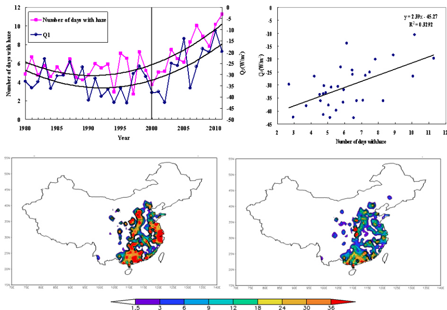
Figure 4. Interannual variability in the apparent heat source Q_1 (the negative values denote cooling) integrated vertically over the TP and haze event frequency averaged in the CEC in winter (December, January and February) over 1980–2012 and their correlation (upper panel). The differences of haze frequencies (days) averaged in five winters with most positive (lower left panel) and most negative Q_1 anomalies (lower right panel) on the TP relative to the mean haze frequency from 1980 to 2012.
