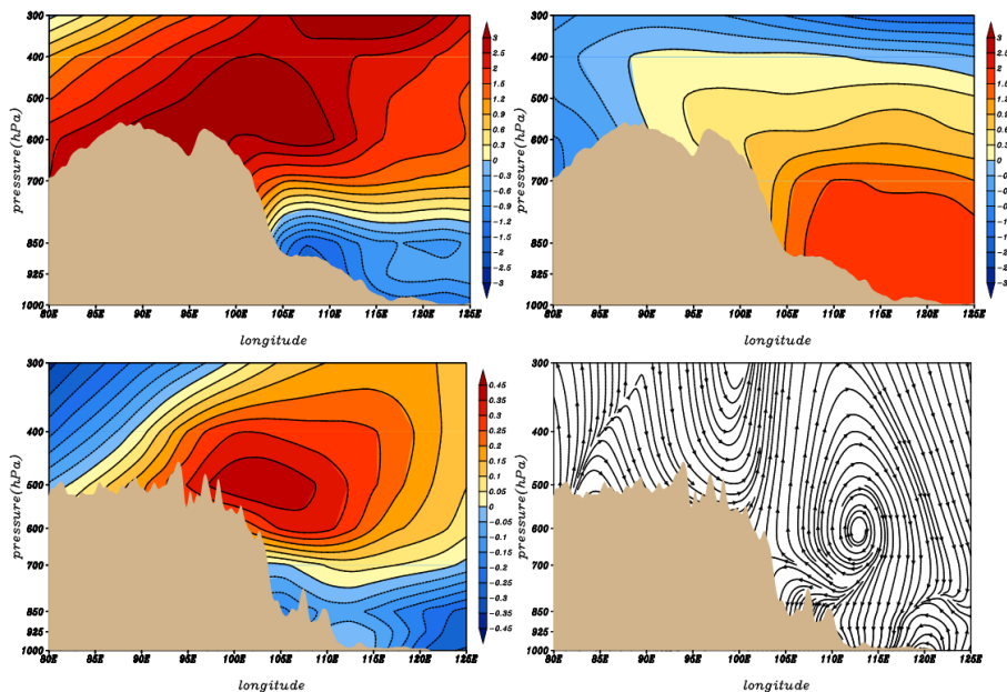
Figure 6. Vertical sections of the anomalous air temperature ( ^{\circ}\text{C} ) averaged along 27\text{--}41^{\circ}\text{N} in five winters with most positive (upper left panel) and most negative Q_1 anomalies (upper right panel) on the TP from 1980 to 2012, and vertical sections of the correlations of the number of haze days with air temperature (lower left panel) and vertical circulations (lower right panel) in winter from 1980 to 2012.
