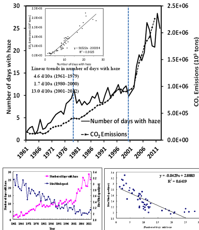
Figure 1. Interannual variations in the total CO 2 emissions in mainland China and the haze event frequency averaged in the CEC region over 1961–2012 with their relationship in the inserted figure (upper panel). The Chinese CO 2 emission data source: http://cdiac.ornl.gov/CO2_Emission/timeseries/national ; two blue dotted lines separate the time series into three phases of the 1960s–1970s, the 1980s–1990s and the 21st century. Interannual variations in wind at 10 m (blue line) and the number of days with haze (red line) in the CEC over 1961–2012 (lower-left panel) and their scatter plot (lower-right panel).
