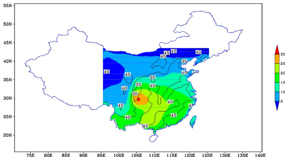
Figure 7. The percentages (%; contour lines) of differences of surface aerosol concentrations between winters of 1998 and 2003 with positive and winters of 1996 and 2002 with negative Q_1 anomalies on the TP relative to the surface aerosol levels averaged over winters of 1996, 1998, 2002 and 2003 ( \mu\text{g m}^{-3} ; color contours) modeled by the sensitivity simulation experiment with GEM-AQ/EC.
