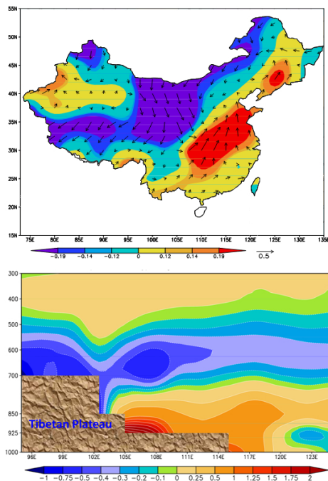
Figure 5. The distributions of the interannual correlations of the apparent heat source Q_1 over the TP to the local V component of surface wind in winter over 1961–2012 (color shading). Arrows denote correlation vectors (showing both correlation coefficients of Q_1 to U and V surface wind components) in China. The correlation coefficients of 0.12 (–0.12), 0.14 (–0.14) and 0.19 (–0.19) respectively passing the significance levels of 90, 95 and 99%. A vertical section of the trends in vapour content (g kg -1 per 10 years) in winter over 1961–2012 averaged along 27–41° N (lower panel).
