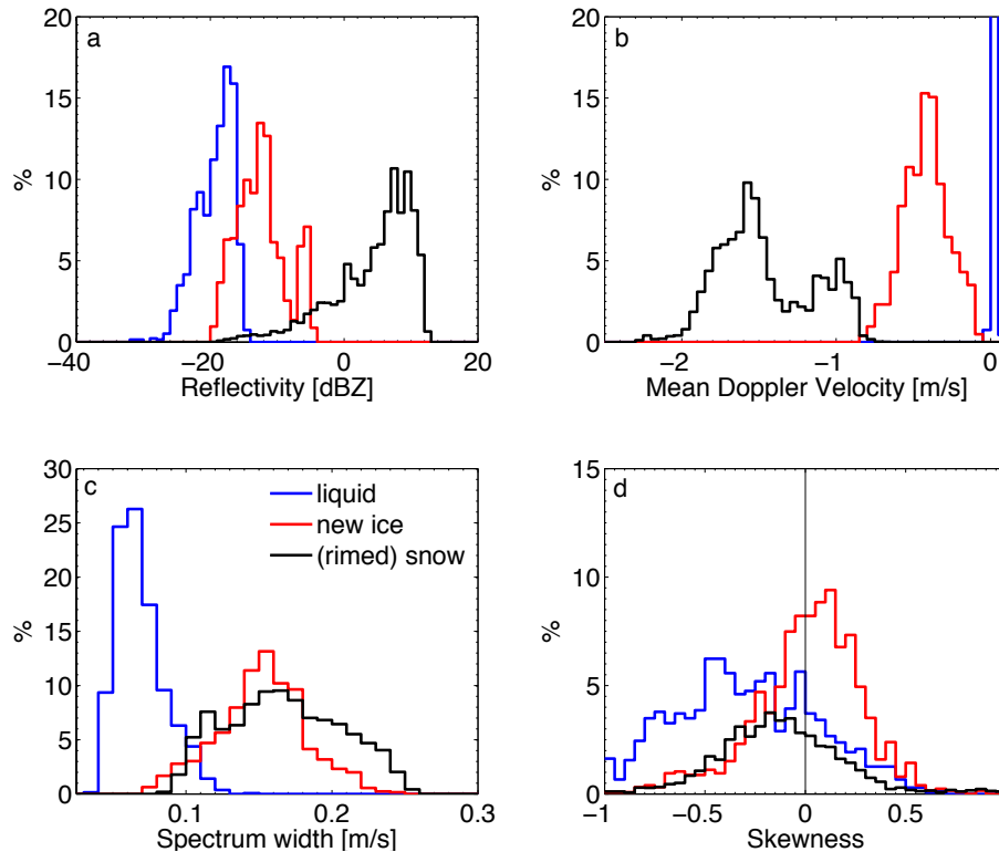
Figure 7. Probability density functions (PDF) of noise-separated peaks of SLW (blue), ice generated in the SLW layer (red), and frontal snow (black) for the slanted paths encompassed by the two dashed lines in Fig. 4. Only data from surface to below top of the SLW layer (3.4 km) is considered. Please note that the PDF of SLW V_d is cut at 20 %.
