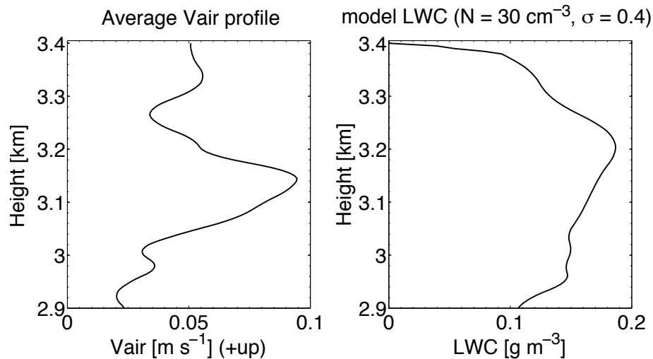
Figure 9. Mean vertical air motion profile (Vair, left) derived from liquid mode mean Doppler velocity and liquid water content (LWC, right) derived from liquid peak reflectivity between the two black fall streaks in Fig. 4, respectively.
