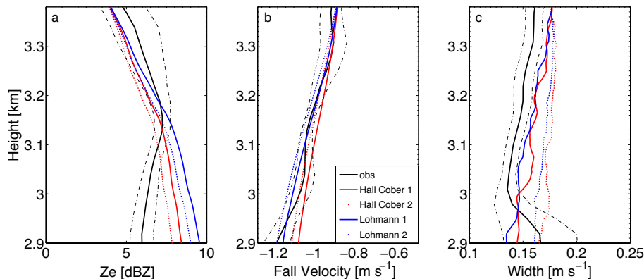
Figure 10. Comparison of observed and modeled moments of the frontal snow mode in the SLW layer. Black solid and dashed lines refer to the mean and standard deviation of the slanted paths encompassed by the two black fall streaks in Fig. 4. Model results based on riming efficiencies by Hall & Cober as well as Lohmann are shown in red and blue, respectively (for details see text). Model results assuming area ratio increase with mass and rimed fraction (solid red and blue line) as well as with mass only (dotted red and blue) are shown.
