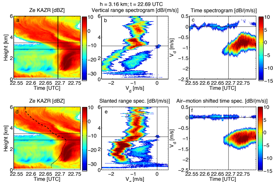
Figure 5. Panels (a) and (d) show KAZR reflectivity ( Z_e ) field. There, the location of the SLW layer is indicated by thin horizontal black lines. Upper middle and upper right panel show range- and time spectrogram of vertical profile which is indicated by black vertical line in (a), lower middle and lower right panel along slanted fall streak shown in (d) as dashed line. (b) Vertical range spectrogram along vertical black line in upper left panel, (c) time spectrogram at 3.16 km, (e) slanted range spectrogram along dashed line in (d). (f) Air-motion corrected time spectrogram at 3.16 km.
