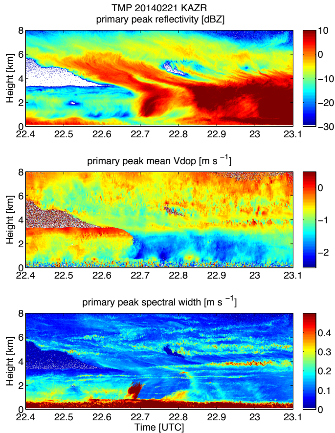
Figure 2. KAZR observed primary Doppler spectrum peak moments on 21 February 2014 in Hyttiälä. Panel (a) shows reflectivity (dBZ), (b) mean Doppler velocity ( \text{m s}^{-1} ), and (c) spectrum width of the primary Doppler spectrum peak ( \text{m s}^{-1} ). Negative Doppler velocities indicate downward motion.
