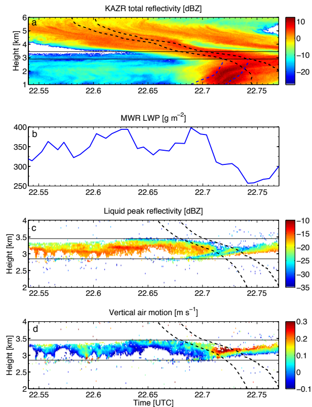
Figure 4. Zoomed view (2–4 km, 22.54–22.77 UTC) of the snow front on 21 February 2014. Panel (a) shows KAZR total reflectivity, (b) microwave radiometer (MWR) liquid water path (LWP), (c) reflectivity of the liquid peak, (d) mean Doppler velocity of the liquid peak used as vertical air motion tracer. The dotted lines depict individual fall streaks starting at different generating levels z_{\text{gen}} ( z_{\text{gen}} = 6 km (black), z_{\text{gen}} = 2.9 km (blue)). All subsequent averaged profiles refer to the area between the two black fall streaks.
