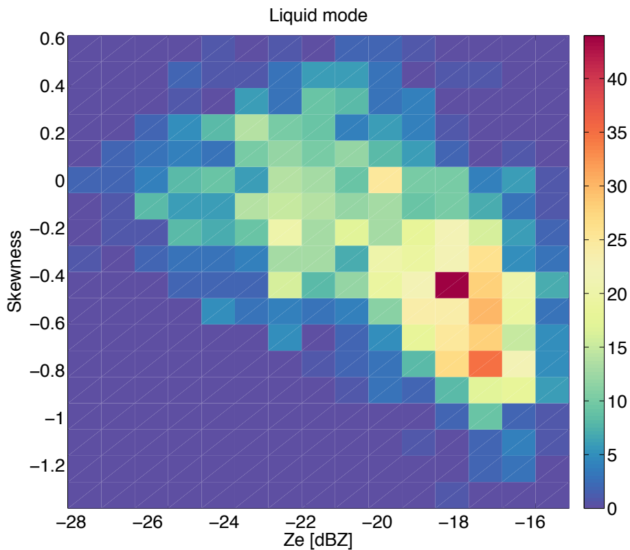
Figure 8. Joint PDF of frequency of occurrence of skewness and reflectivity of supercooled liquid mode encompassed by the two black fall streaks in Fig. 4.
