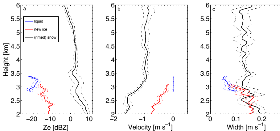
Figure 6. Slanted profile moments of SLW (blue), ice generated in the SLW layer (red), and frontal snow (black). Means and standard deviations of (a) reflectivity, (b) mean Doppler velocity, and (c) mode width are shown for the slanted paths encompassed by the two dashed lines in Fig. 4. Within the SLW water layer, velocities are corrected for vertical air motion.
