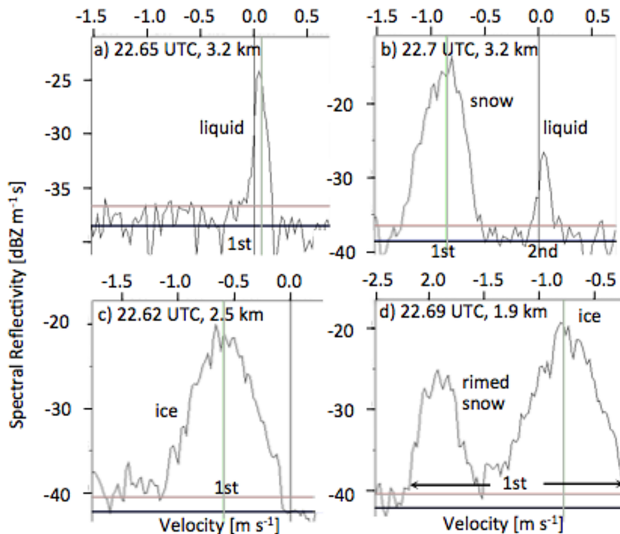
Figure 3. Examples of KAZR Doppler spectra at different times and heights. Notice the different x and y scales. Maximum and mean noise floor determined according to Hildebrand and Sekhon (1974) are indicated by grey and black horizontal lines, respectively. Primary peak is labeled as 1st, secondary peak as 2nd. Mean Doppler velocity of primary peak is shown by vertical grey line. The plots are created with the Doppler Spectrum Visualizer, a visualization toolkit which is publicly available at http://www.gim.bnl.gov/armclouds/specvis_java_toolkit/ .
