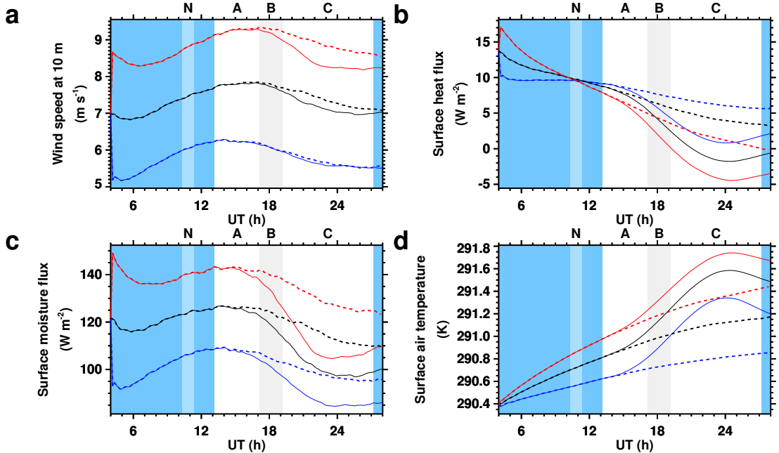
Figure 5. Wind speed and the diurnal cycle. Time series from simulations M^- (blue), M^0 (black), M^+ (red), solid curves, and from simulations M^-_{\text{dark}} (blue), M^0_{\text{dark}} (black), M^+_{\text{dark}} (red), dashed curves. Blue shading indicates nighttime. The time periods A, B, C, and N are highlighted to facilitate the discussion.
