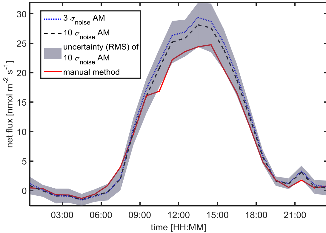
2 Figure 5: Diurnal averagenet flux of the automated method (AM) with 3 and 10 \sigma_{\text{noise}} threshold for 3 the flux calculation and the manual method. , the automated method with compound filter (AMCF) 4 using a 10 \sigma_{\text{noise}} threshold. The uncertainty (root mean square) was calculated for the automated 5 method with 10 \sigma_{\text{noise}} . its uncertainty (root mean square) and the classical method. The time is in CET 6 wintertime.
