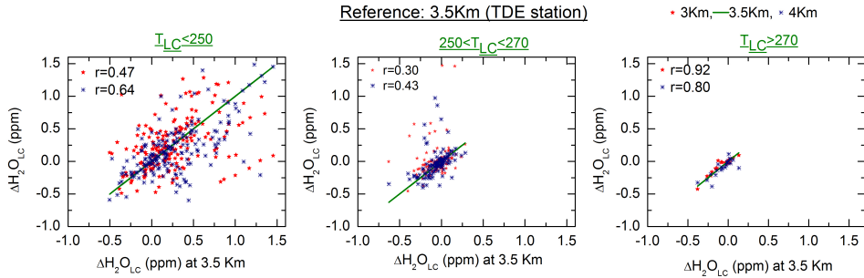
Figure A6. A 3-year (2012-2014) analysis of the uncertainty in the vertical resolution of the model using TDE as reference station. The correlation between \Delta H_2O = \log[H_2O'_{t=0}] - \log[H_2O_{LC}] at 3500 m with 3000 and 4000 m respectively, is shown.
