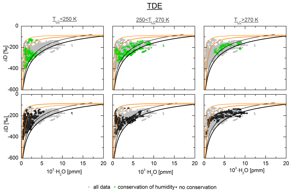
Figure 9. Same as Fig. 8 for the data collected at TDE station.
