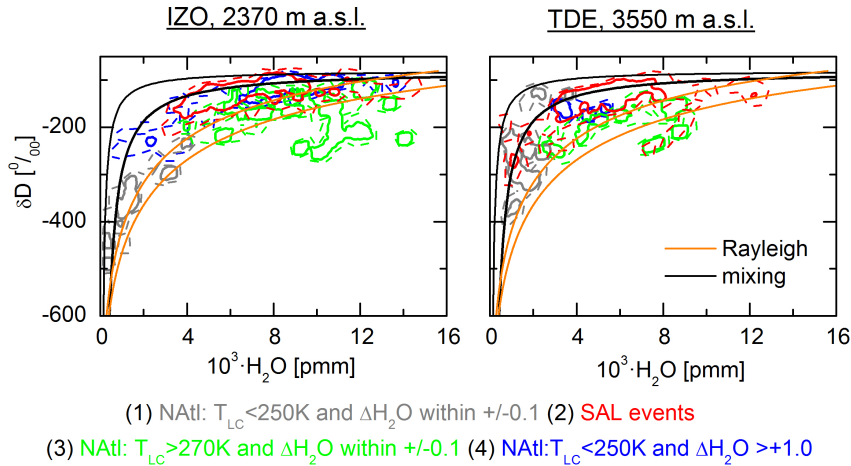
Figure 10. H_2O - \delta D distributions as obtained for the four different moisture pathways that determine the free troposphere moisture budget in the surroundings of Tenerife (Left panel for IZO and right panel for TDE). Depicted are contour lines indicating the areas of the highest data point density. The thin dashed and thick solid lines mark the areas that include 95 and 66 % of all data, respectively. The different colour of the contour lines mark the different pathways (1–4) as given in the legend. Rayleigh and mixing curves are plotted as in Figs. 5, 6, 8 and 9.
