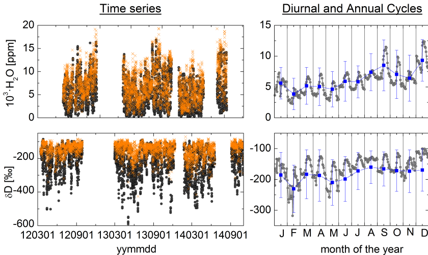
Figure 2. Left: time series of \pm 1 h averages of \text{H}_2\text{O} and \delta\text{D} measured at IZO station. Black dots represent the data collected from midnight to 1 h after sunrise (nighttime). Orange crosses represent the data collected during daylight (from 3 to 10 h after sunrise). Right: monthly mean of Grey dots show the mean diurnal cycle of \text{H}_2\text{O} and \delta\text{D} observed each month of the year. Blue dots show the annual cycle (mean and standard deviation) of the data set.
