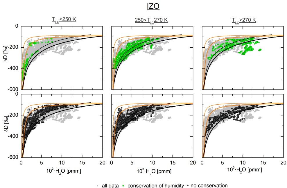
Figure 8. H_2O - \delta D distribution (10 min data within \pm 3 h of the arrival time of the airmass) measured at IZO station and analysed with regard to the LC point. The data set has been grouped in 3 groups corresponding to different condensation temperatures: T_{LC} < 250 \text{ K} , 250 \text{ K} < T_{LC} < 270 \text{ K} and T_{LC} > 270 \text{ K} . The H_2O - \delta D pairs measured for reduced mixing since LC ( \Delta H_2O \pm 0.1 ) are presented in green. Pairs measured for increased mixing since LC ( \Delta H_2O outside \pm 0.1 ) are presented in dark grey. Rayleigh and mixing curves are plotted as in Figs. 5 and 6.
