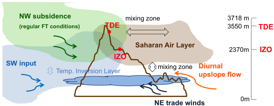
Figure 1. Schematic depiction of the processes influencing the water vapour balance over Tenerife Island in the subtropical North Atlantic. A temperature inversion layer (TIL) separates the Marine Boundary Layer (MBL) and the Free Troposphere (FT). In the MBL, NE trade winds blow, while in the FT, the regular NW subsidence regime is alternated in summer with Saharan dust outbreaks. At the island, the upslope winds prompt that MBL air reaches the low FT during daylight. IZO and TDE stations are represented as red dots.
