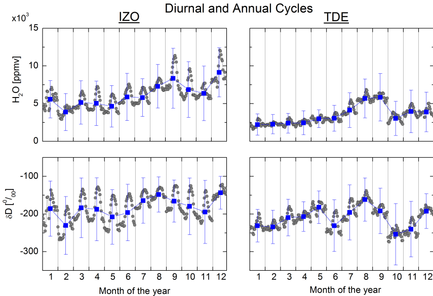
Figure 3. The mean diurnal cycle and annual cycles of \text{H}_2\text{O} - \delta\text{D} (left panels for IZO and right panels for TDE). Grey dots show the mean diurnal cycles for each month (mean value for each hour of the day) and the blue squares the annual cycle (mean and standard deviation of all observations that fall within an individual month).
