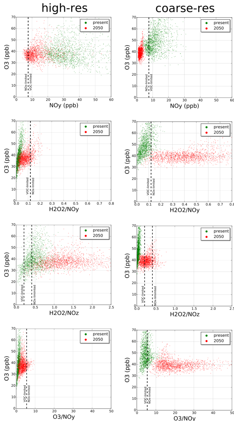
Figure 6. Scatter plots of MD8hr ozone concentrations (y-axis) against chemical regime indicators (x-axis) for the present and future runs in Paris. Results are presented for the high-resolution (left panels) and the coarse-resolution (right panels) applications. All chemical compounds are represented by their MD8hr values. Dots correspond to MD8hr concentrations for each day of the ozone period. For each indicator the limit value that separates the regimes is also depicted with a dashed line.
