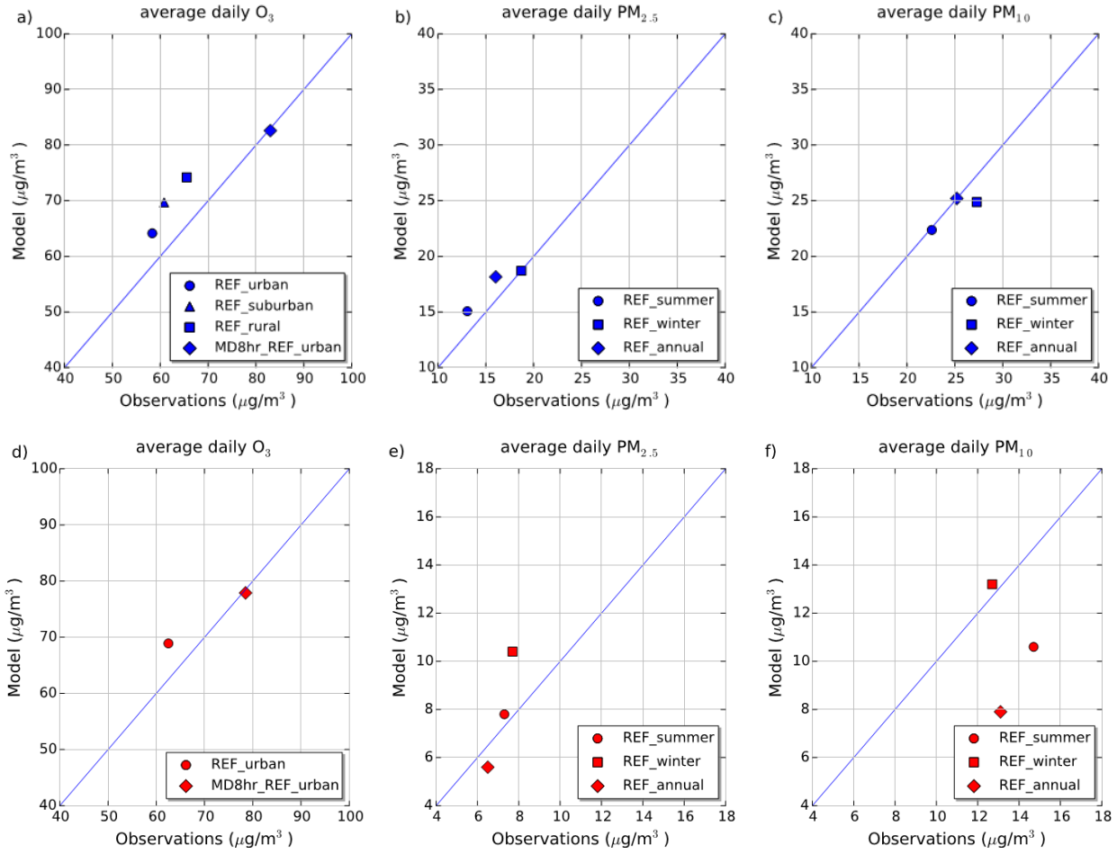
Figure 3. Ozone period (April-August) average ozone concentrations at urban, suburban and rural stations in IdF (panel a) and one urban station in the Stockholm area (panel d). The MD8hr values at urban locations are also shown (MD8hr_REF_urban). Average PM_{2.5} and PM_{10} concentrations in wintertime (DJF), summertime (JJA) and on annual basis over urban stations in IdF are shown in panels b,c (panels e,f for Stockholm).
