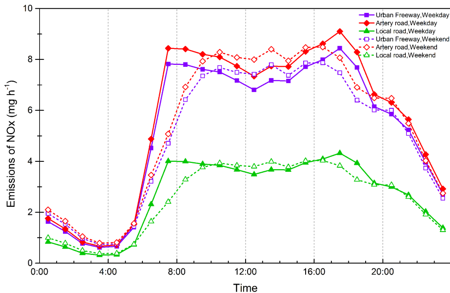
Figure 6. Hourly variation of vehicle emissions by road type on weekdays and weekends.
