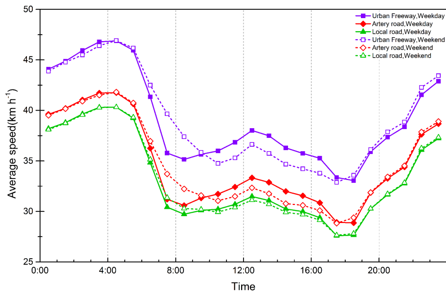
Figure 3. Hourly traffic average speed on different road types in Beijing.
