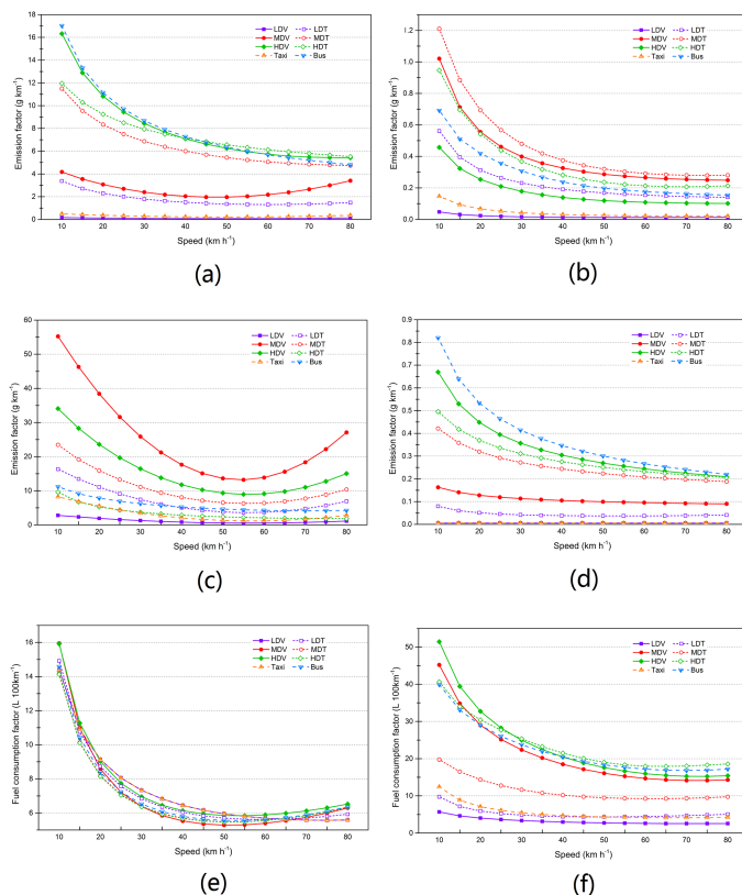
Figure 1. Emission factors of NO x , HC, CO, PM and fuel consumption factors of gasoline and diesel (Huo, 2009; Hu et al., 2012; Wu et al., 2012; Wang et al., 2013): (a) emission factors of NO x , (b) emission factors of HC, (c) emission factors of CO, (d) emission factors of PM, (e) fuel consumption of gasoline, (f) fuel consumption factors of diesel.
